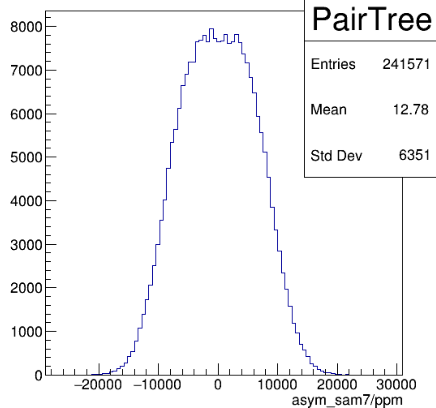
asym_sam7/ppm {ErrorFlag==0}
