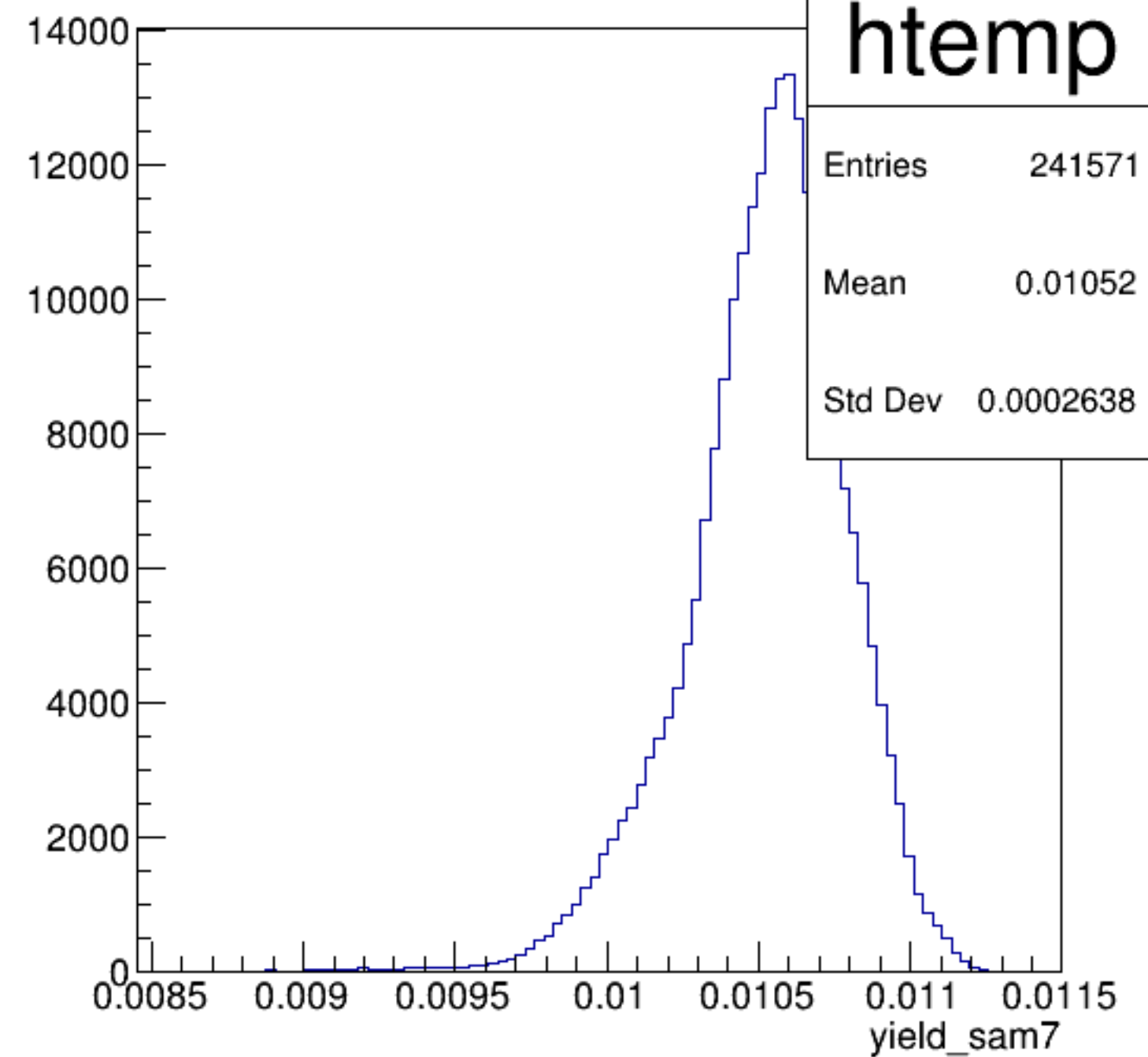
yield_sam7 {ErrorFlag==0}
