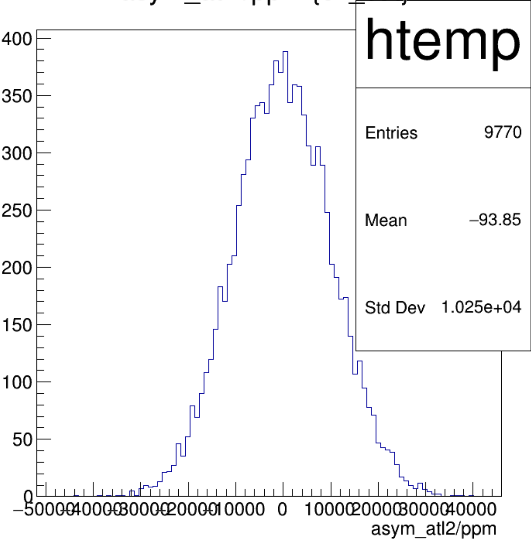
asym_atl2/ppm {ok_cut}
