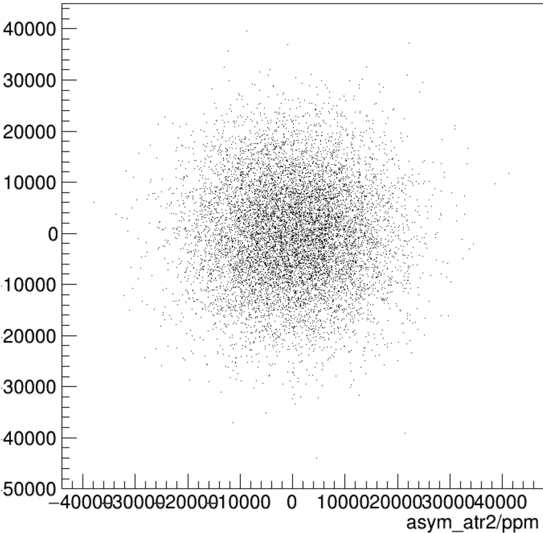
asym_atl2/ppm:asym_atr2/ppm {ok_cut}
