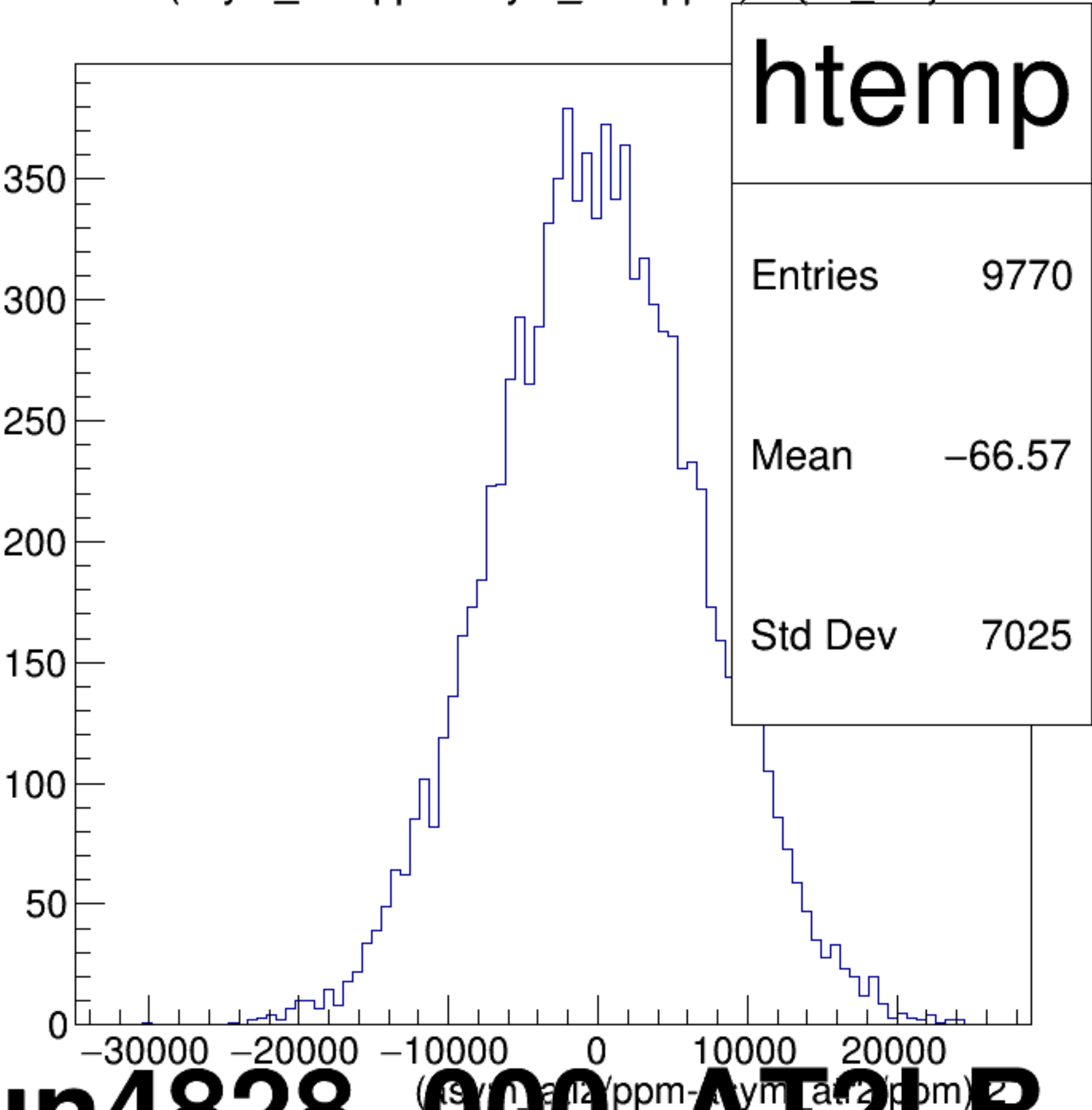
(asym_atl2/ppm-asym_atr2/ppm)/2 {ok_cut}
