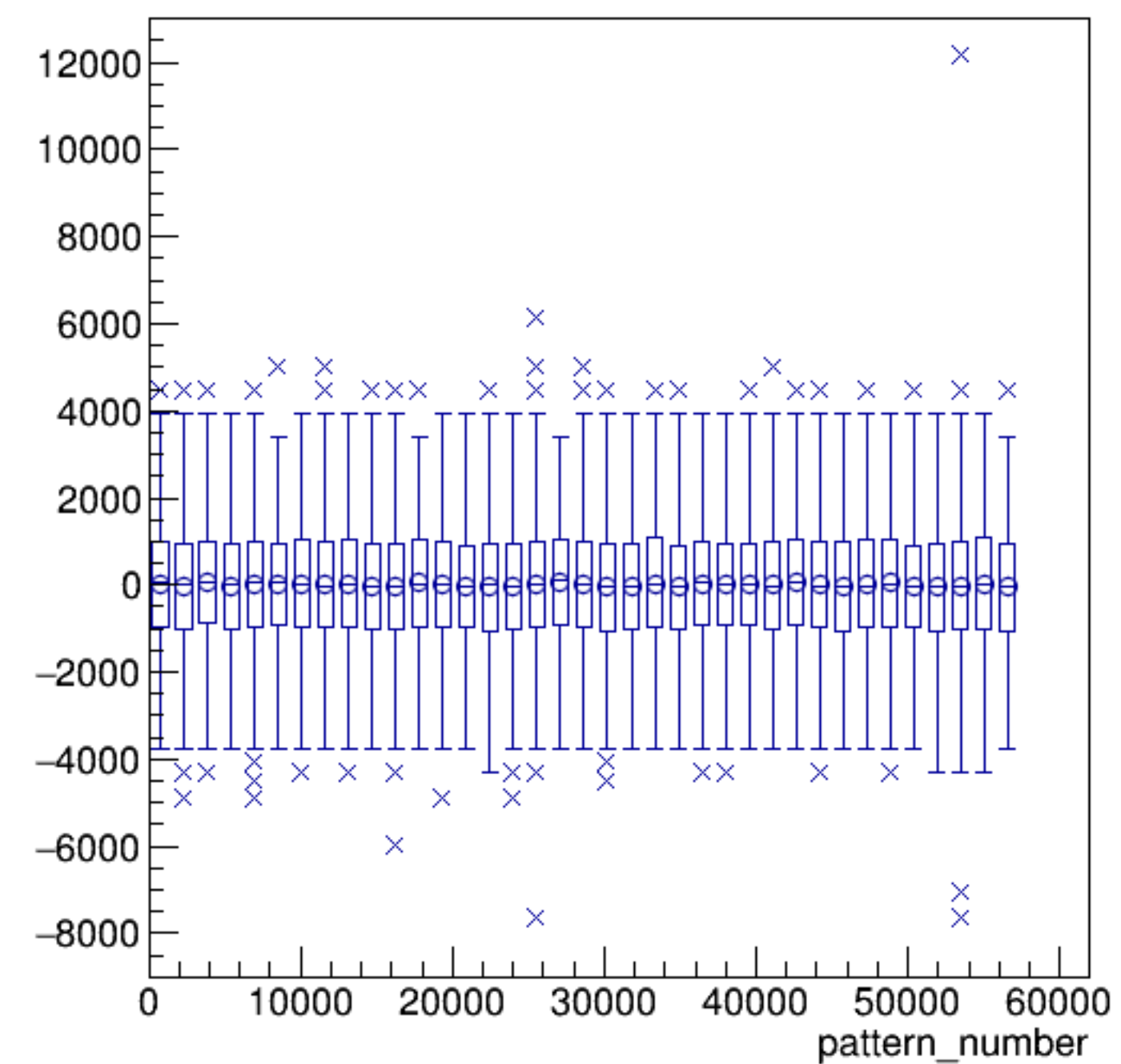
asym_sam8/ppm:pattern_number {ErrorFlag==0}
