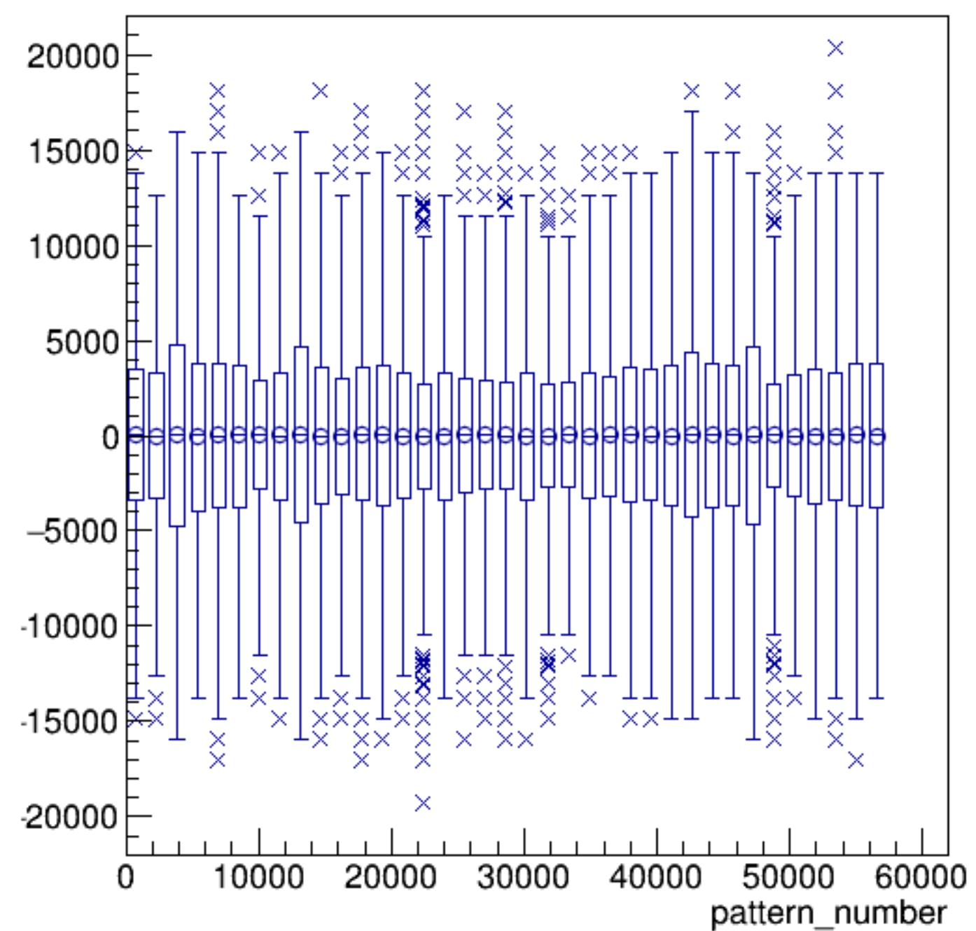
asym_sam8/ppm:pattern_number {ErrorFlag==0}
