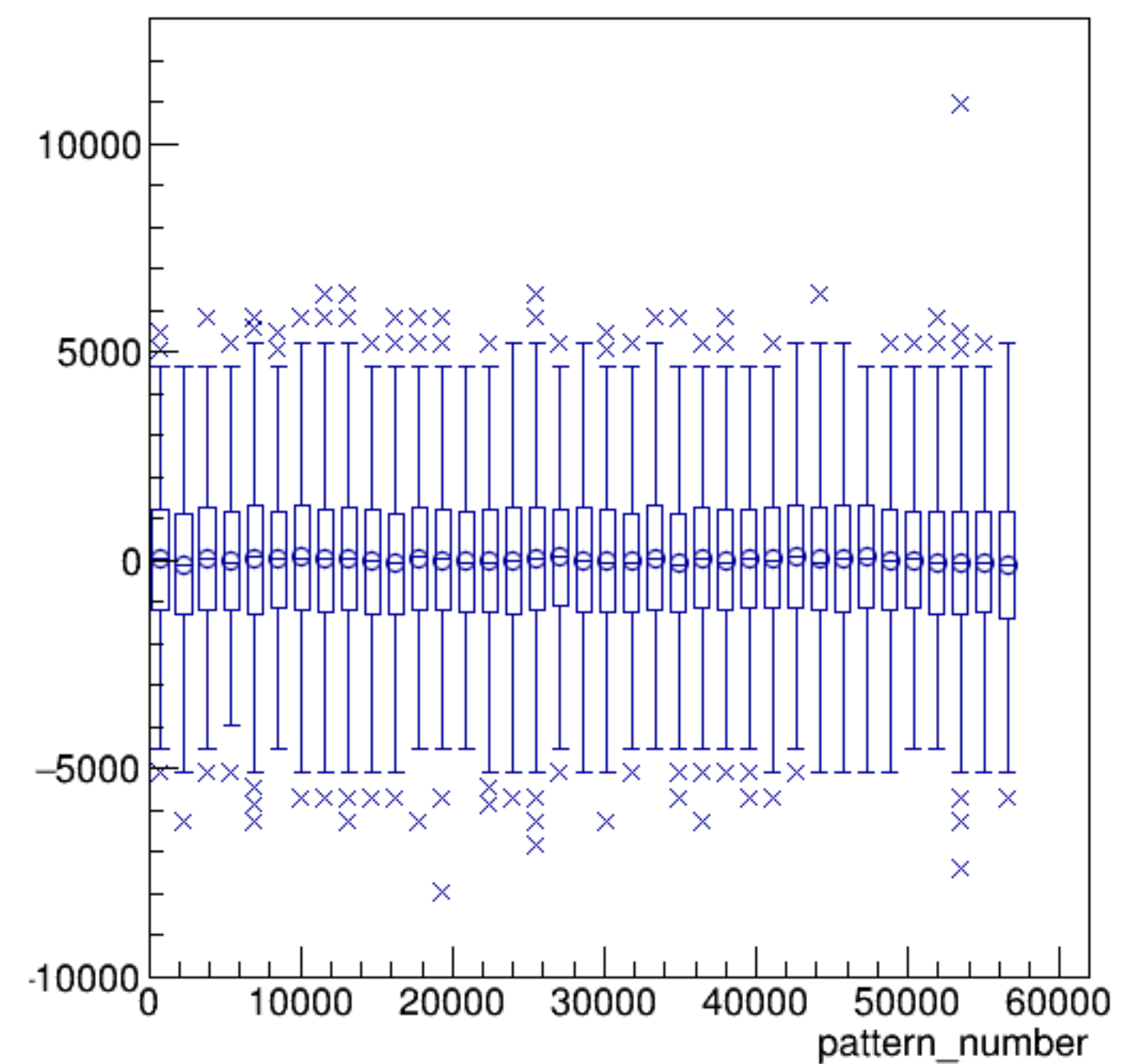
asym_sam6/ppm:pattern_number {ErrorFlag==0}
