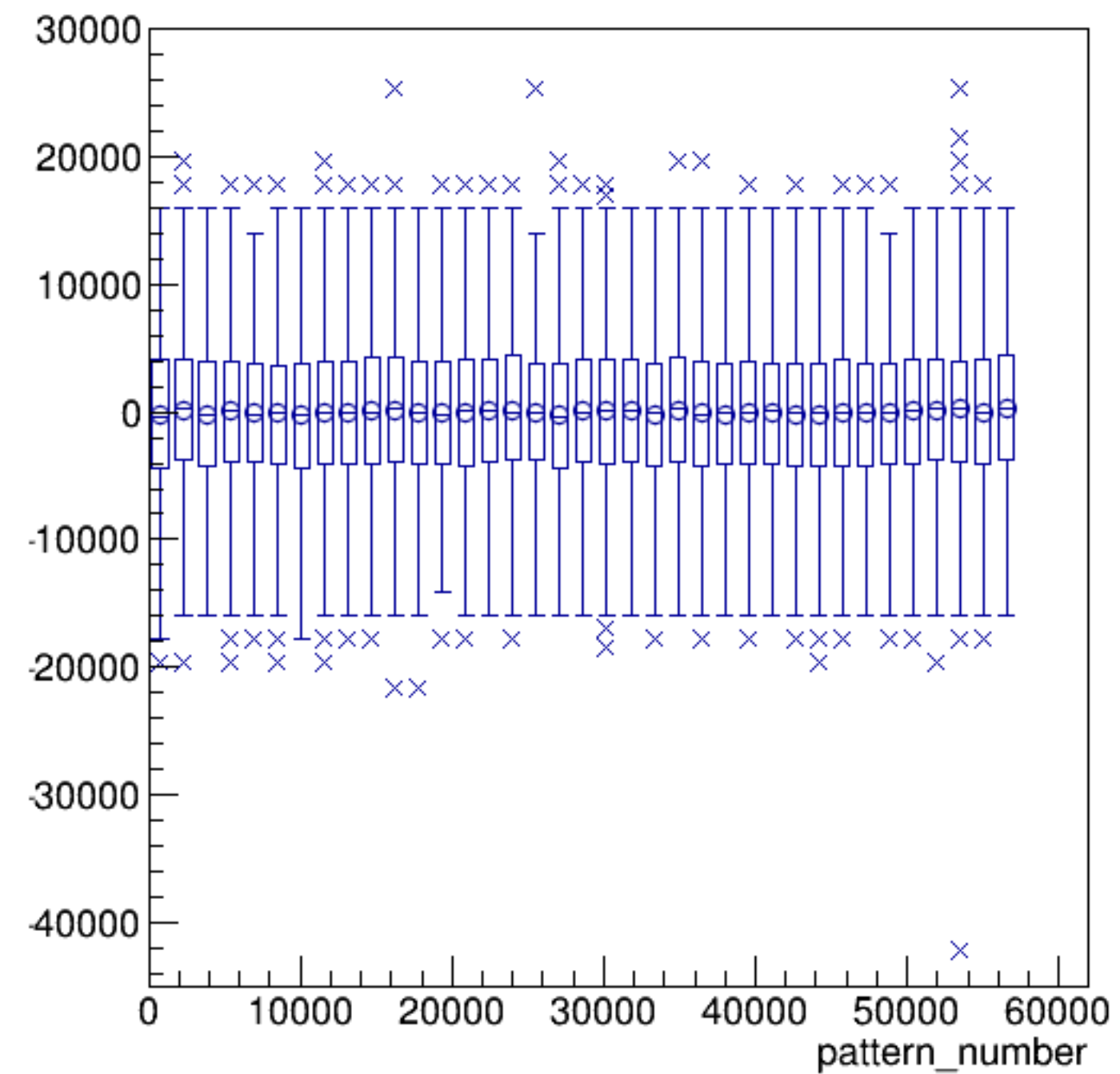
asym_sam2/ppm:pattern_number {ErrorFlag==0}
