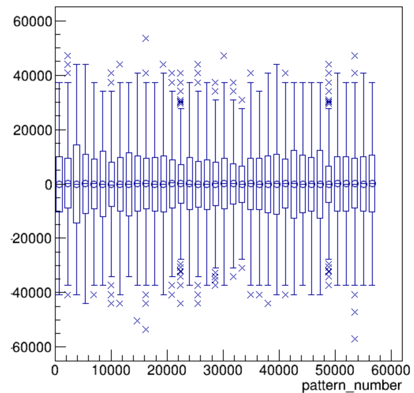
asym_sam4/ppm:pattern_number {ErrorFlag==0}
