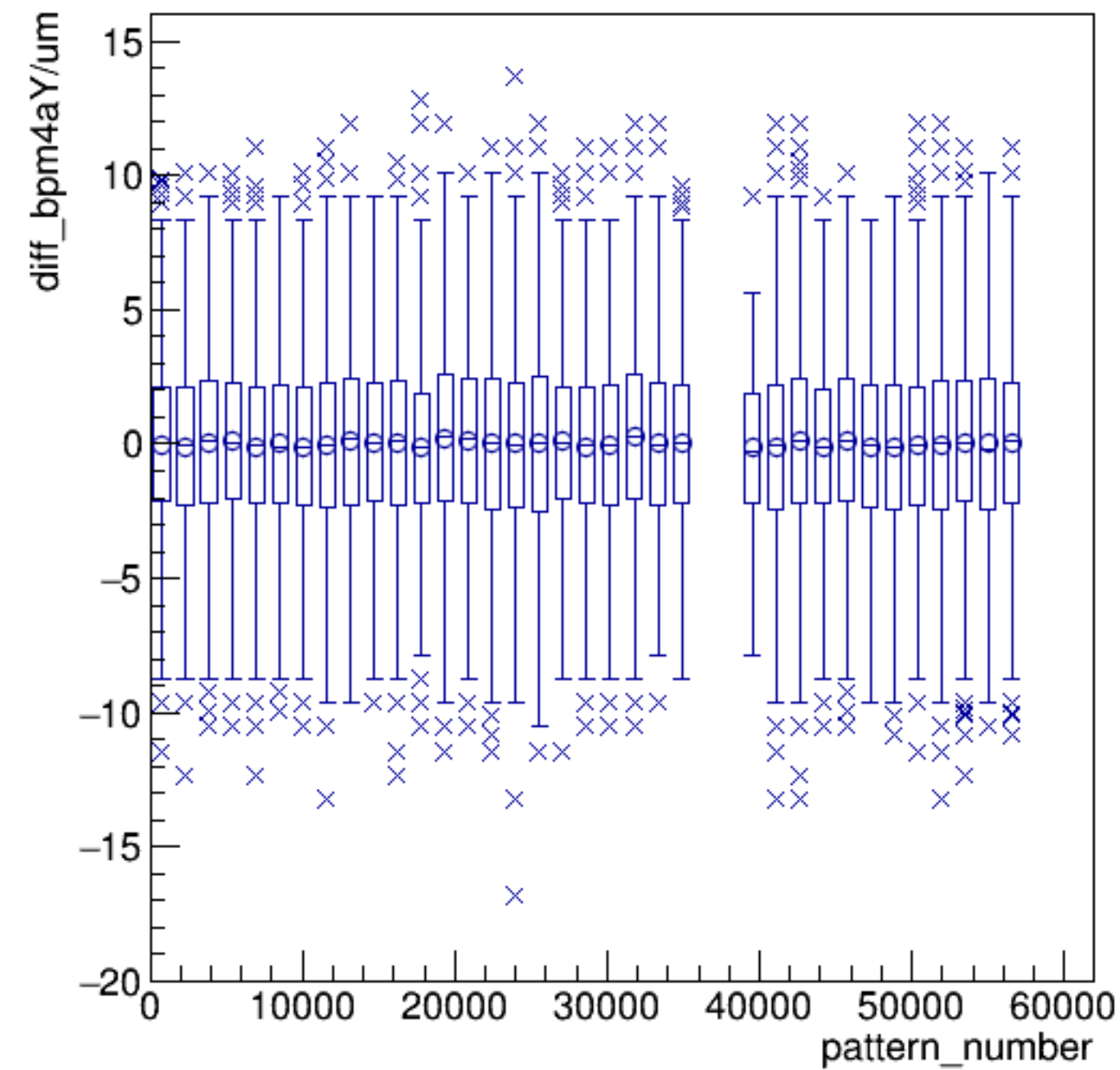
diff_bpm4aY/um:pattern_number {ErrorFlag==0}
