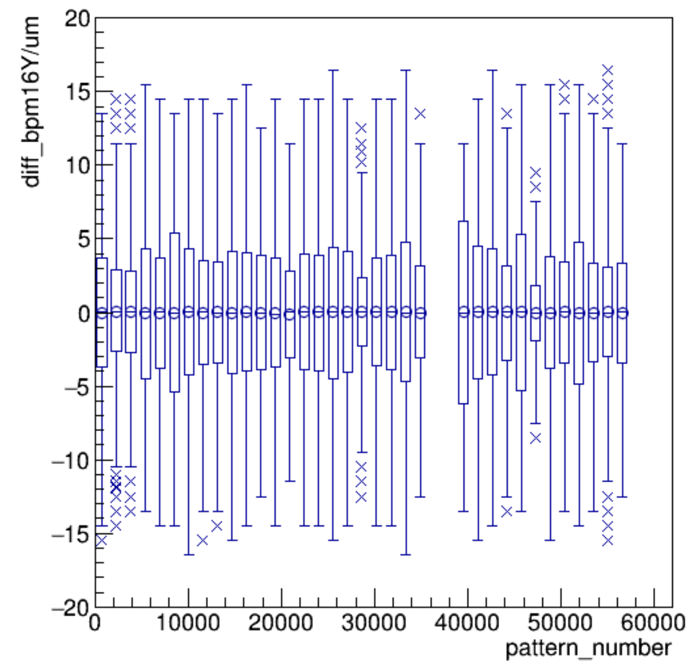
diff_bpm16Y/um:pattern_number {ErrorFlag==0}
