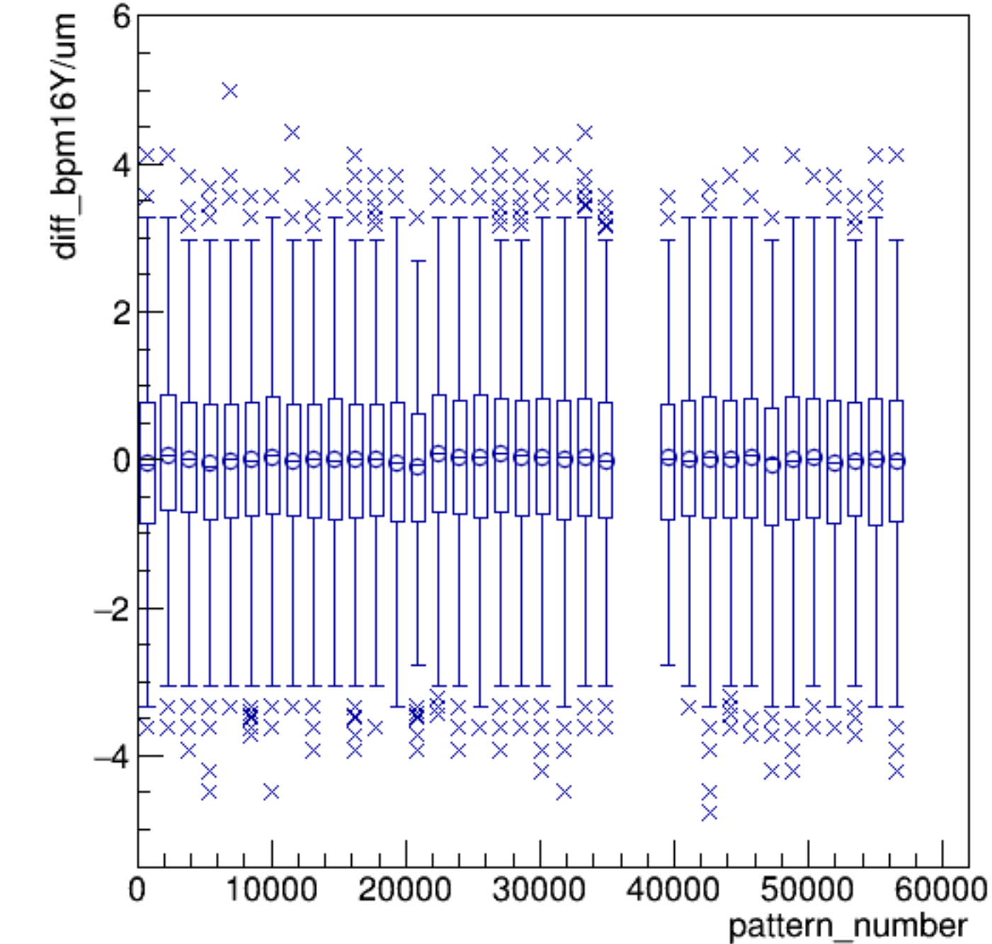
diff_bpm16Y/um:pattern_number {ErrorFlag==0}
