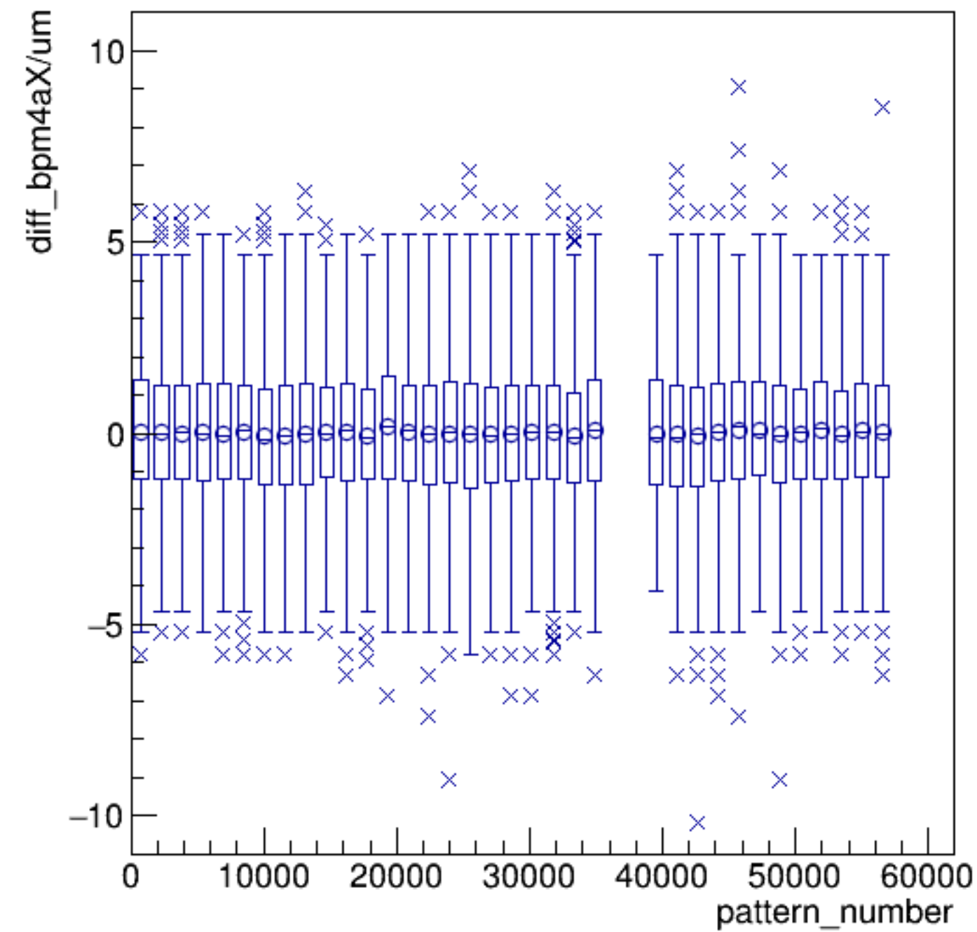
diff_bpm4aX/um:pattern_number {ErrorFlag==0}
