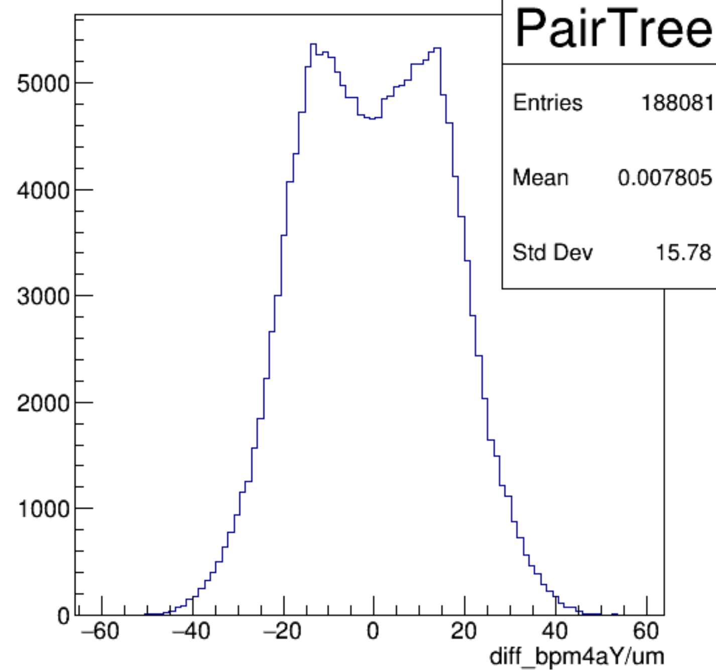
diff_bpm4aY/um {ErrorFlag==0}
