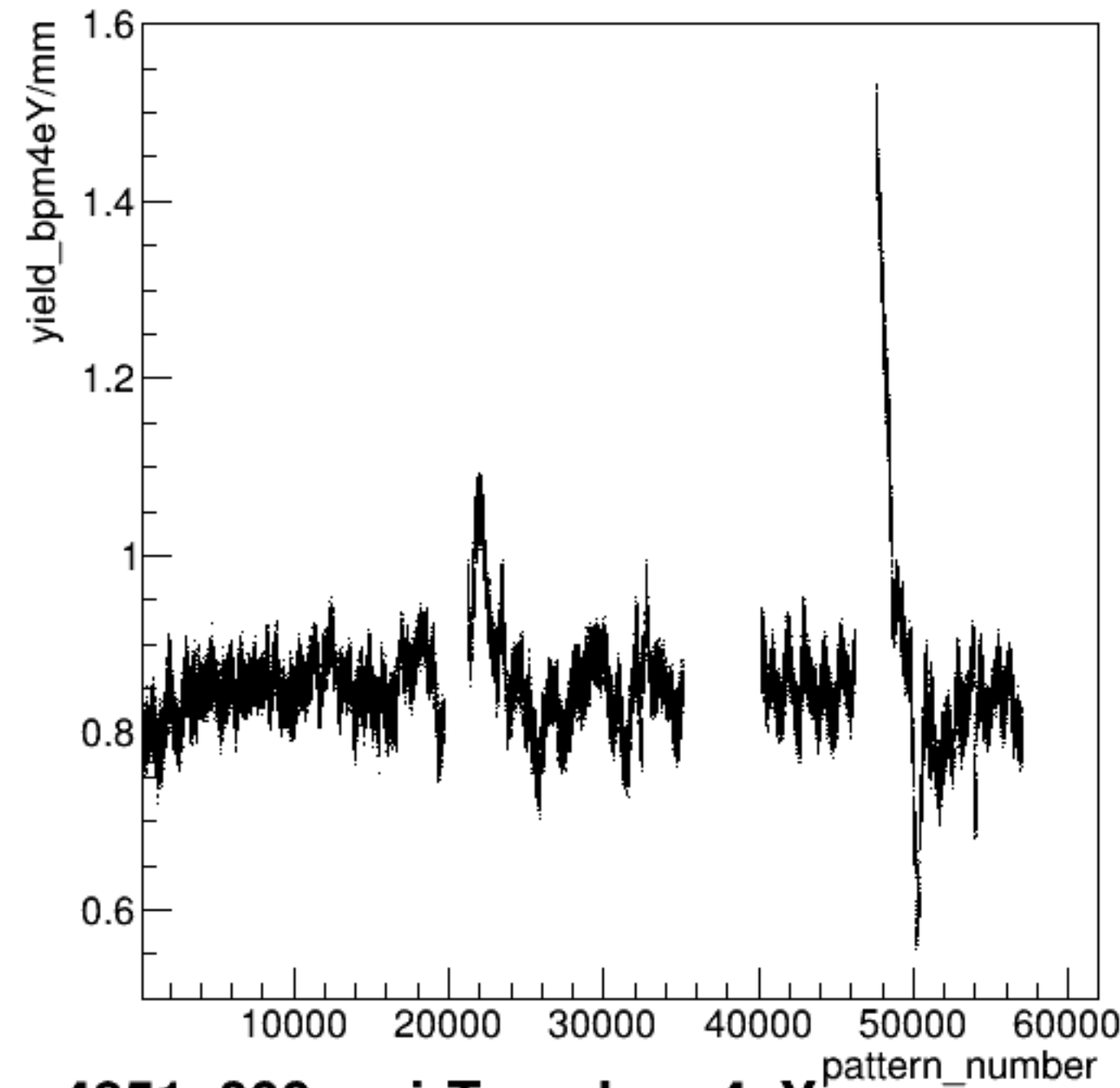
yield_bpm4eY/mm:pattern_number {ErrorFlag==0}
