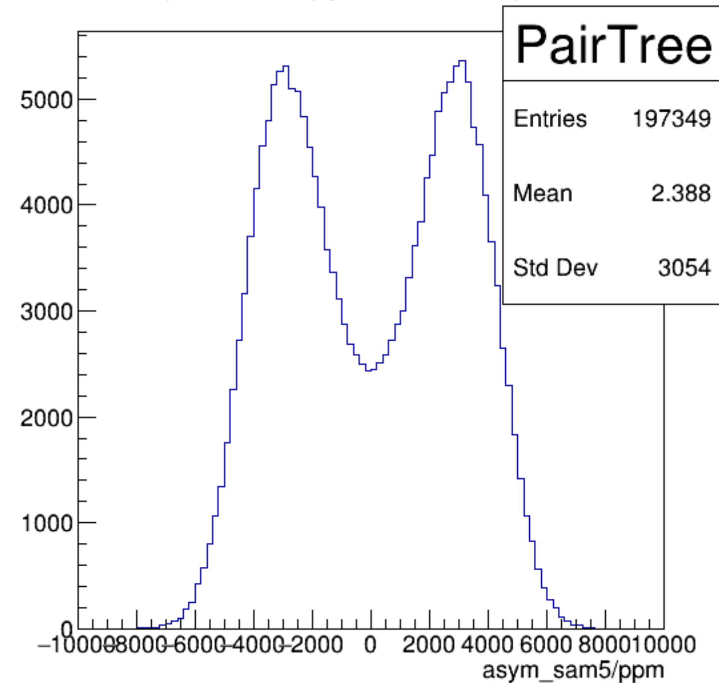
asym_sam5/ppm {ErrorFlag==0}
