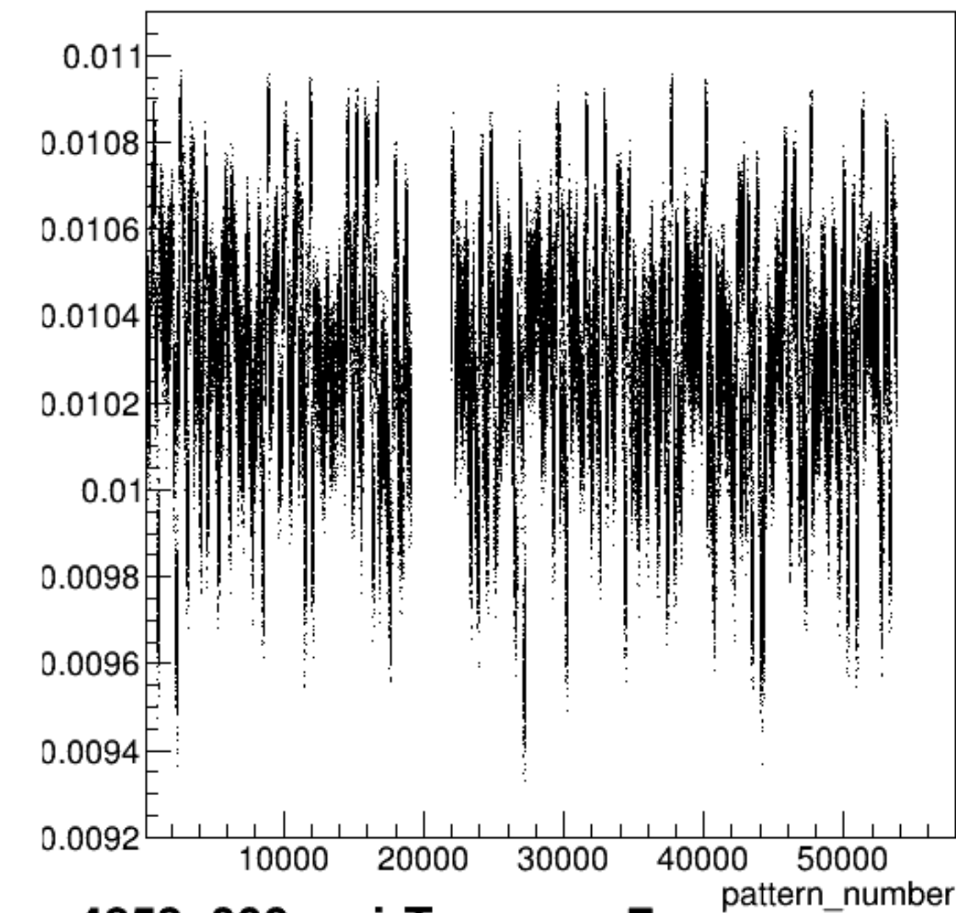
yield_sam7:pattern_number {ErrorFlag==0}
