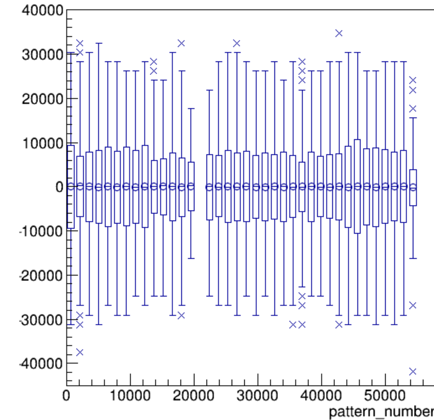
asym_sam6/ppm:pattern_number {ErrorFlag==0}
