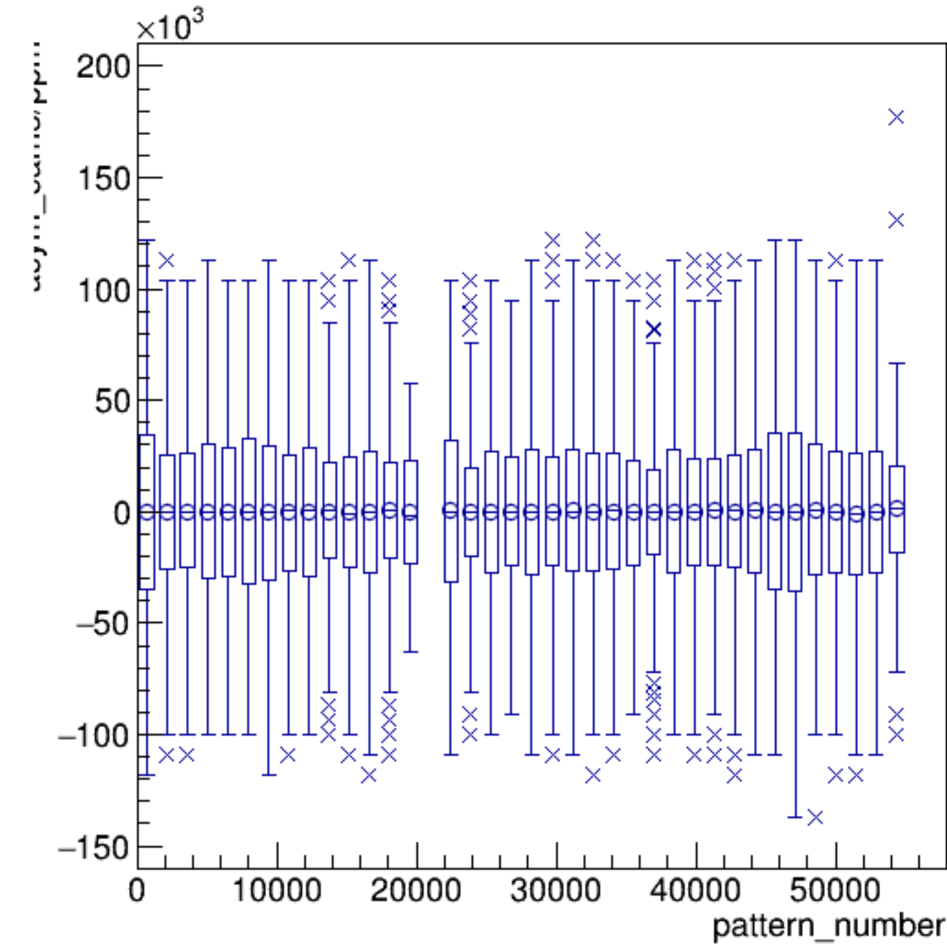
asym_sam3/ppm:pattern_number {ErrorFlag==0}
