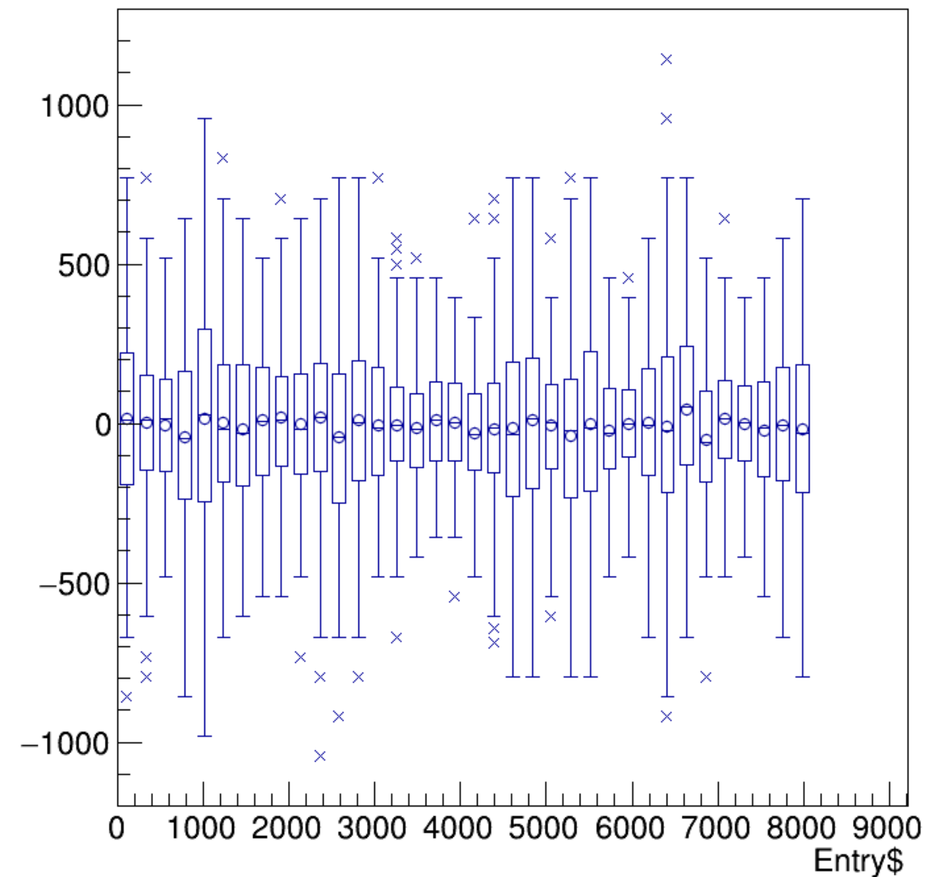
asym_bpm0i07WS/ppm:Entry$ {ErrorFlag==0}
