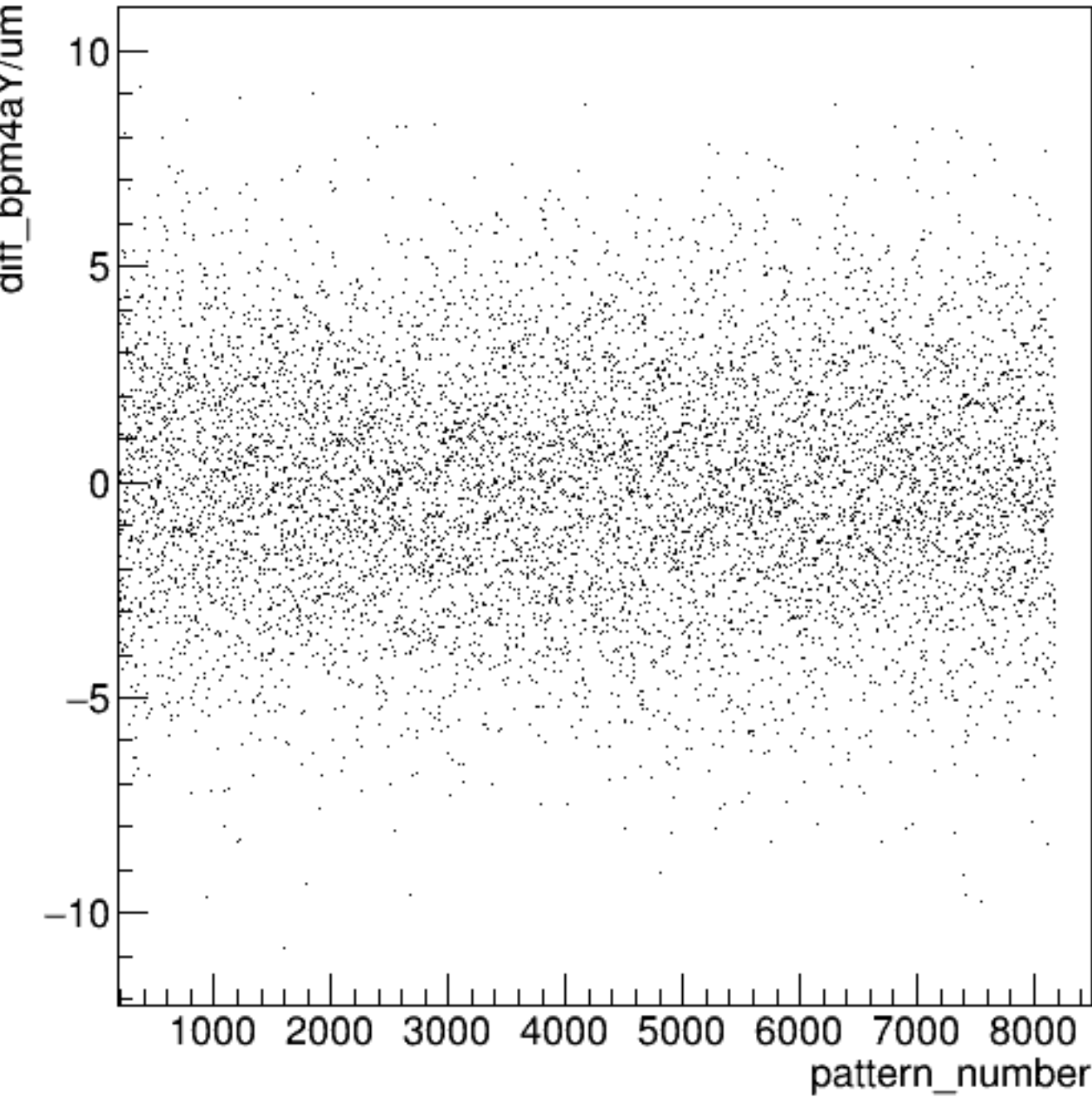
diff_bpm4aY/um:pattern_number {ErrorFlag==0}
