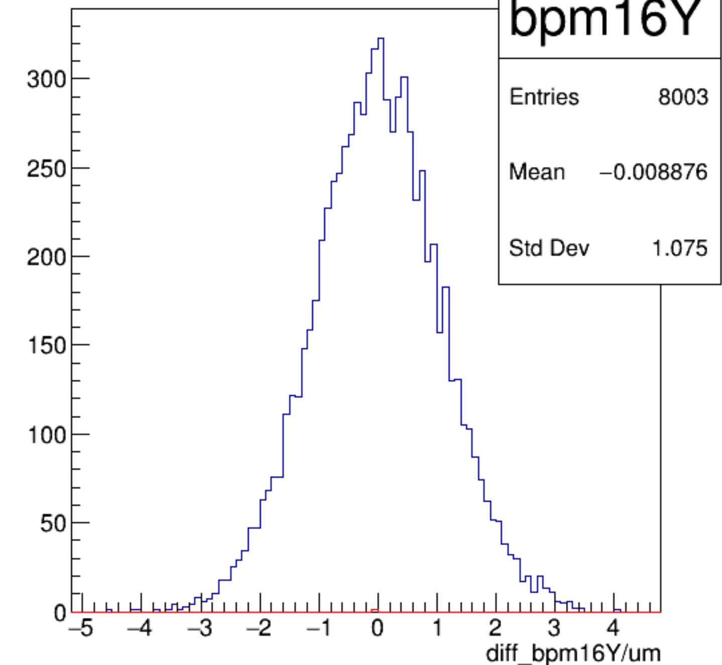
diff_bpm16Y/um {ErrorFlag==0}
