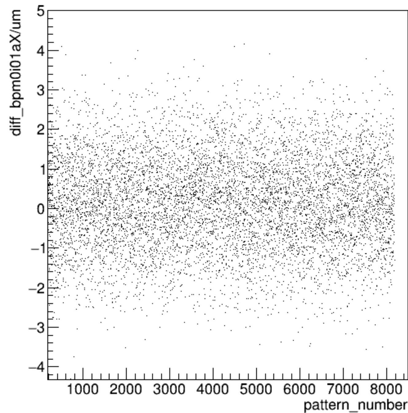
diff_bpm0i01aX/um:pattern_number {ErrorFlag==0}
