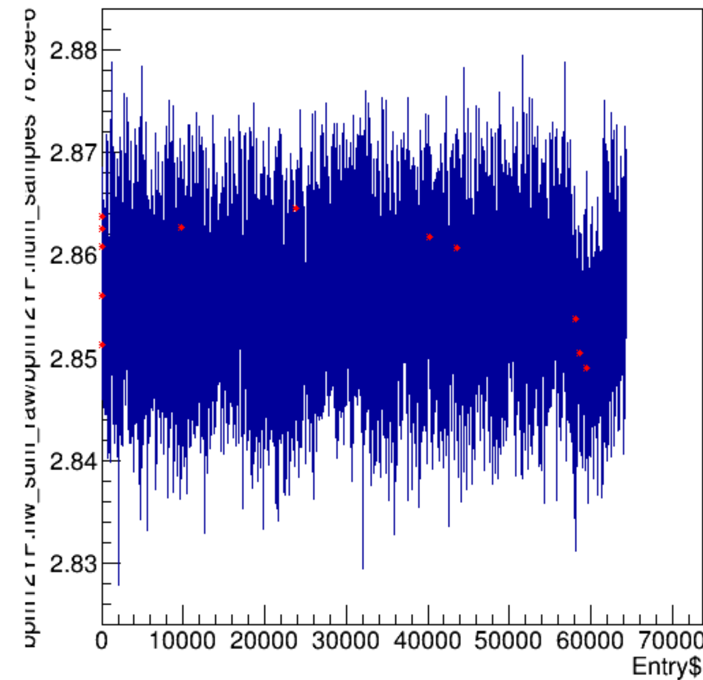
bpm12YP.hw_sum_raw/bpm12YP.num_samples*76.29e-6:Entry$
