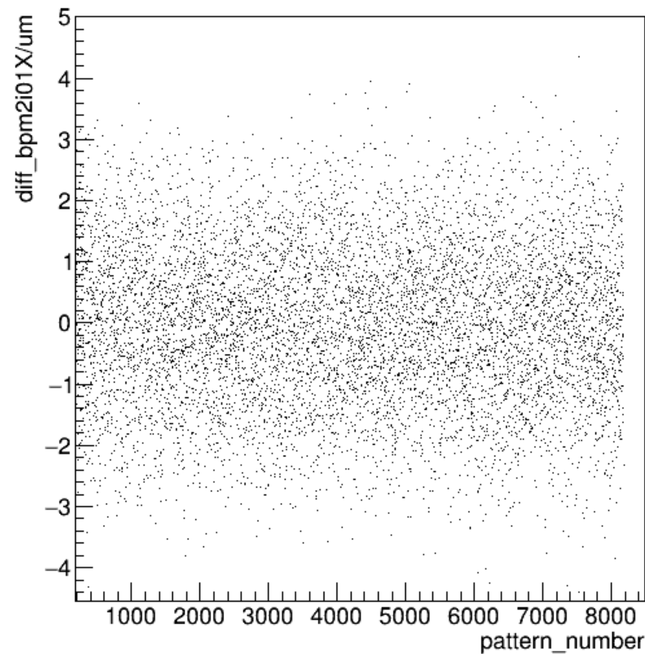
diff_bpm2i01X/um:pattern_number {ErrorFlag==0}
