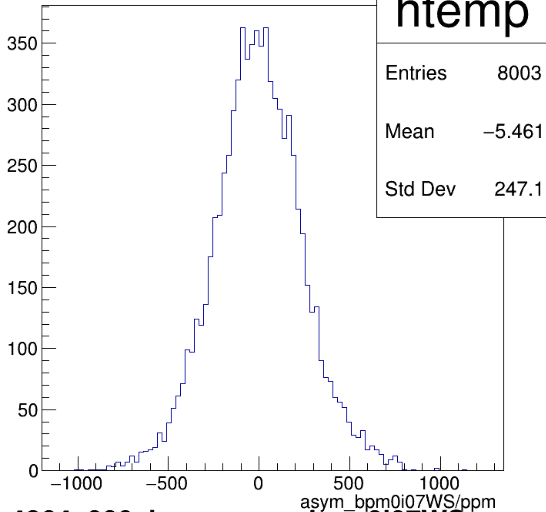
asym_bpm0i07WS/ppm {ErrorFlag==0}
