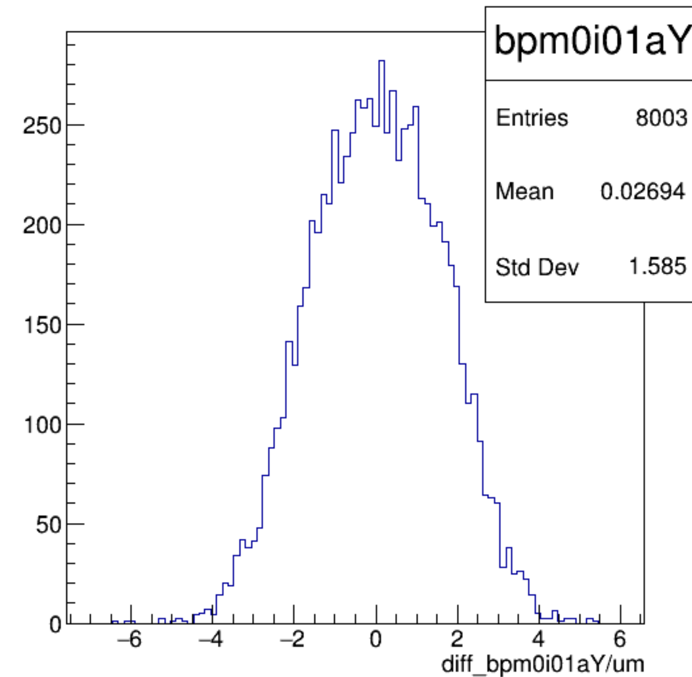
diff_bpm0i01aY/um {ErrorFlag==0}
