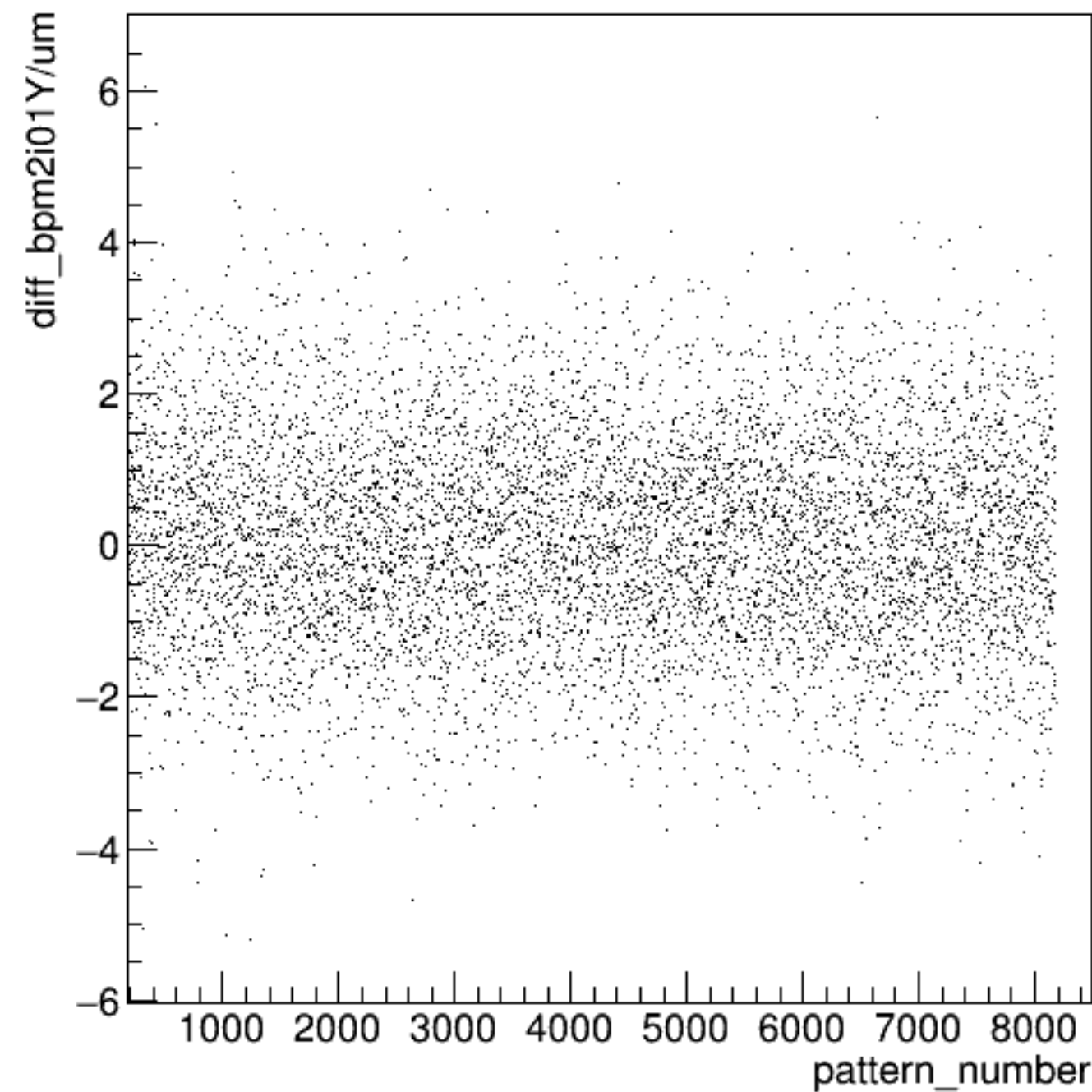
diff_bpm2i01Y/um:pattern_number {ErrorFlag==0}
