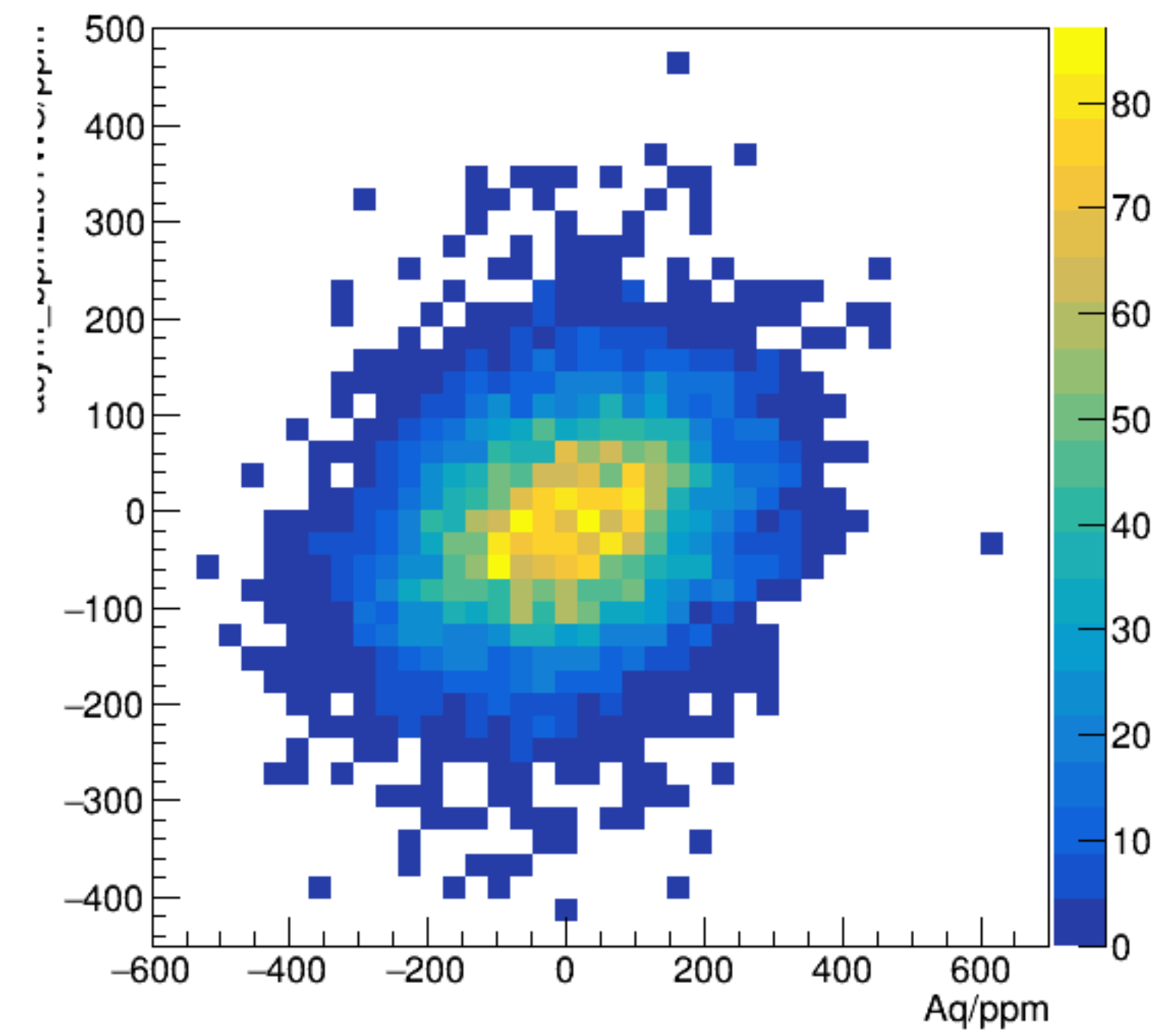
asym_bpm2i01WS/ppm:Aq/ppm {ErrorFlag==0}
