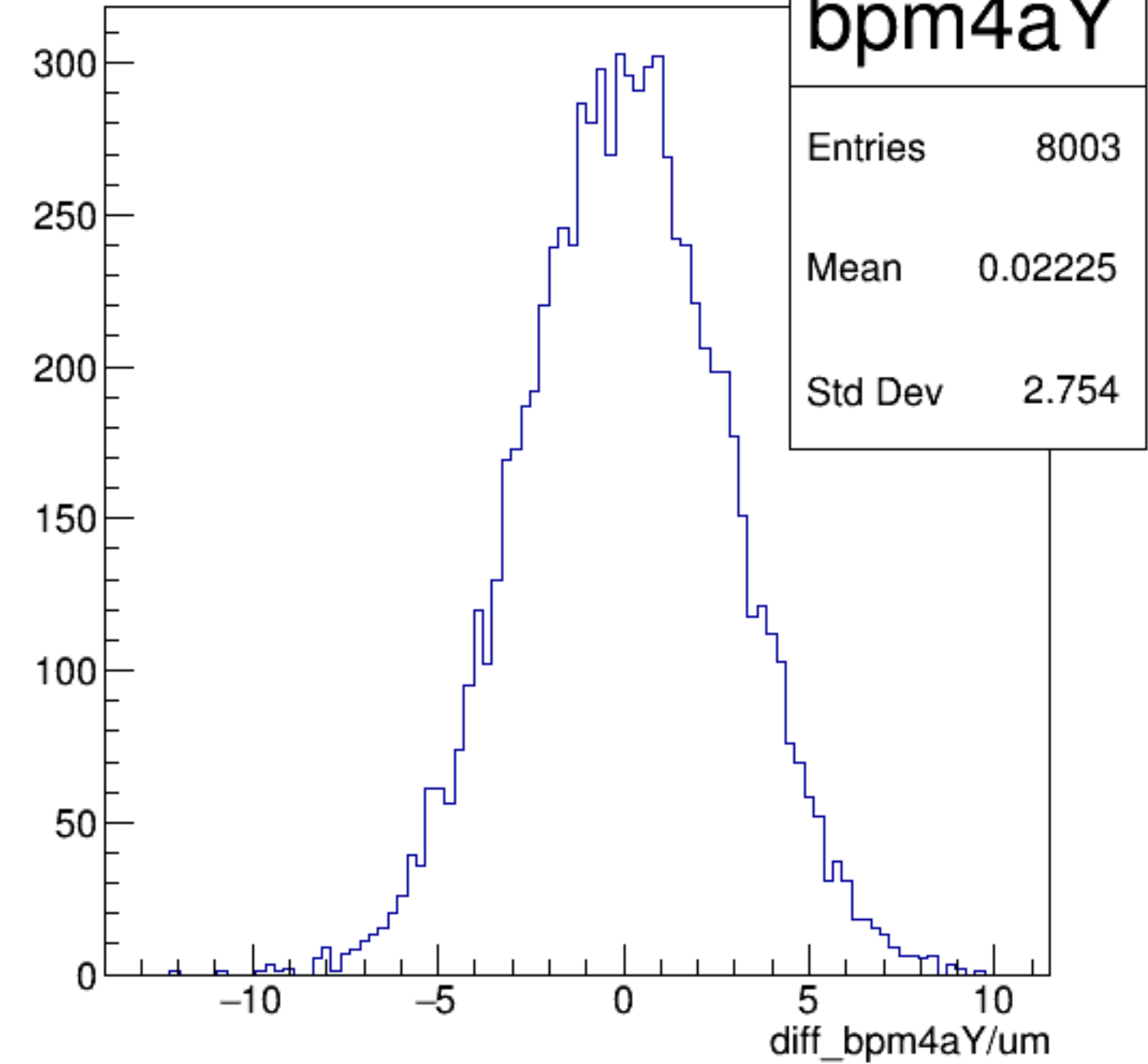
diff_bpm4aY/um {ErrorFlag==0}
