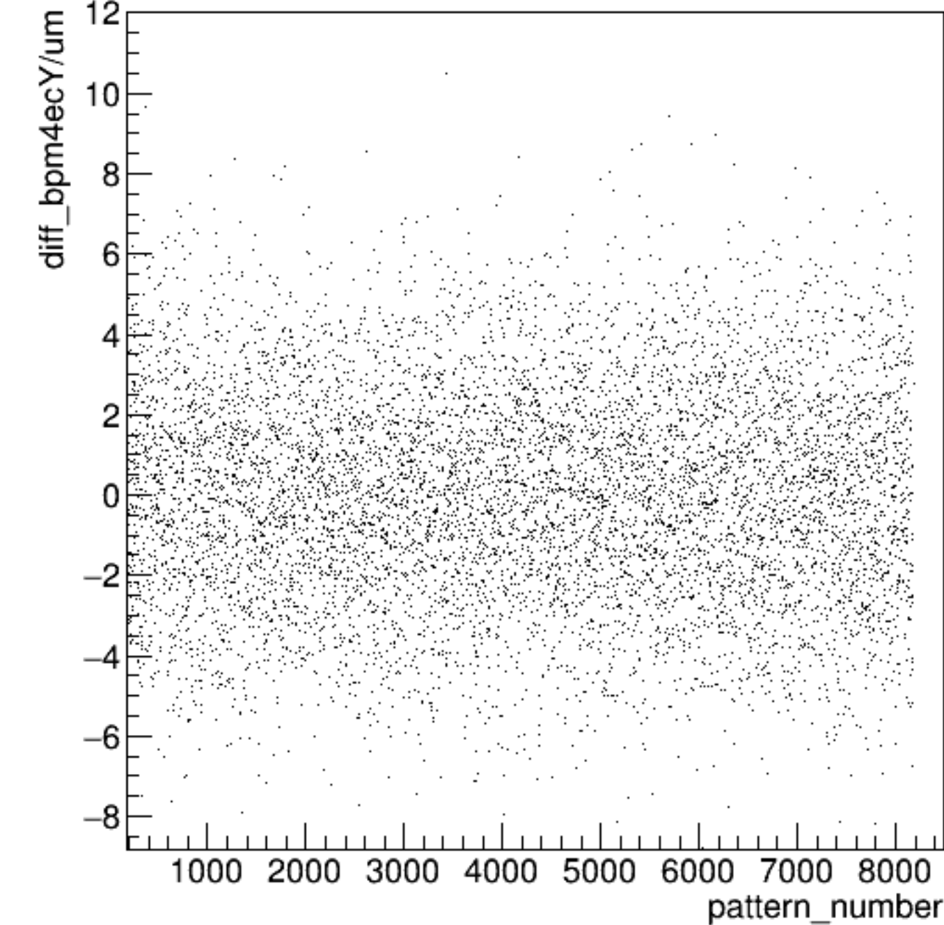
diff_bpm4ecY/um:pattern_number {ErrorFlag==0}
