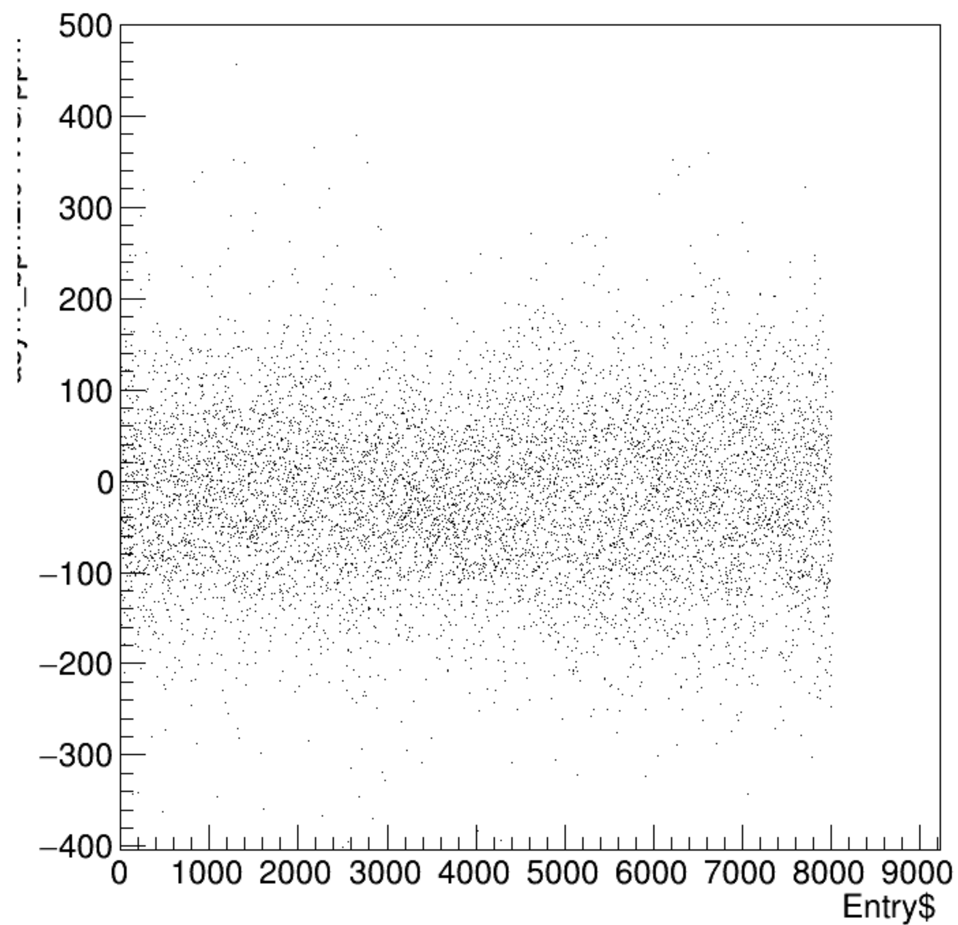
asym_bpm2i01WS/ppm:Entry$ {ErrorFlag==0}
