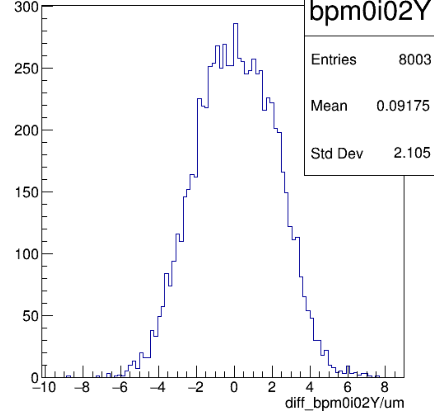
diff_bpm0i02Y/um {ErrorFlag==0}
