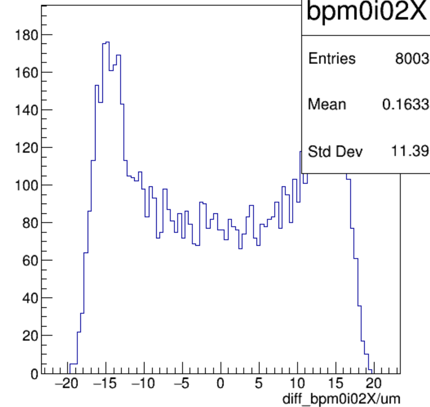
diff_bpm0i02X/um {ErrorFlag==0}
