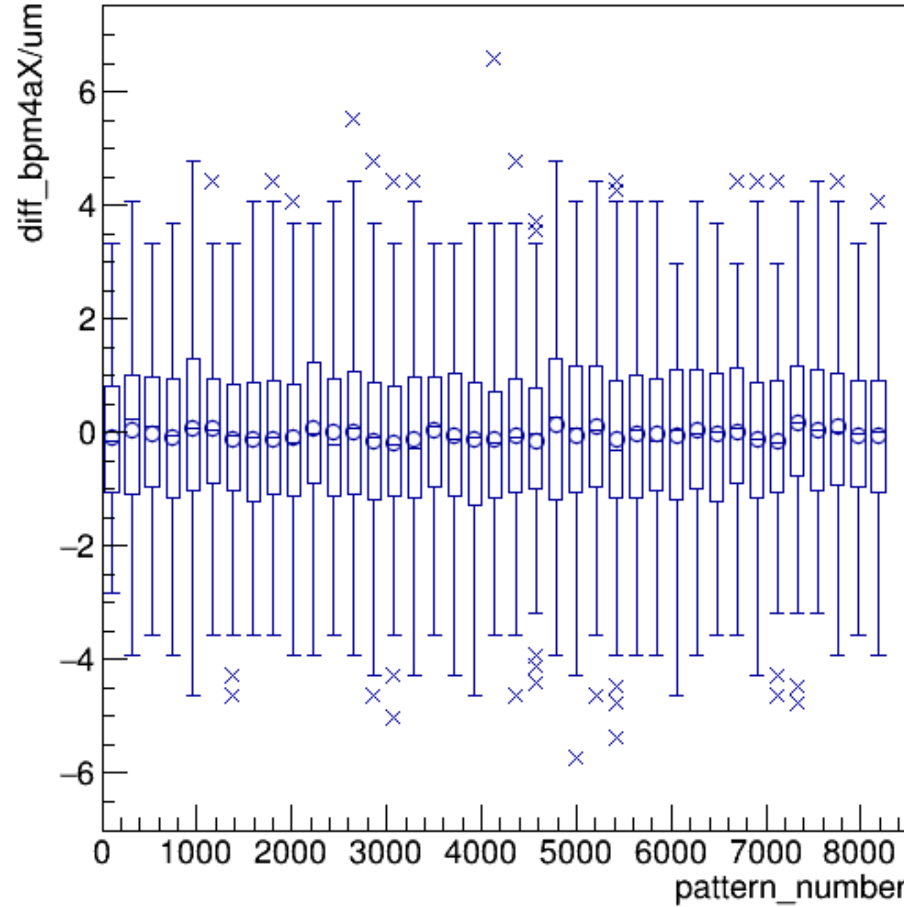
diff_bpm4aX/um:pattern_number {ErrorFlag==0}
