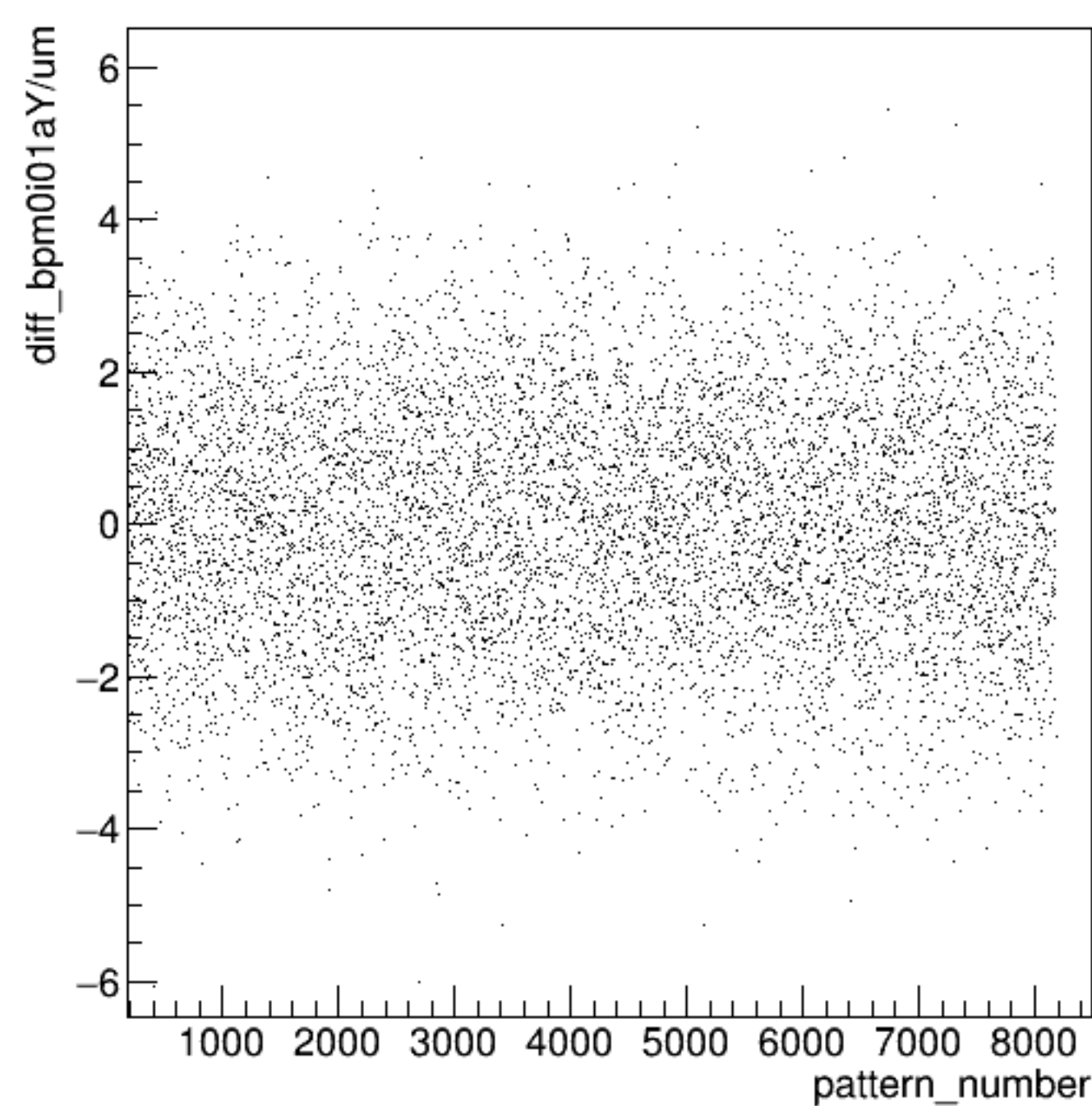
diff_bpm0i01aY/um:pattern_number {ErrorFlag==0}
