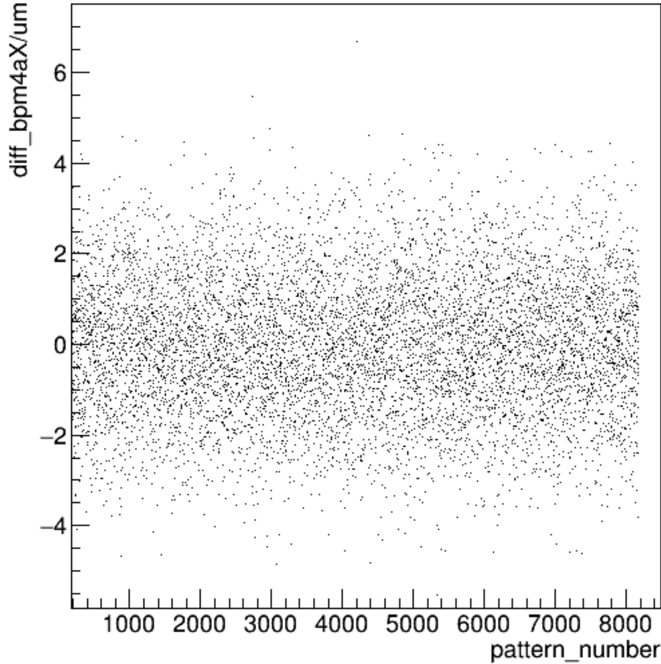
diff_bpm4aX/um:pattern_number {ErrorFlag==0}
