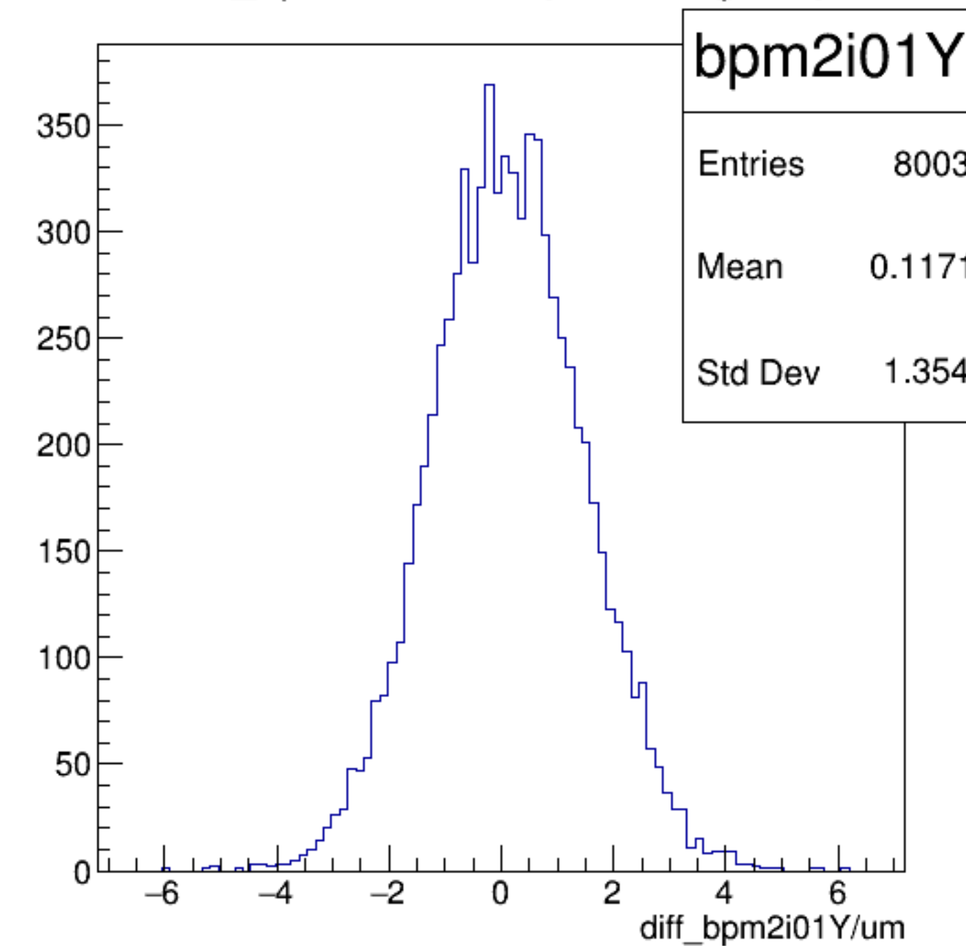
diff_bpm2i01Y/um {ErrorFlag==0}
