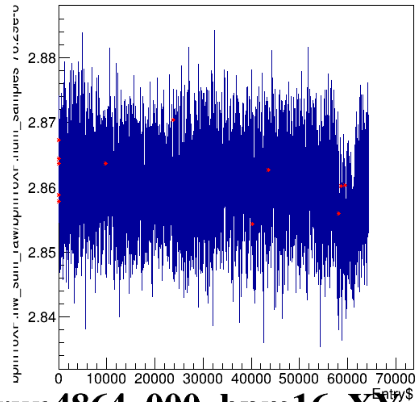
bpm16XP.hw_sum_raw/bpm16XP.num_samples*76.29e-6:Entry$
