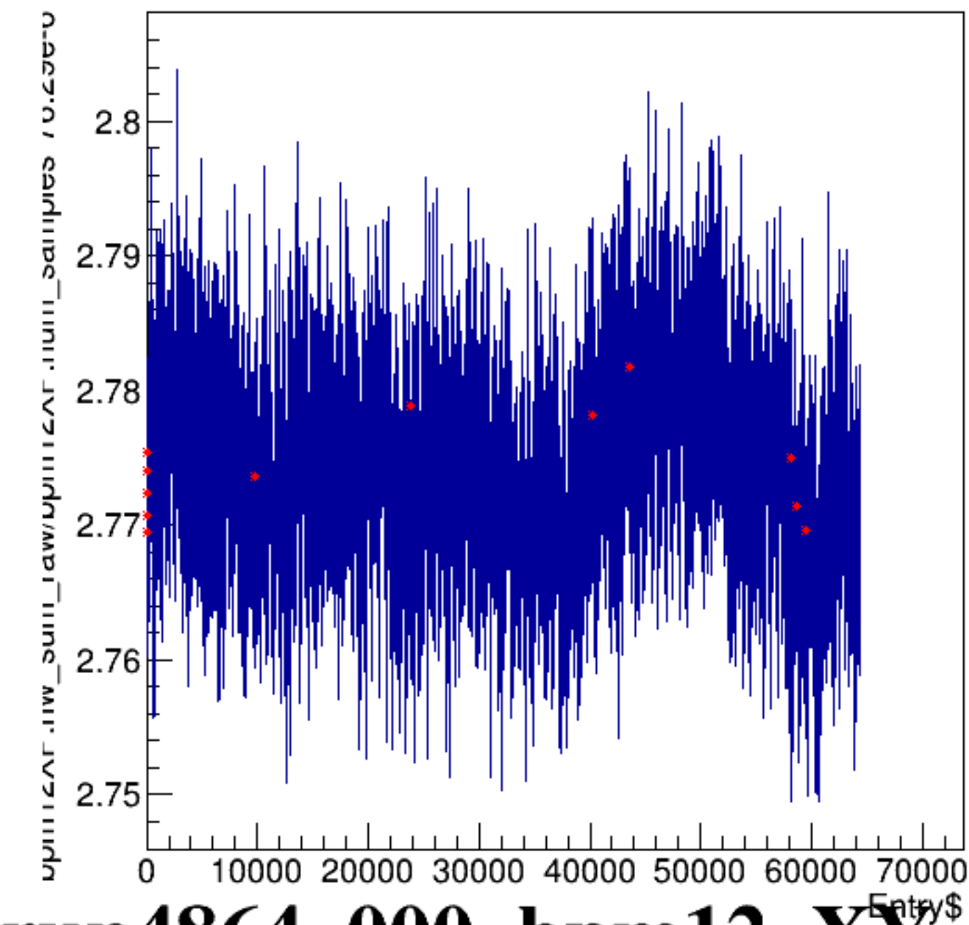
bpm12XP.hw_sum_raw/bpm12XP.num_samples*76.29e-6:Entry$
