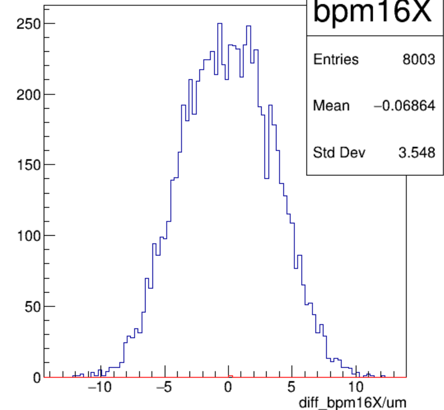
diff_bpm16X/um {ErrorFlag==0}
