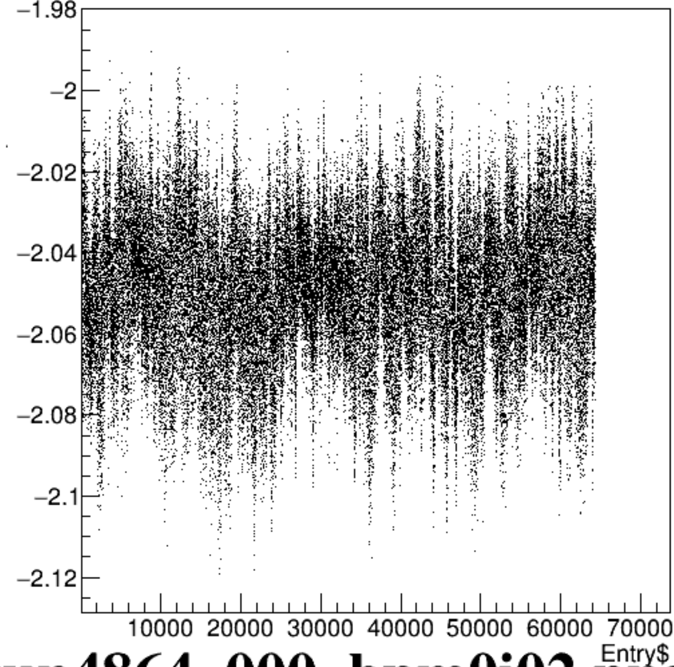
bpm0i02Y/mm:Entry$ {ErrorFlag==0}
