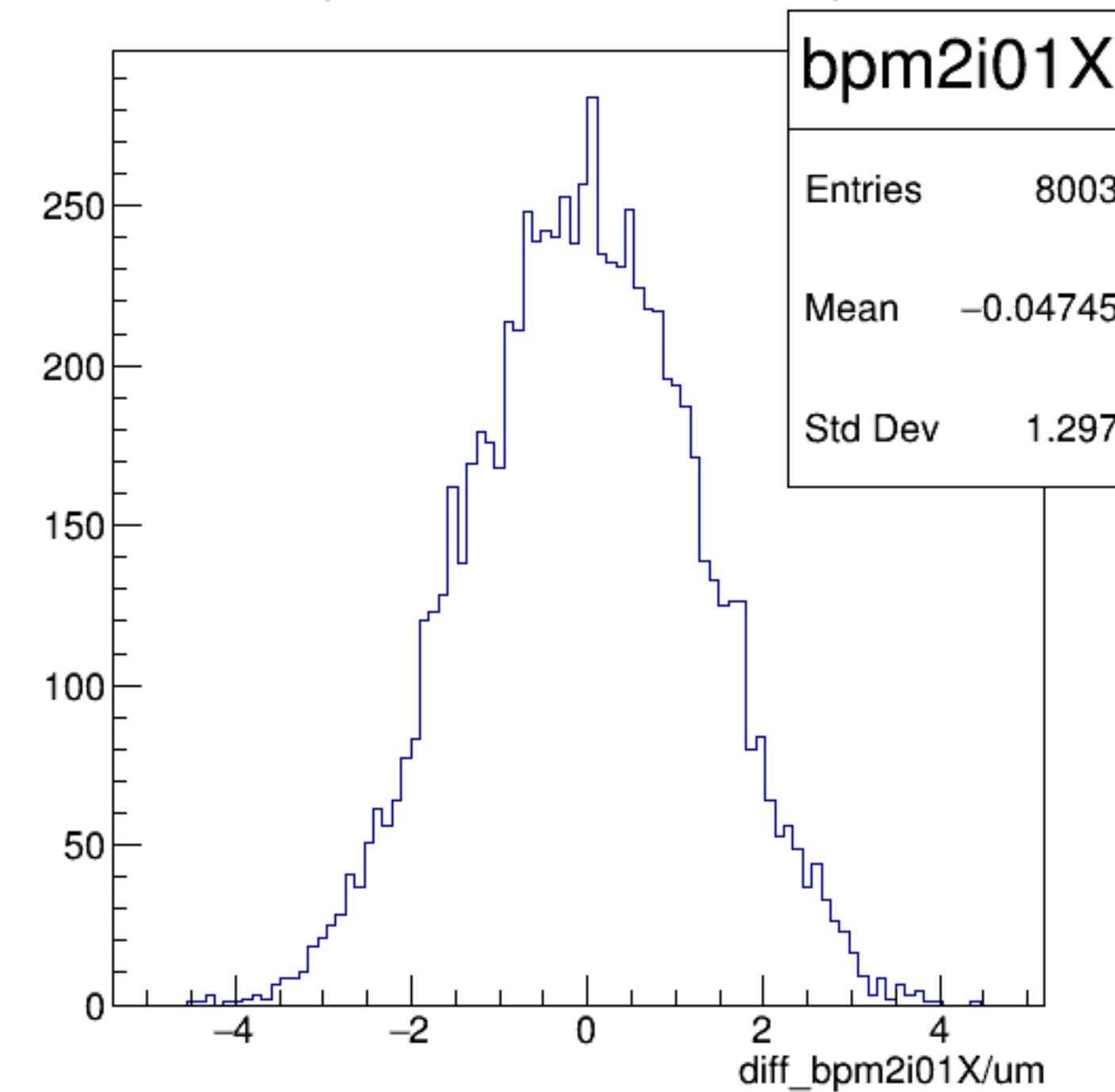
diff_bpm2i01X/um {ErrorFlag==0}
