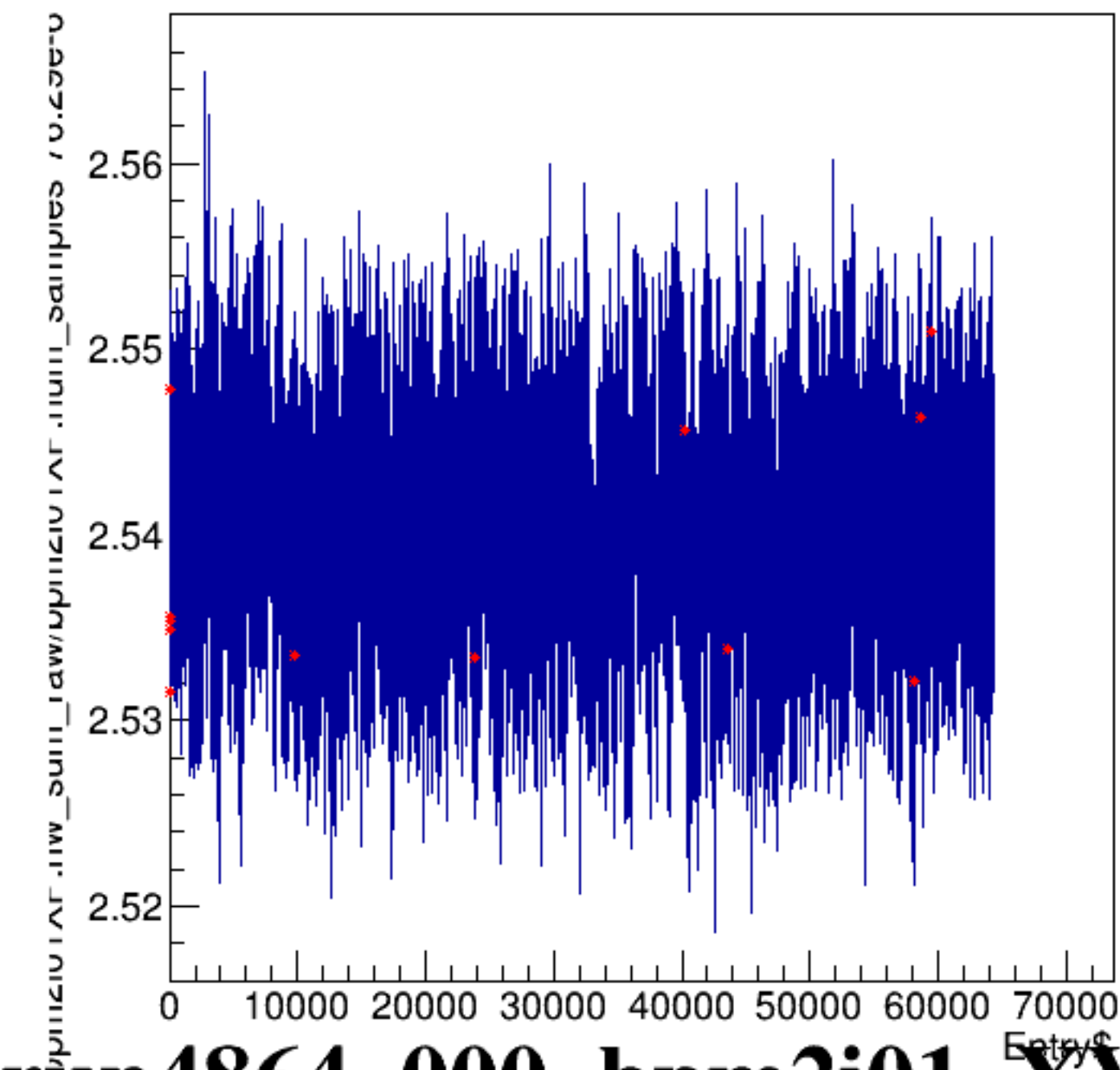
bpm2i01XP.hw_sum_raw/bpm2i01XP.num_samples*76.29e-6:Entry$
