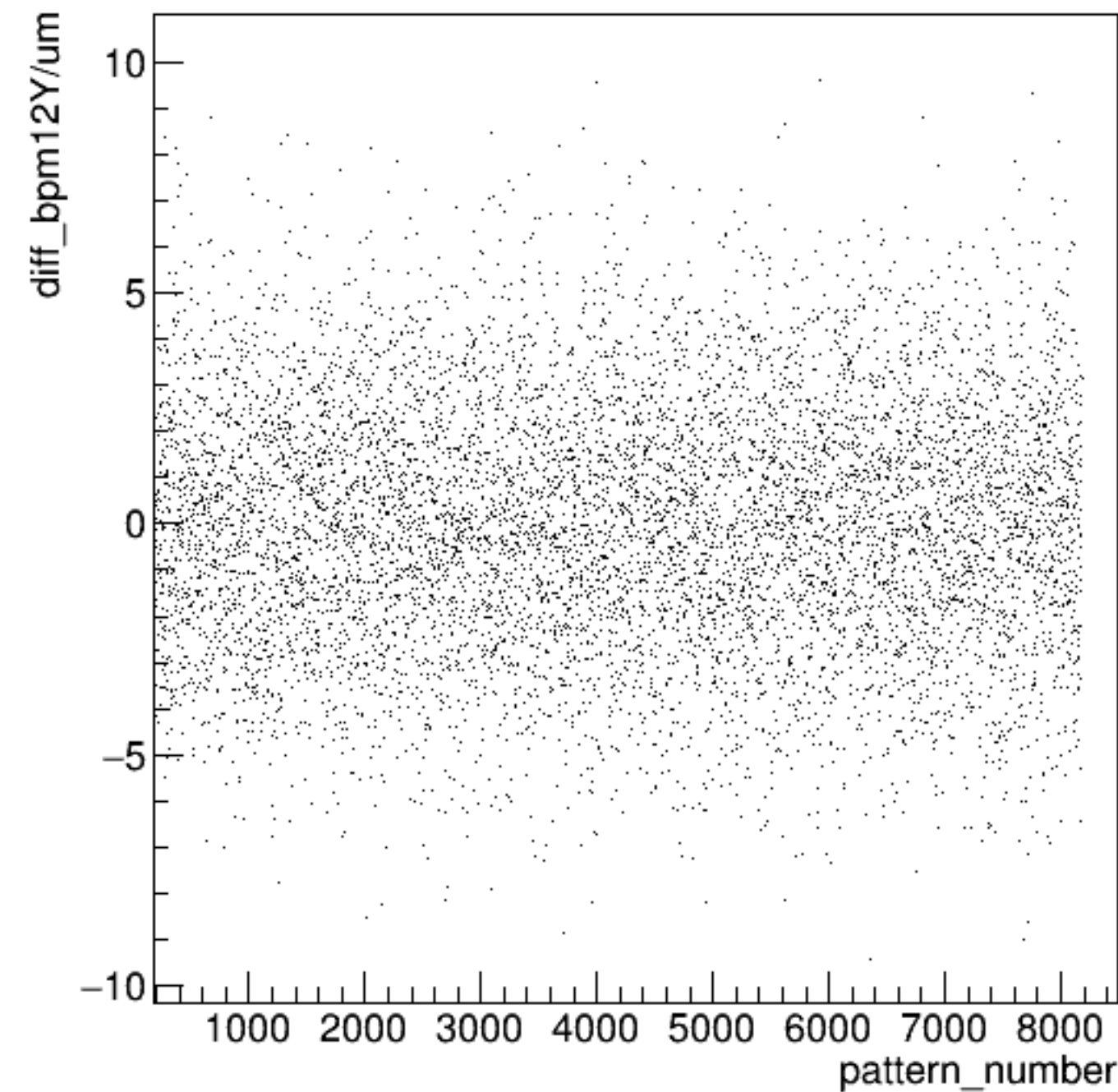
diff_bpm12Y/um:pattern_number {ErrorFlag==0}
