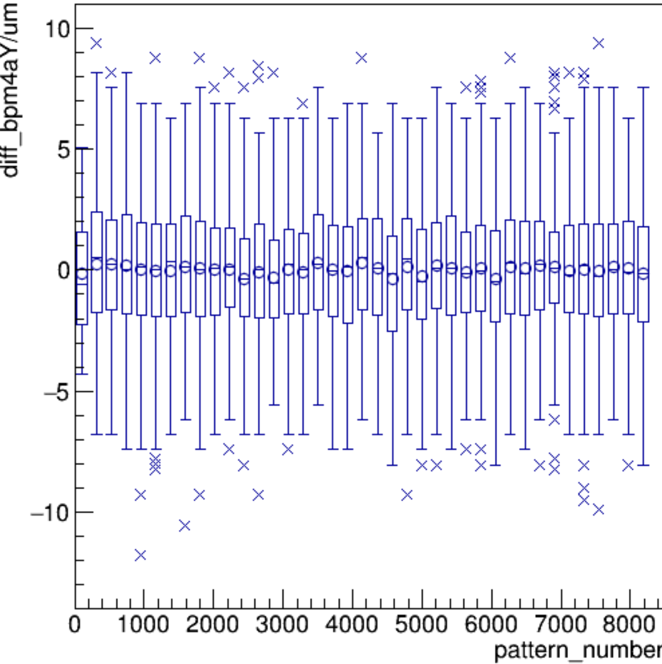
diff_bpm4aY/um:pattern_number {ErrorFlag==0}
