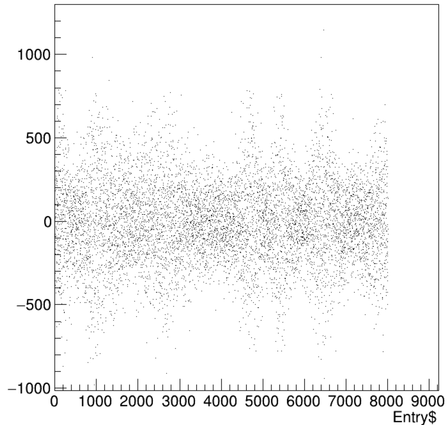
asym_bpm0i07WS/ppm:Entry$ {ErrorFlag==0}
