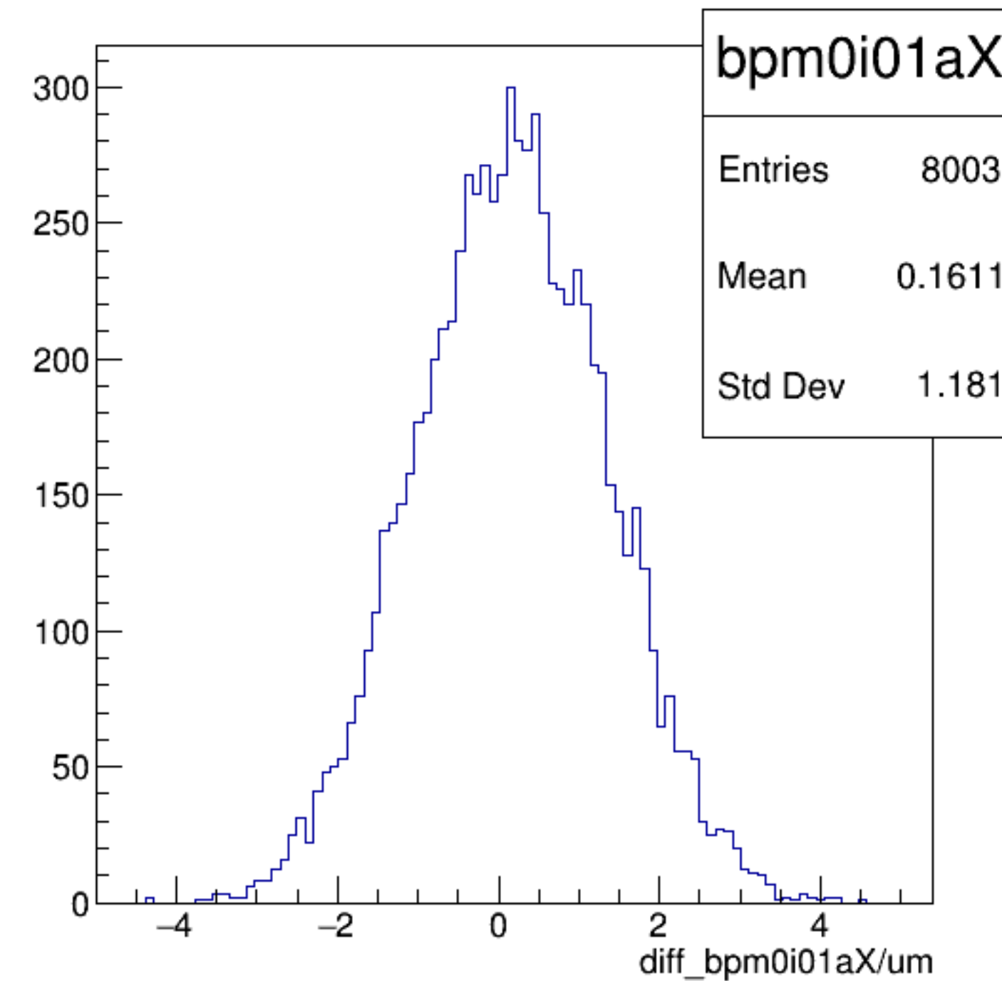
diff_bpm0i01aX/um {ErrorFlag==0}
