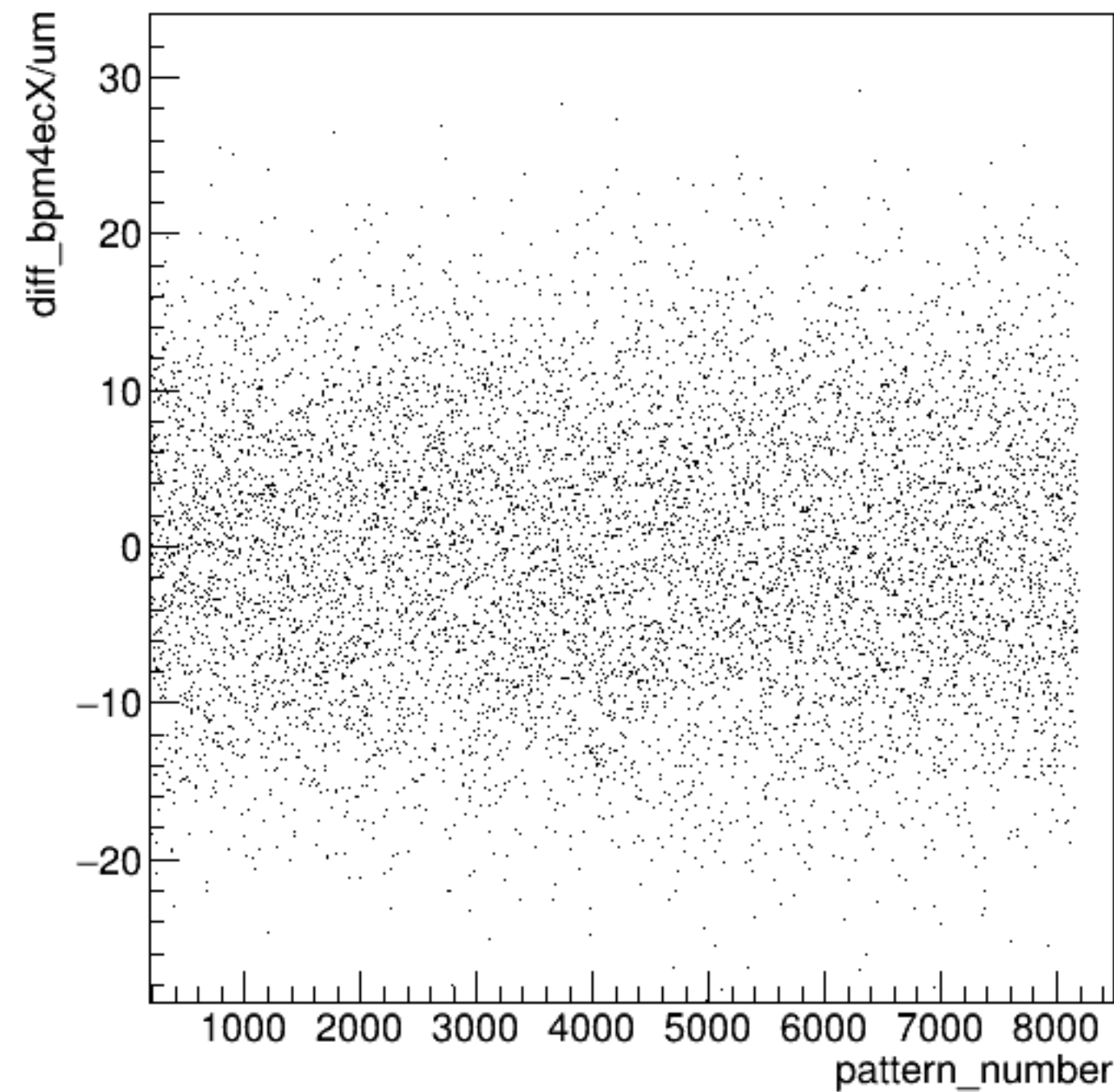
diff_bpm4ecX/um:pattern_number {ErrorFlag==0}
