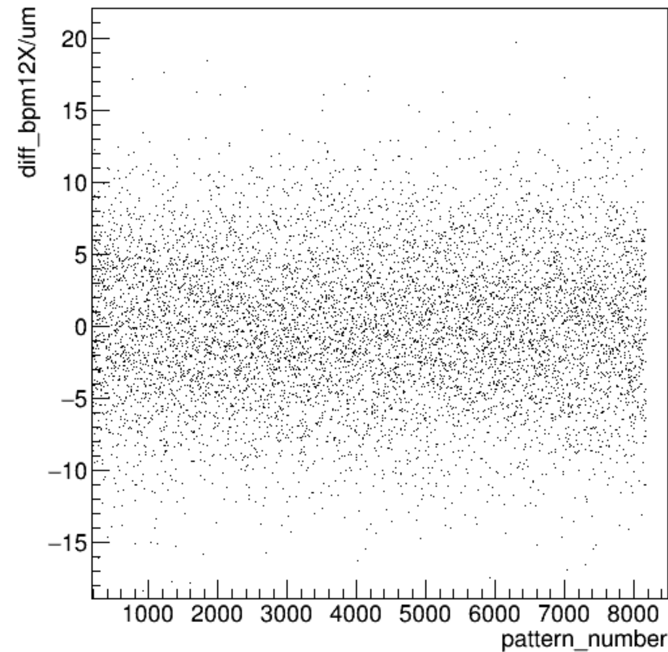
diff_bpm12X/um:pattern_number {ErrorFlag==0}
