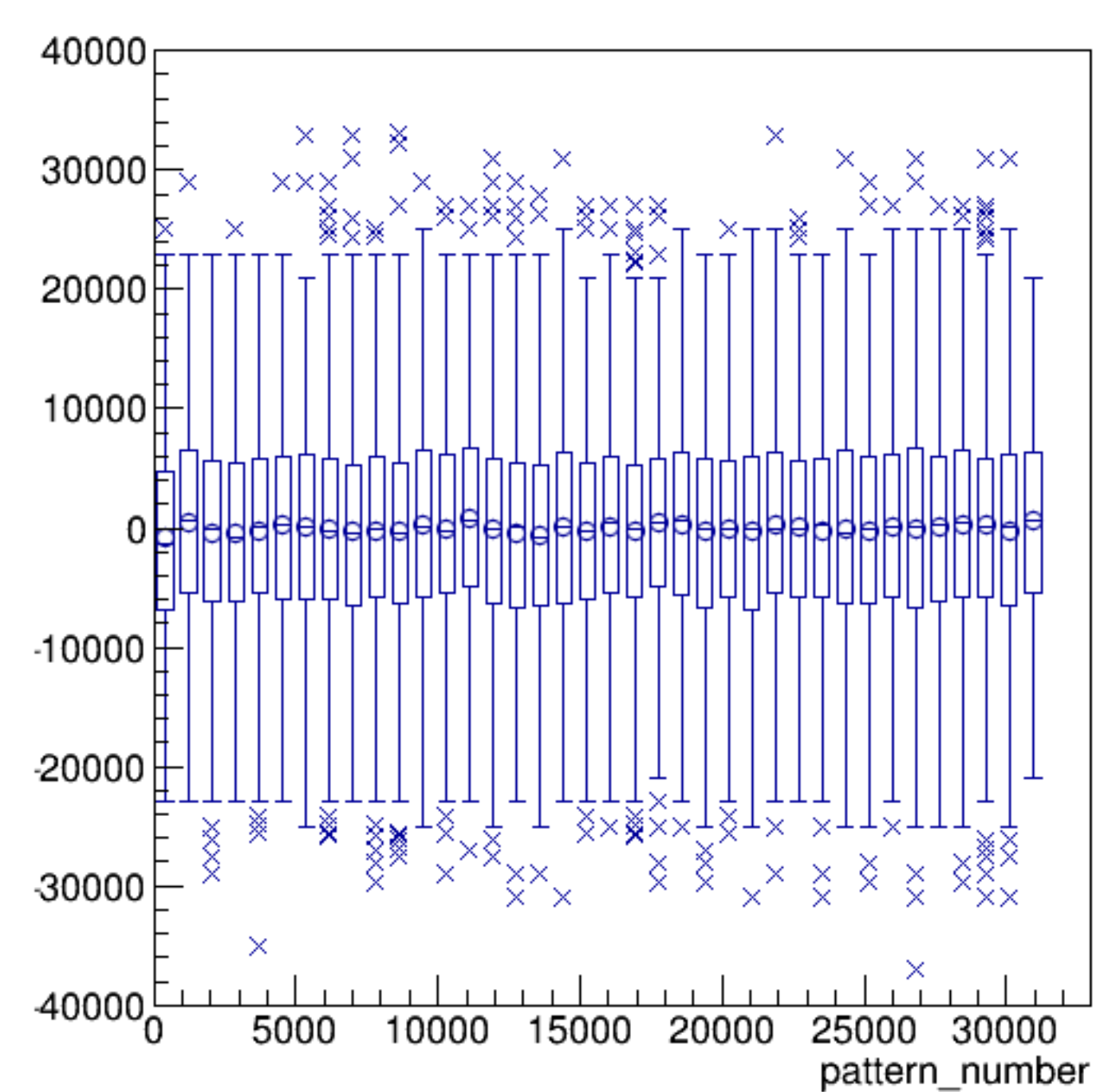
asym_atl1/ppm:pattern_number {ErrorFlag==0}
