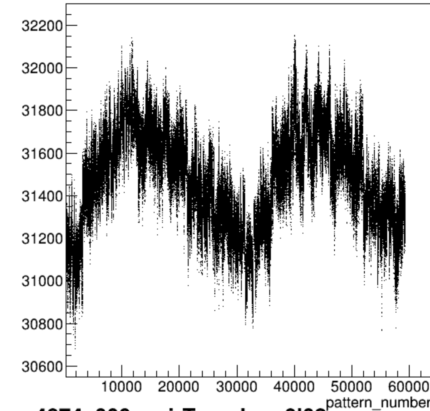
yield_bcm0l02:pattern_number {ErrorFlag==0}
