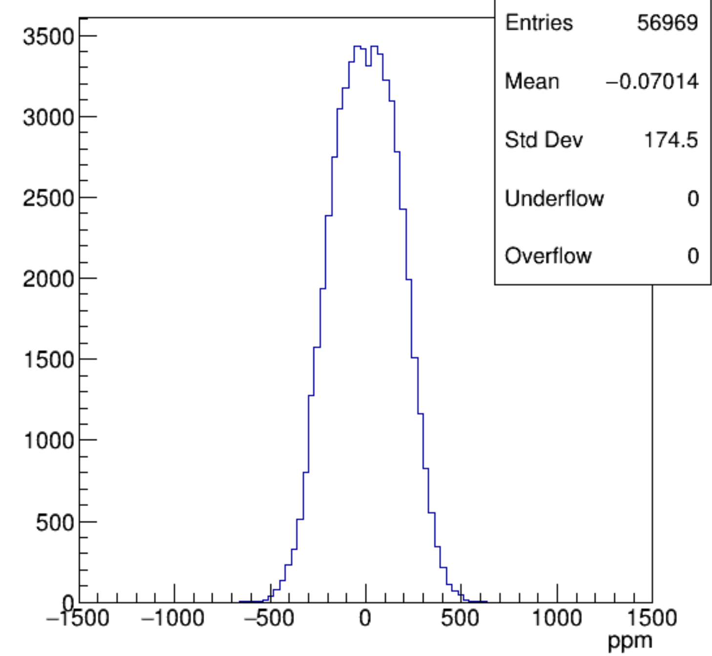
asym_bcm_dg_ds
