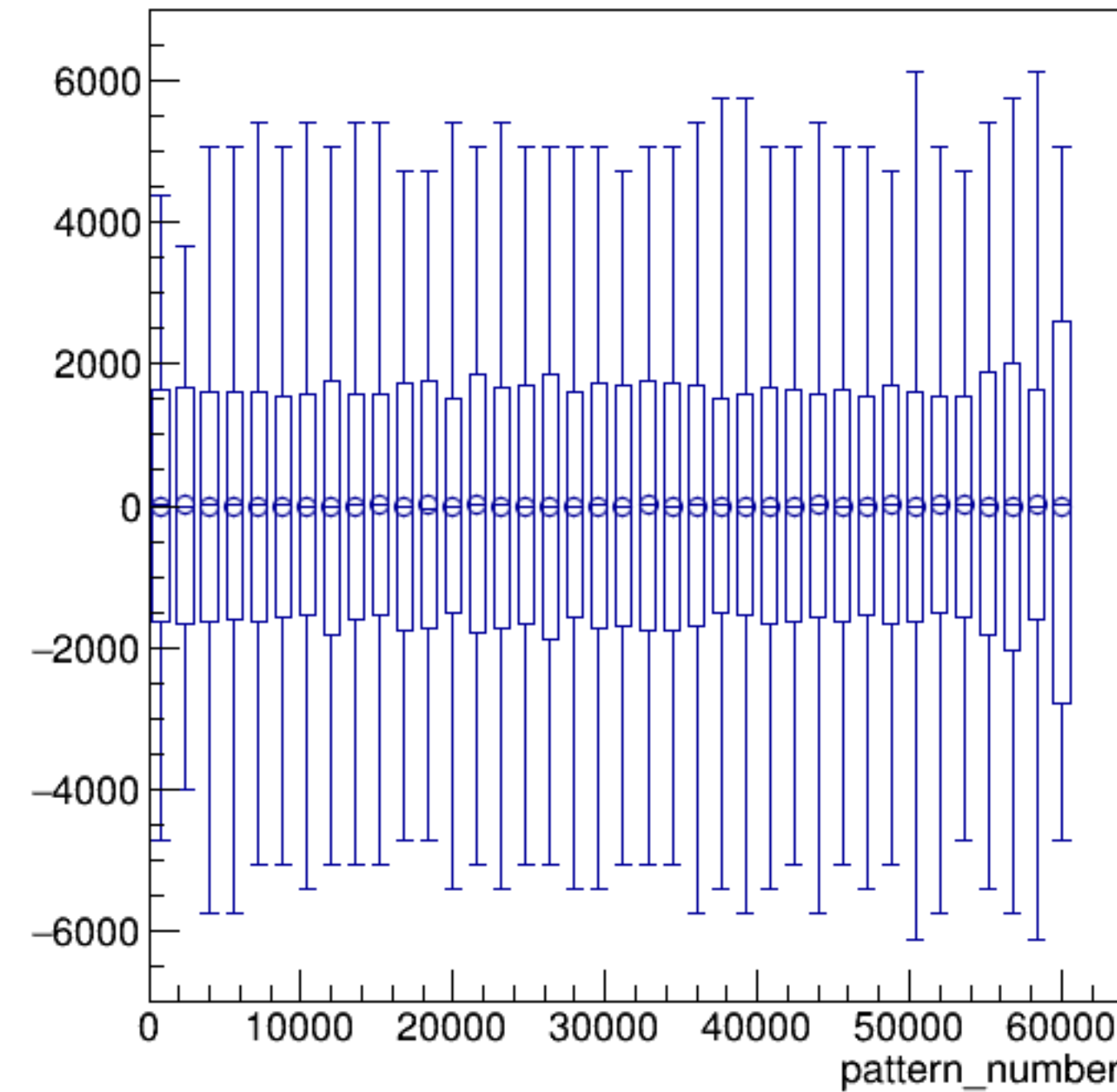
asym_bcm0l02/ppm:pattern_number {ErrorFlag==0}
