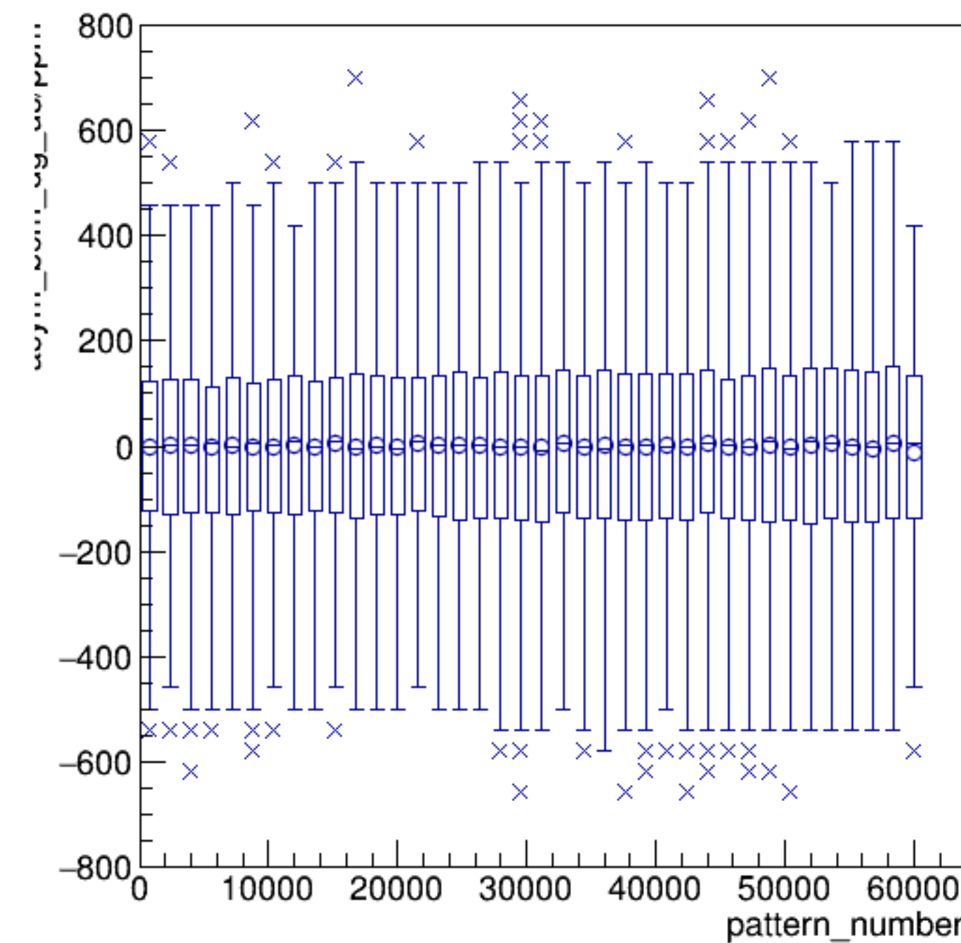
asym_bcm_dg_us/ppm:pattern_number {ErrorFlag==0}
