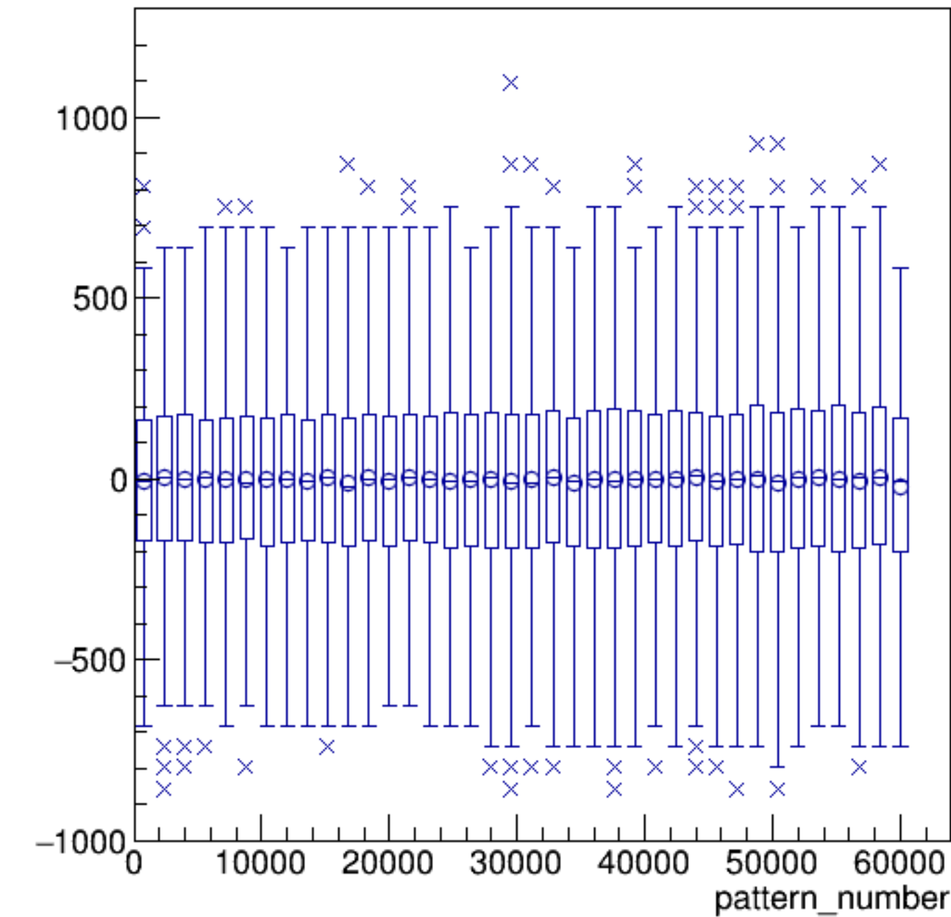
asym_bcm0l02/ppm:pattern_number {ErrorFlag==0}
