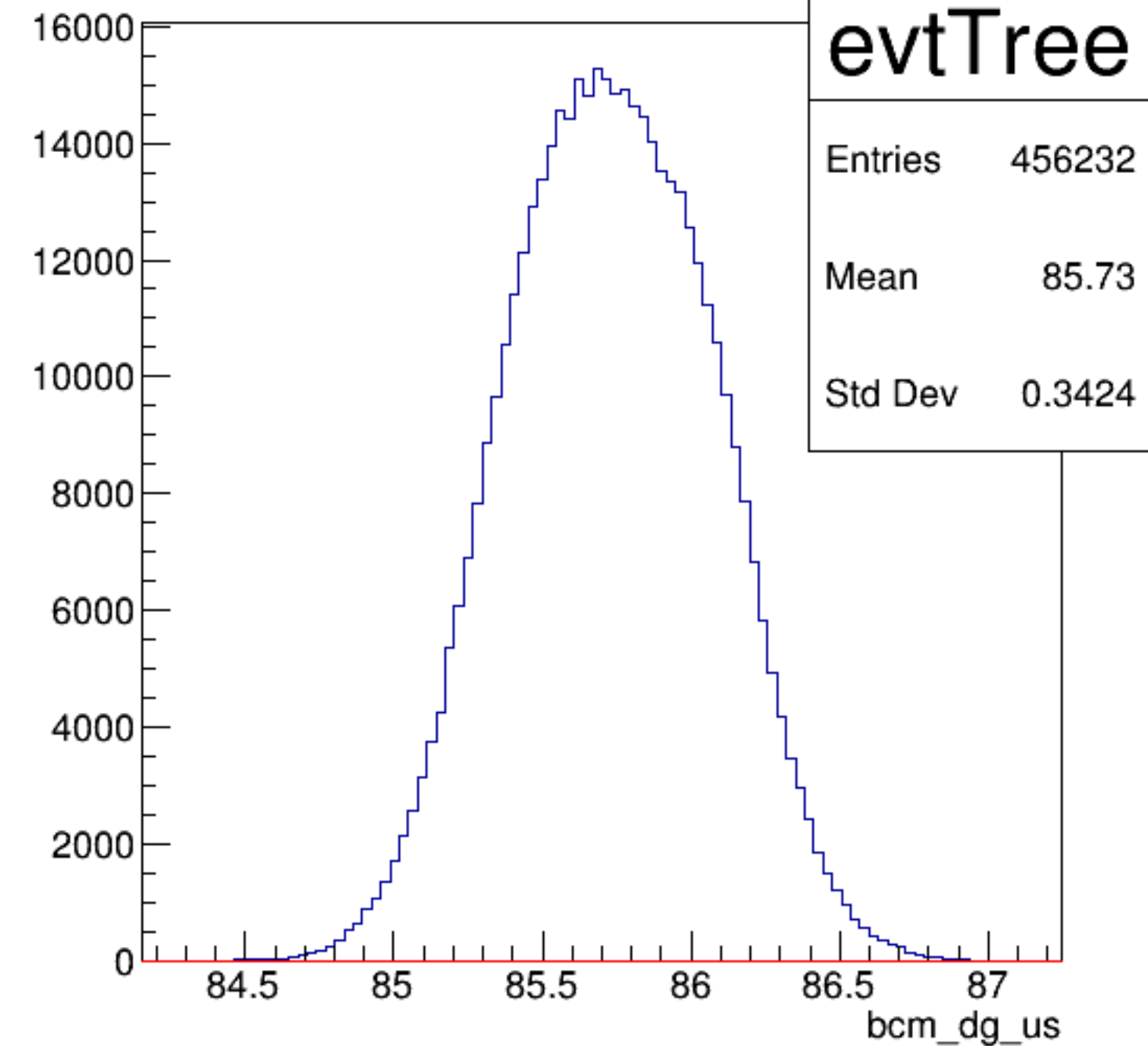
bcm_dg_us {ErrorFlag==0}
