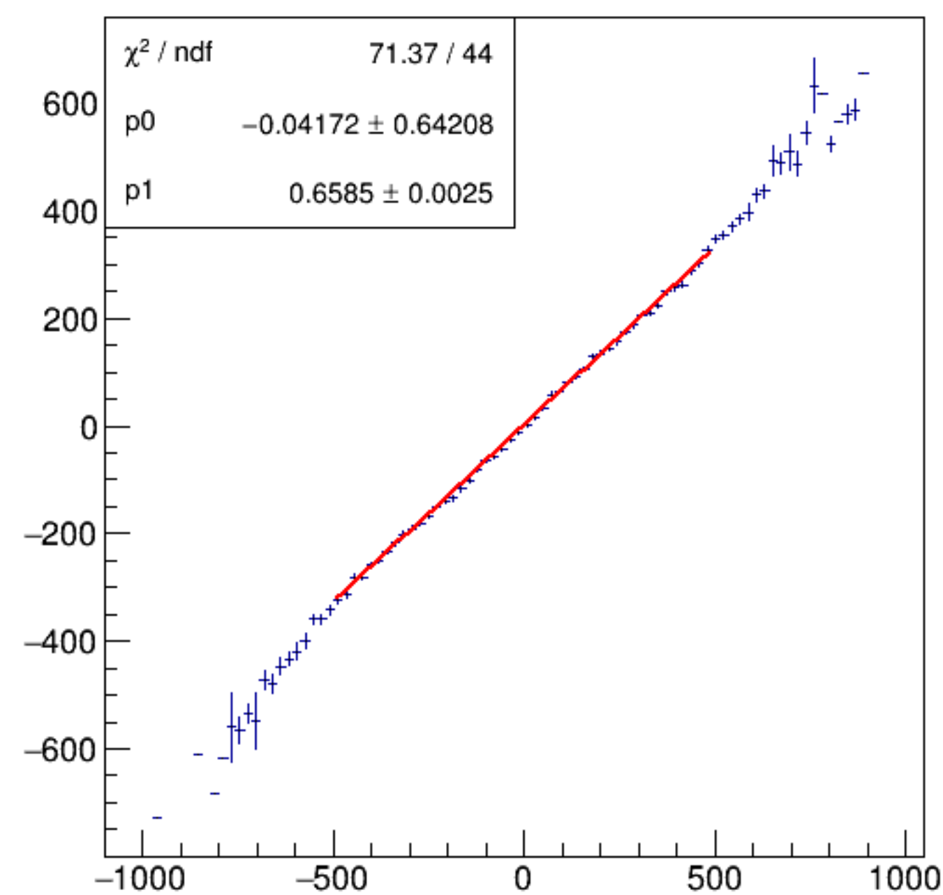
asym_bpm4eWS/ppm:Aq/ppm {ErrorFlag==0}
