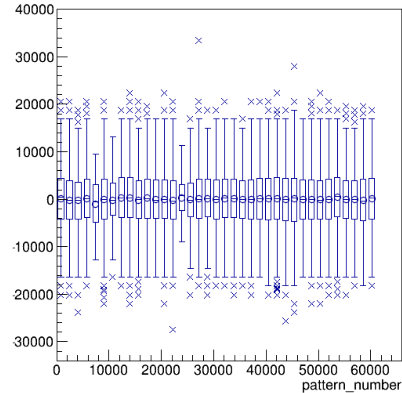
asym_sam3/ppm:pattern_number {ErrorFlag==0}
