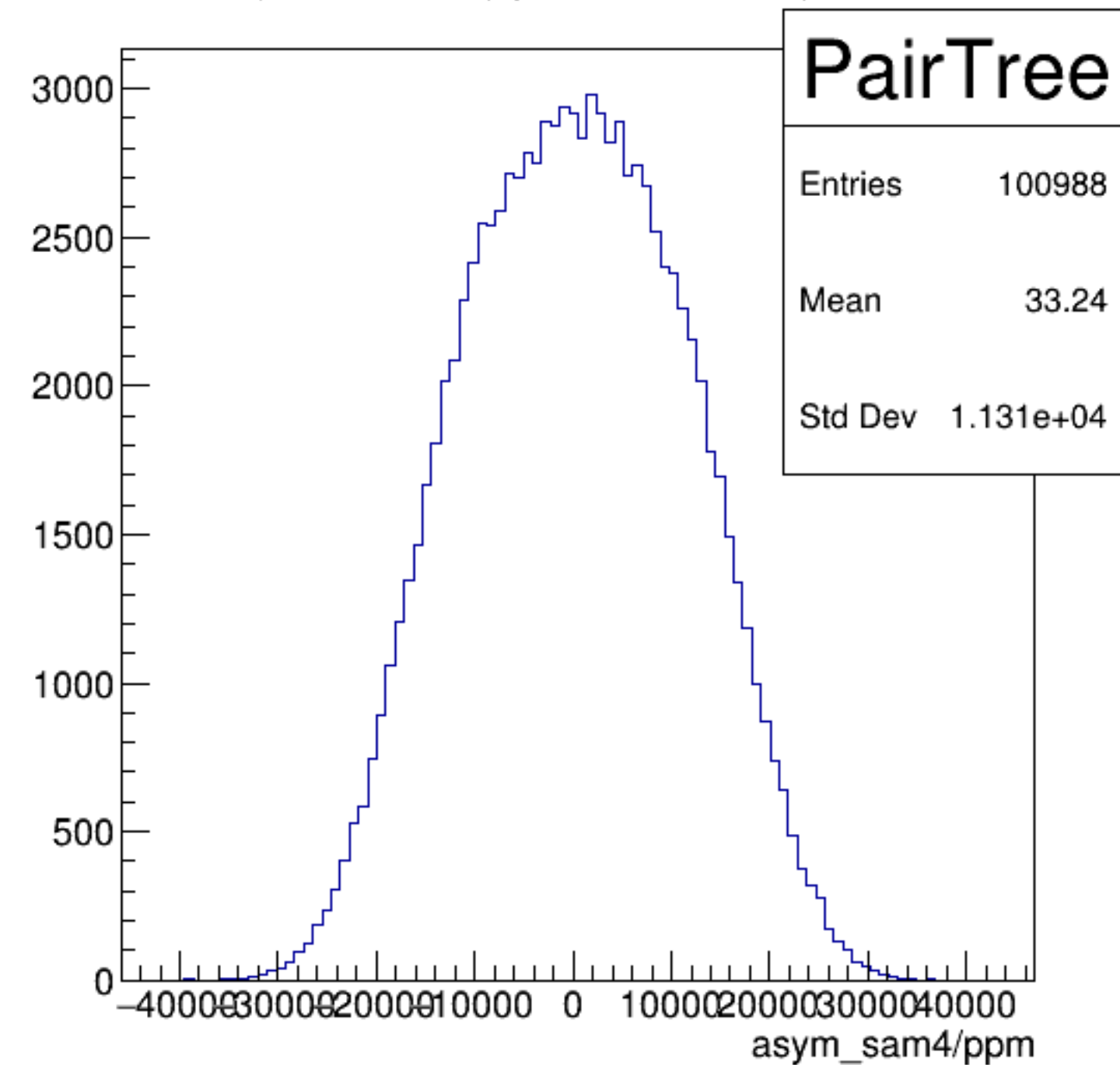
asym_sam4/ppm {ErrorFlag==0}
