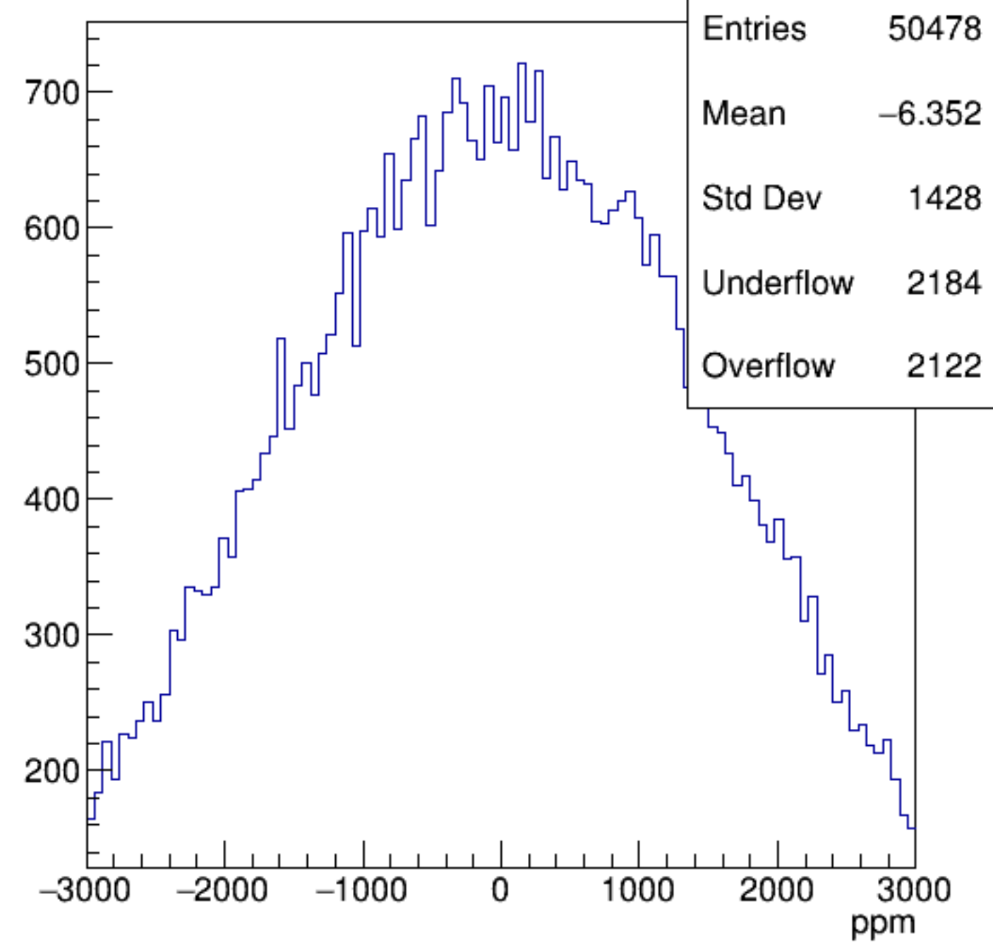
asym_sam8
