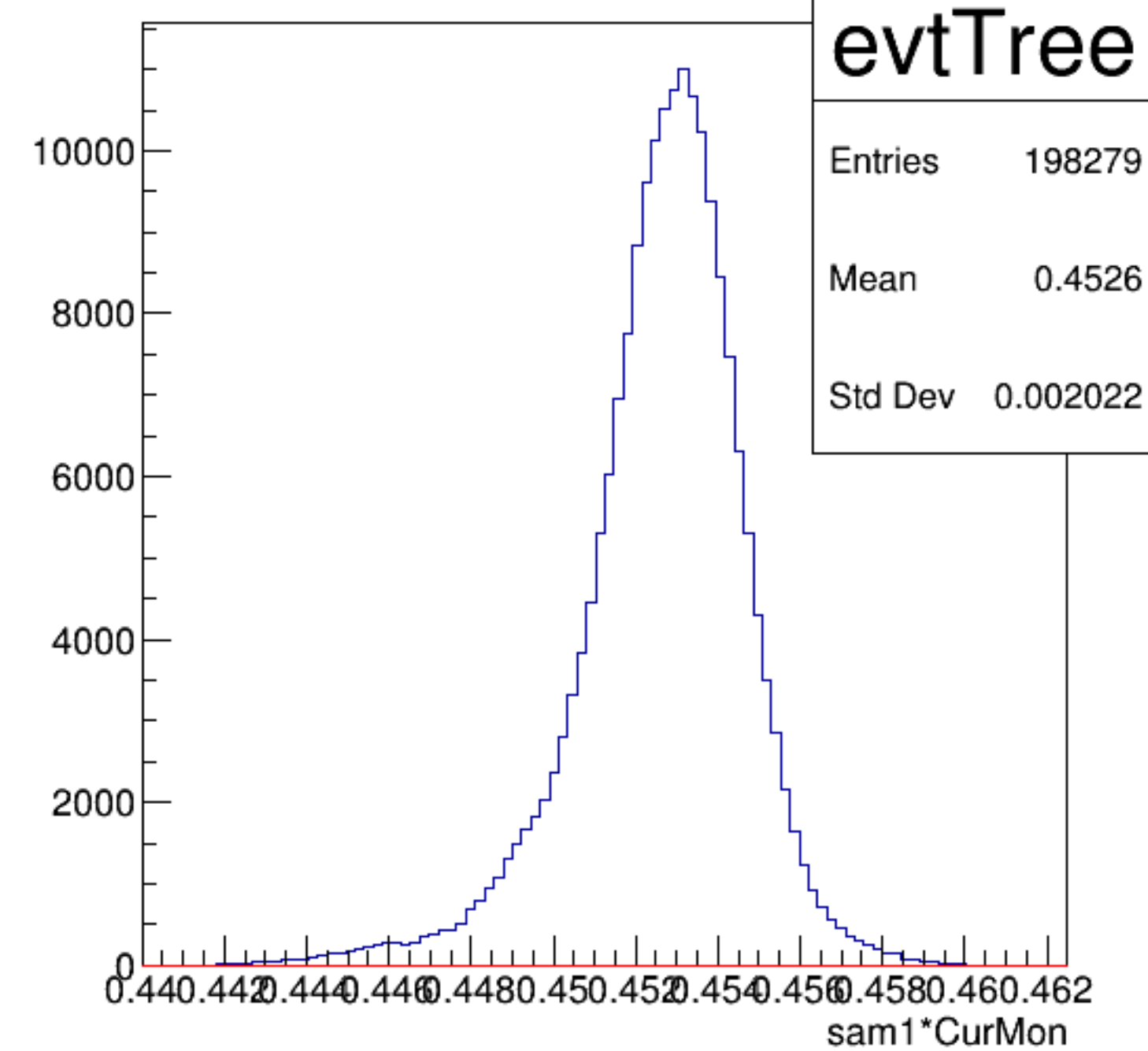
sam1*CurMon {ErrorFlag==0}
