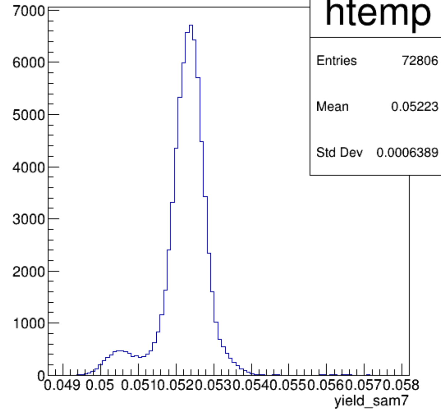
yield_sam7 {ErrorFlag==0}
