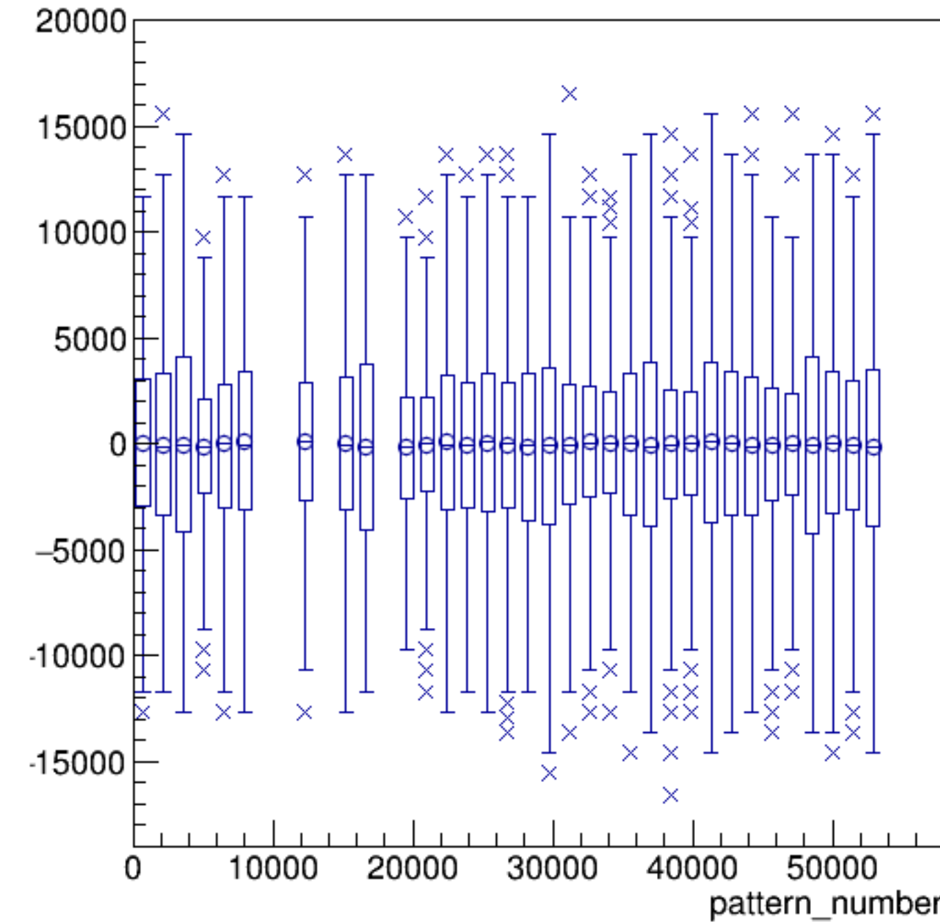
asym_sam7/ppm:pattern_number {ErrorFlag==0}
