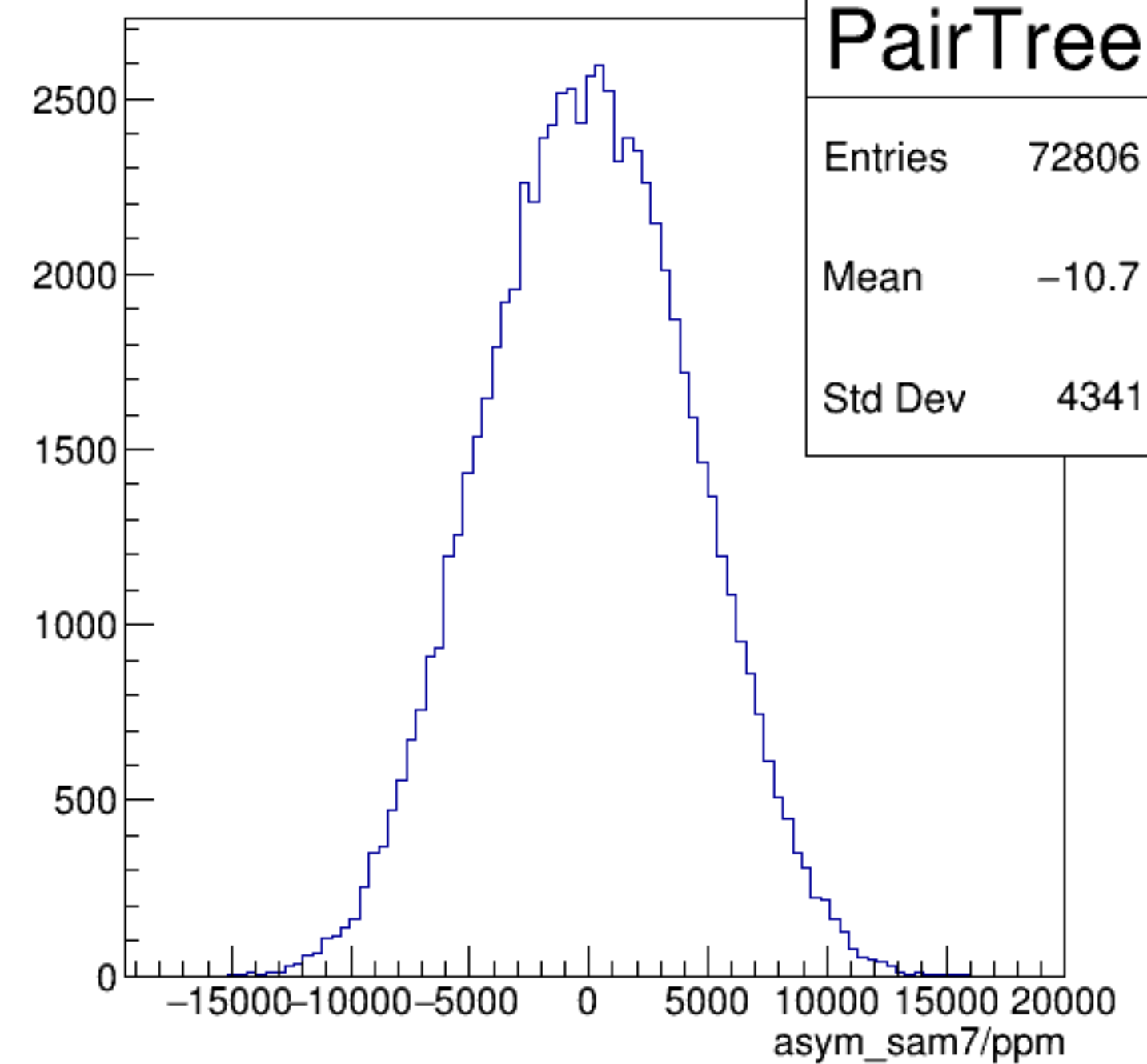
asym_sam7/ppm {ErrorFlag==0}
