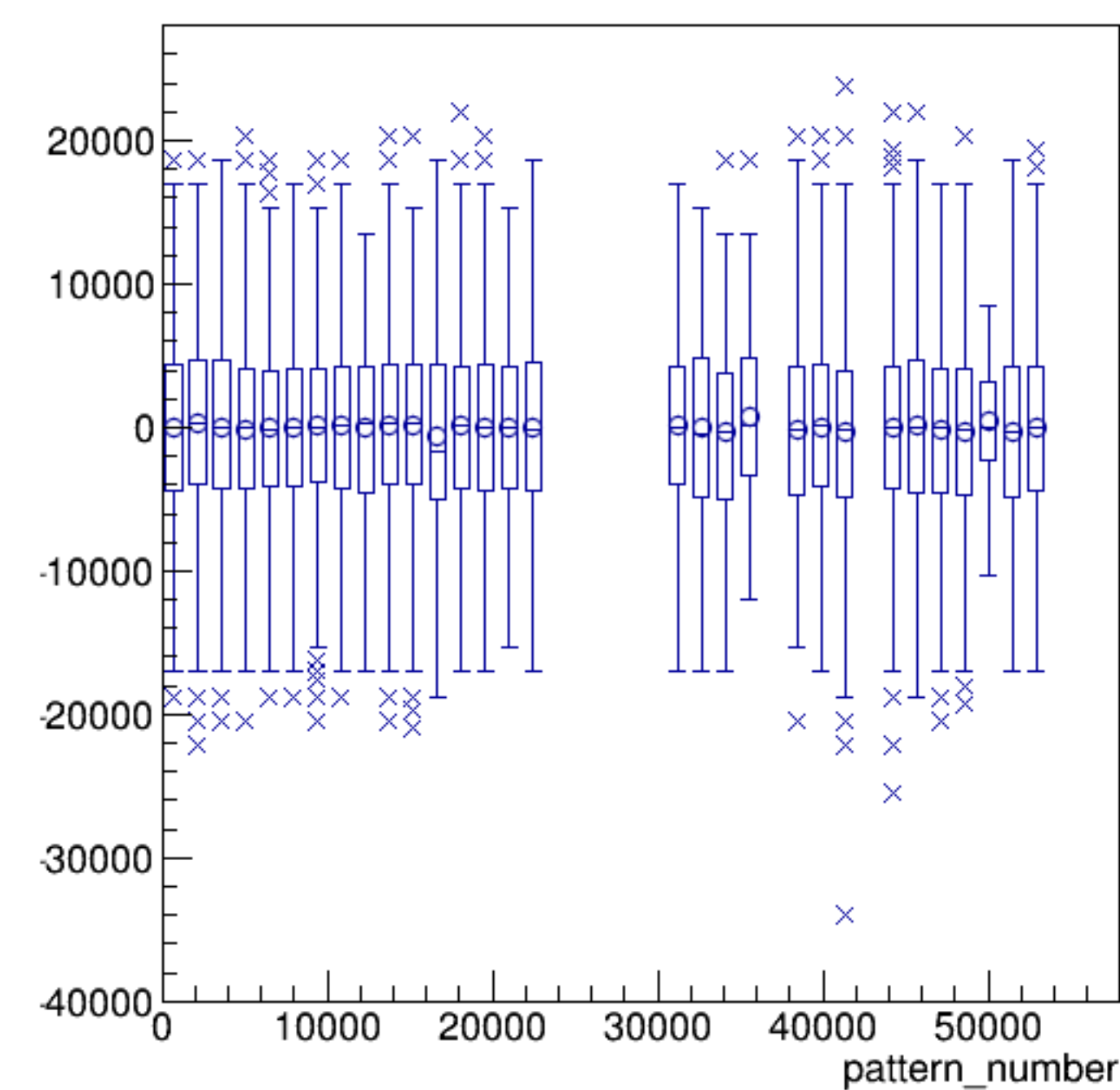
asym_sam2/ppm:pattern_number {ErrorFlag==0}
