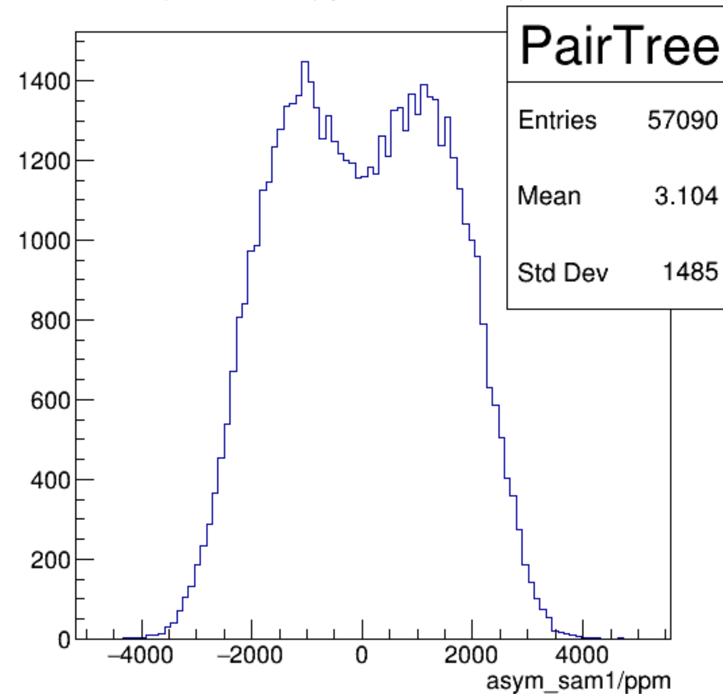
asym_sam1/ppm {ErrorFlag==0}
