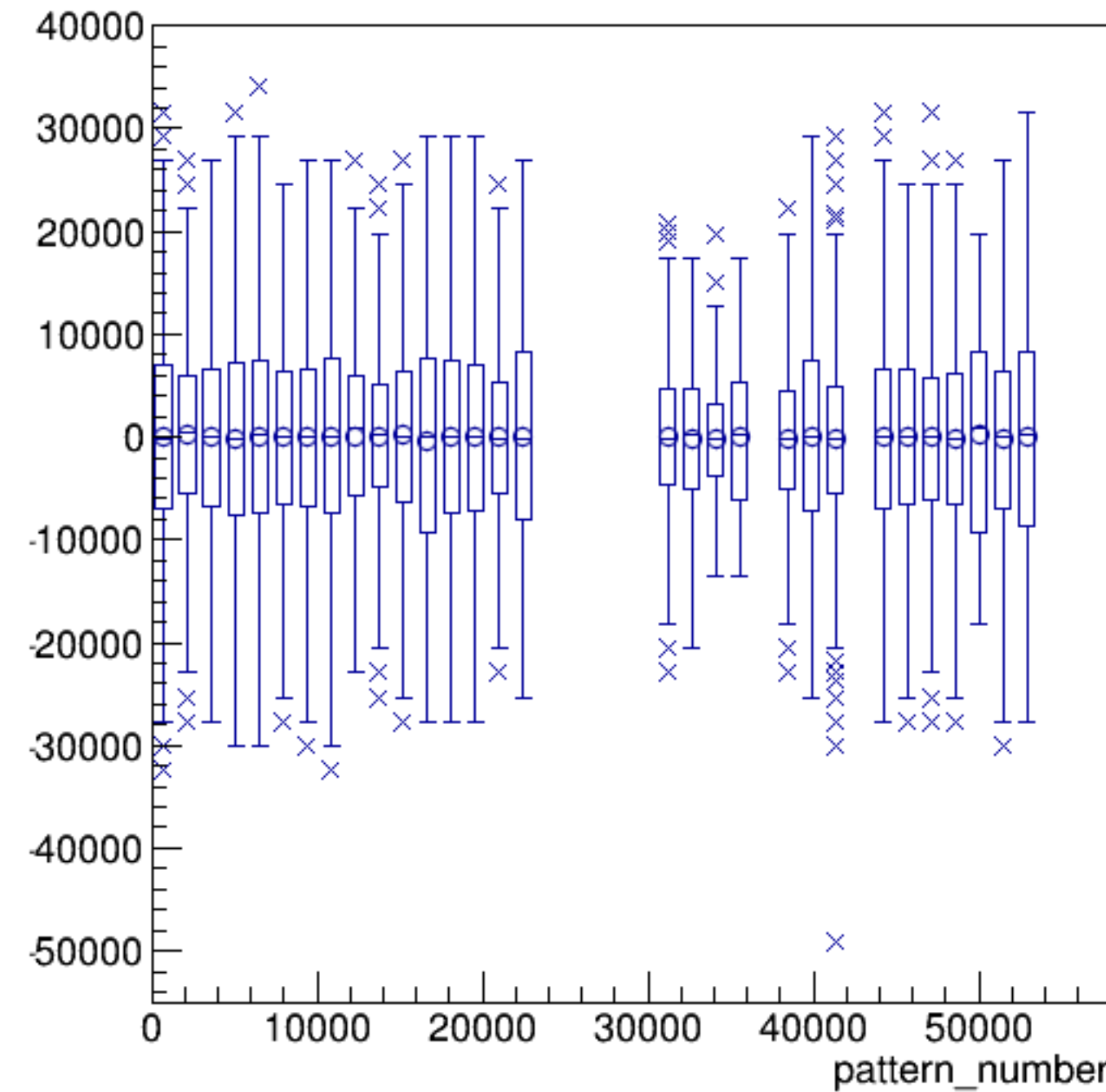
asym_sam3/ppm:pattern_number {ErrorFlag==0}
