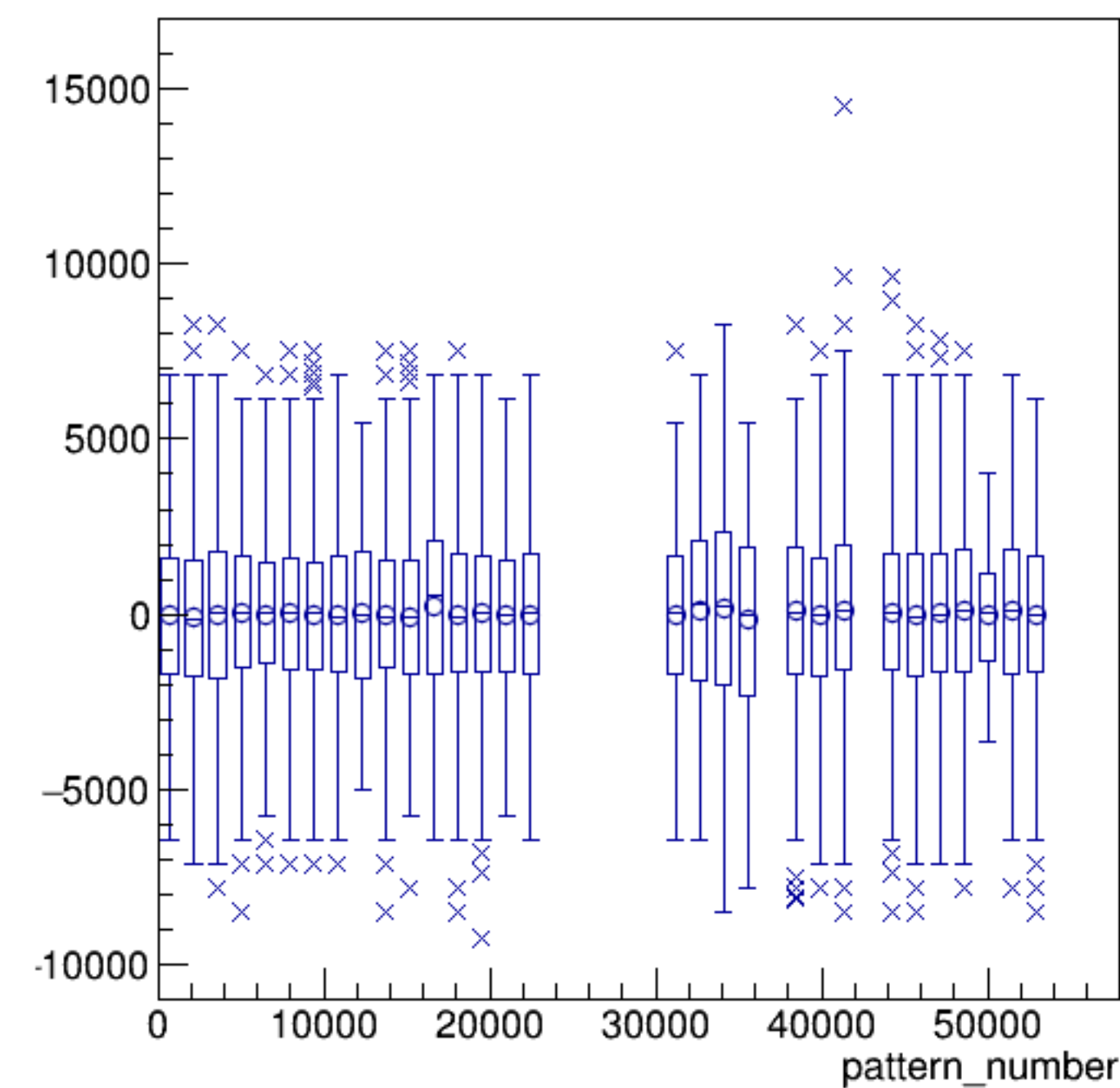
asym_sam7/ppm:pattern_number {ErrorFlag==0}
