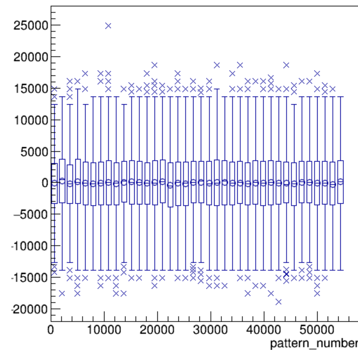
asym_sam4/ppm:pattern_number {ErrorFlag==0}
