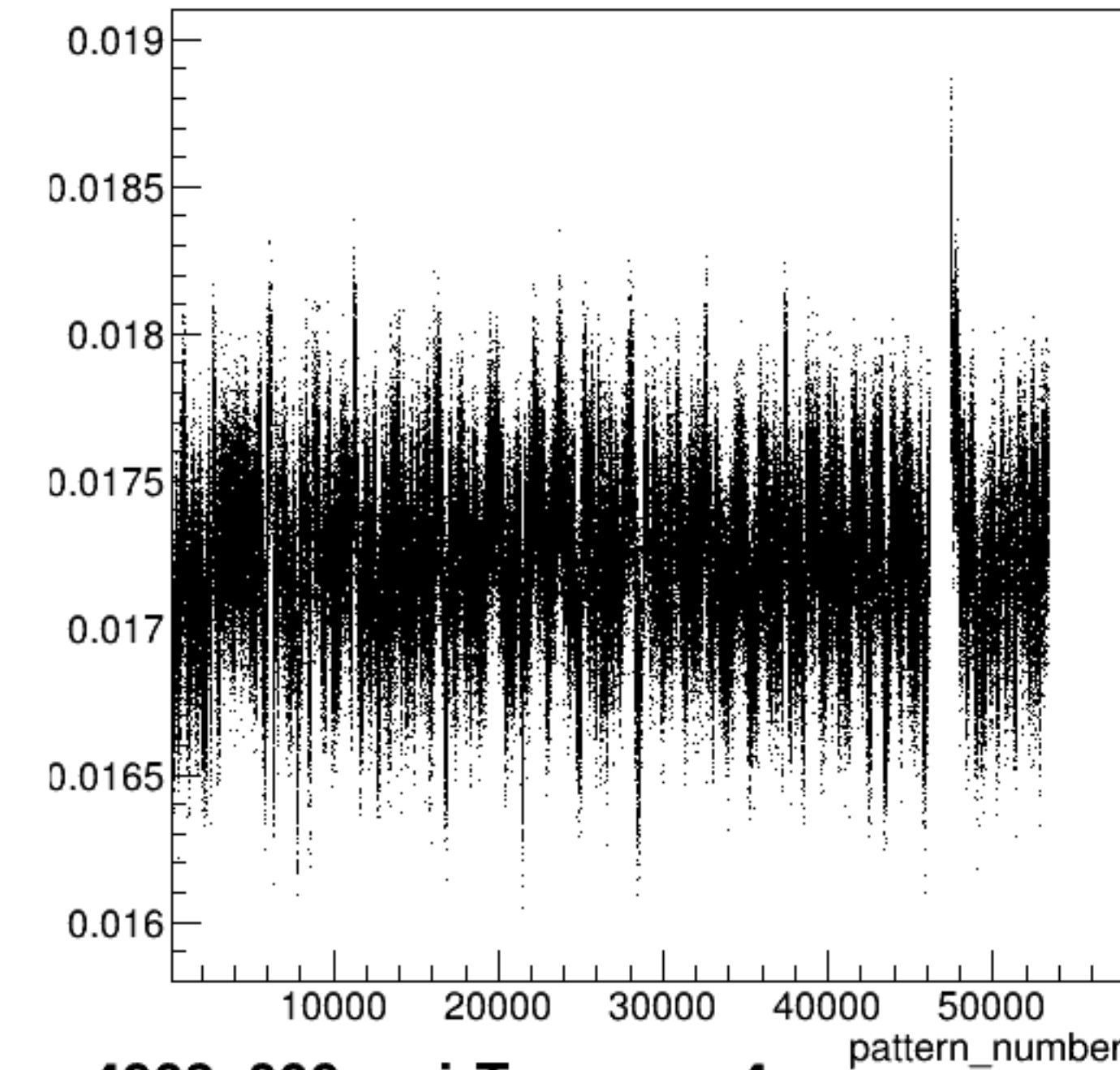
yield_sam4:pattern_number {ErrorFlag==0}
