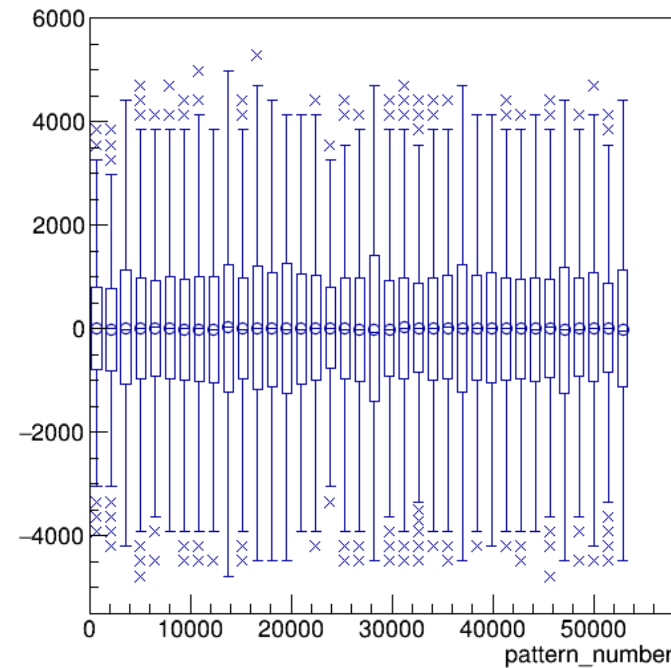
asym_sam1/ppm:pattern_number {ErrorFlag==0}
