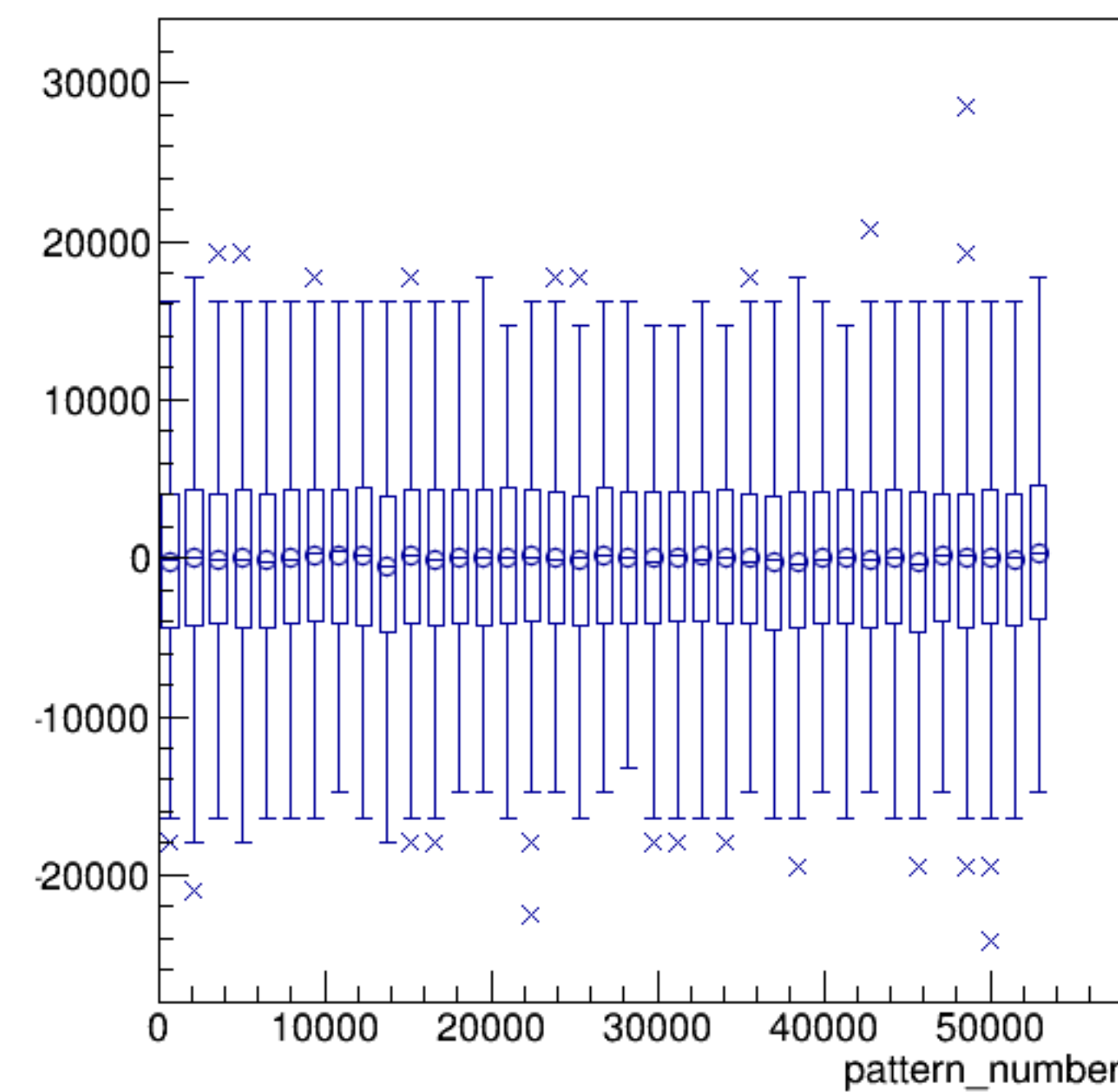
asym_sam3/ppm:pattern_number {ErrorFlag==0}
