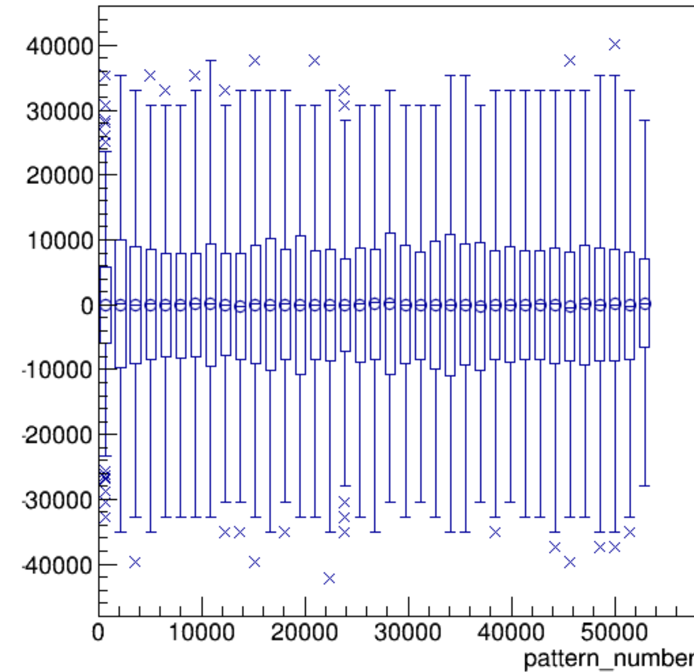
asym_sam4/ppm:pattern_number {ErrorFlag==0}
