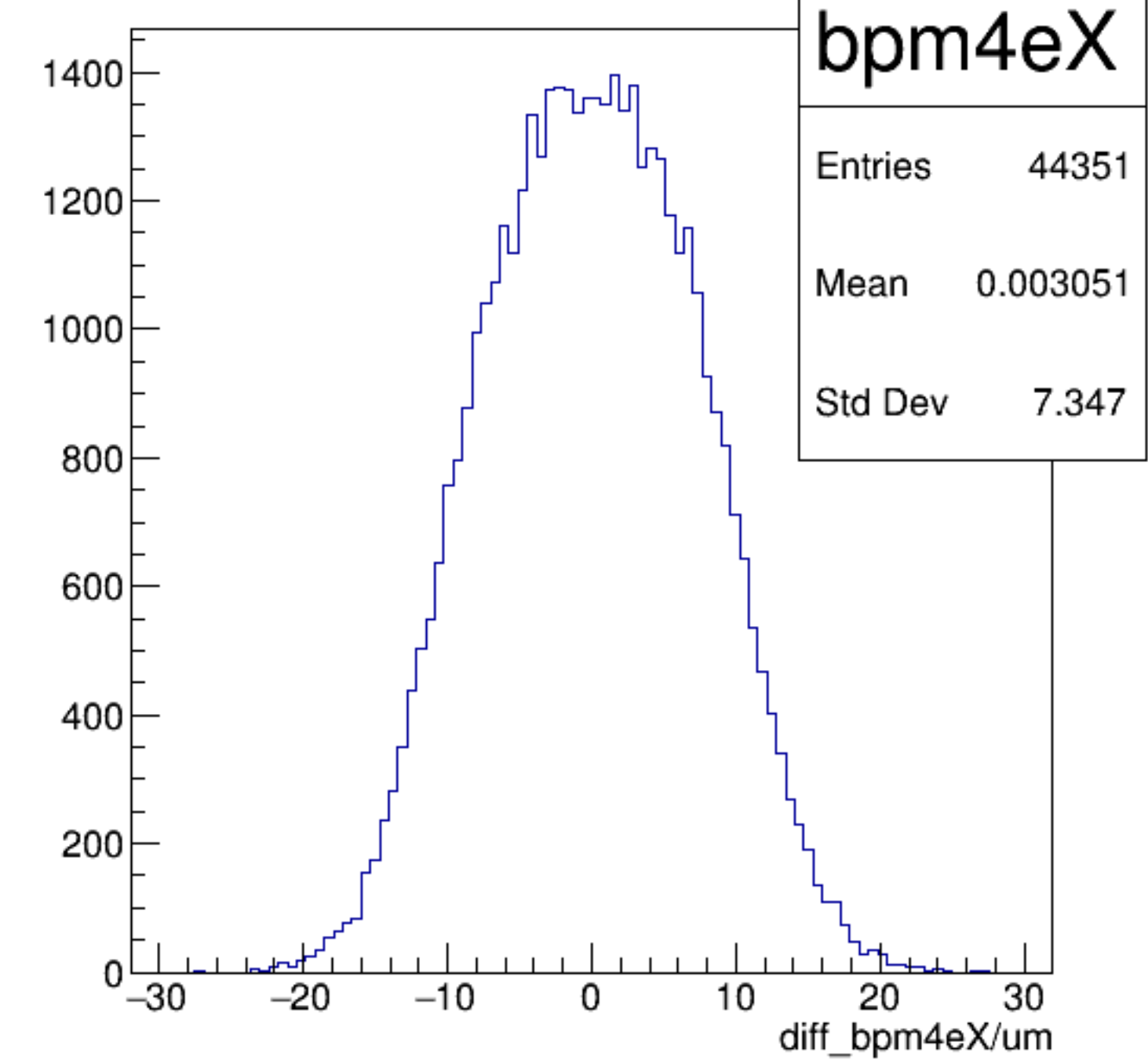
diff_bpm4eX/um {ErrorFlag==0}
