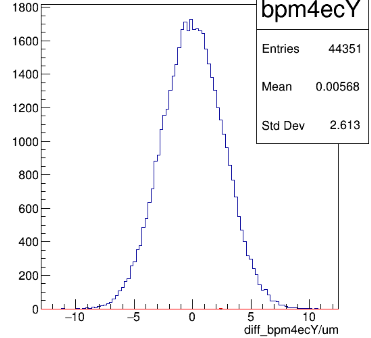
diff_bpm4ecY/um {ErrorFlag==0}
