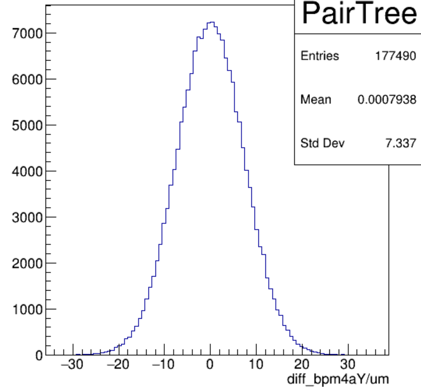
diff_bpm4aY/um {ErrorFlag==0}
