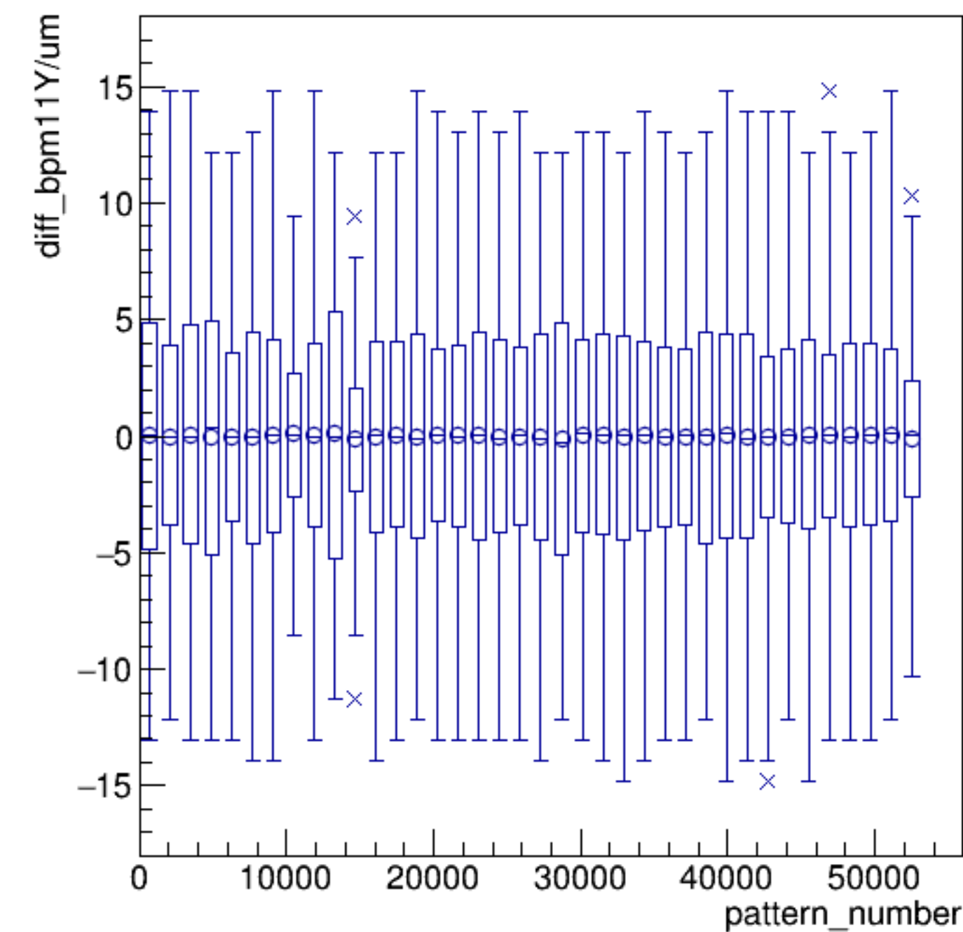
diff_bpm11Y/um:pattern_number {ErrorFlag==0}
