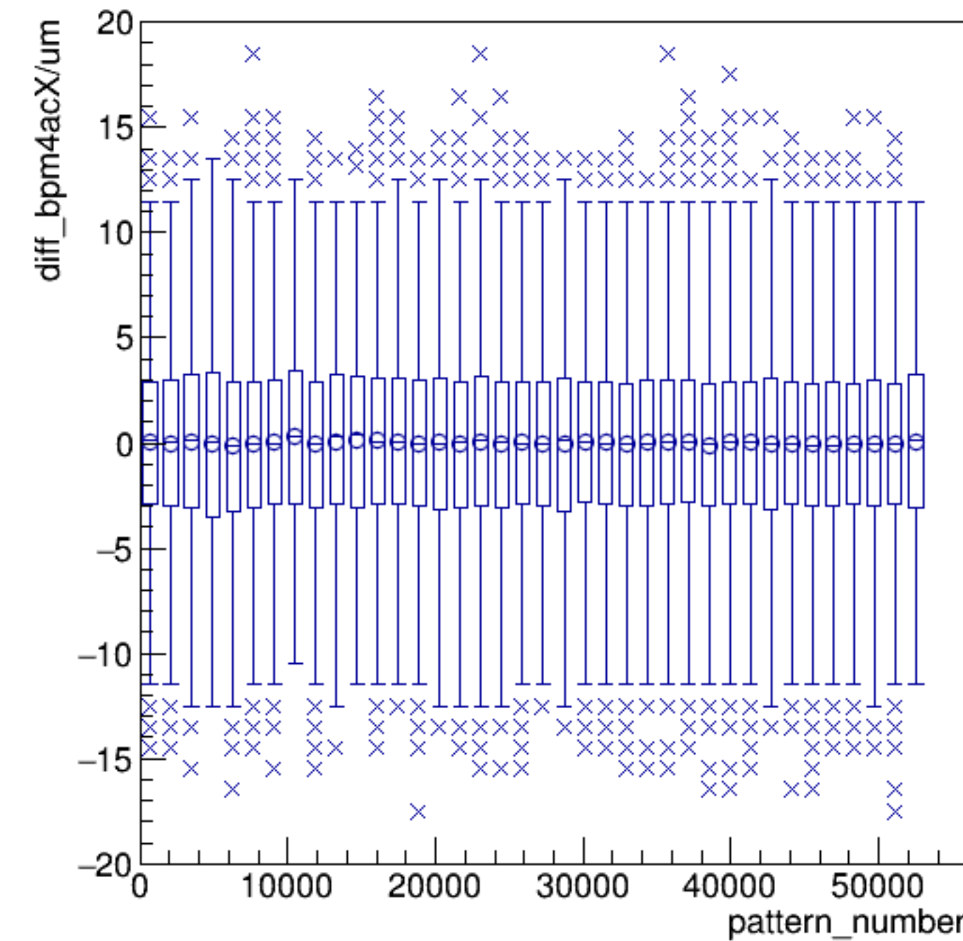
diff_bpm4acX/um:pattern_number {ErrorFlag==0}
