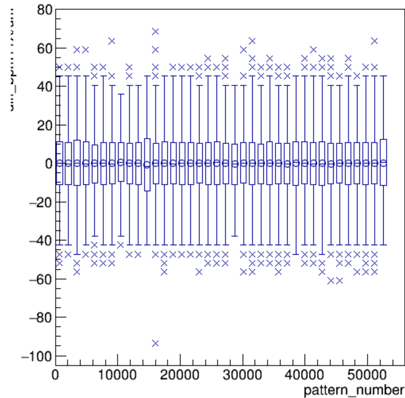
diff_bpm11X/um:pattern_number {ErrorFlag==0}
