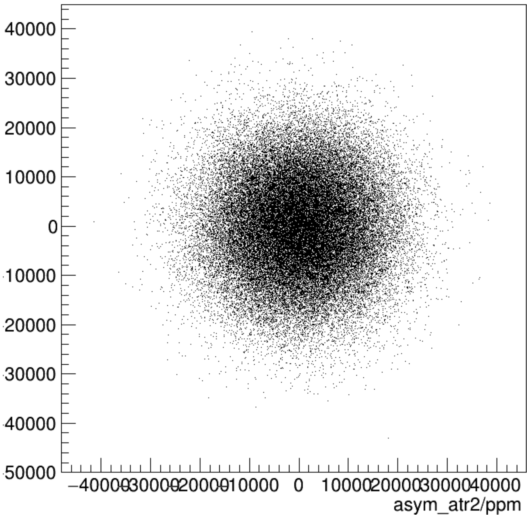
asym_atl2/ppm:asym_atr2/ppm {ok_cut}
