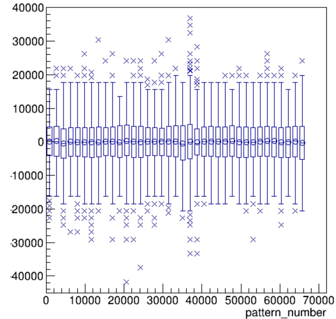
asym_sam3/ppm:pattern_number {ErrorFlag==0}
