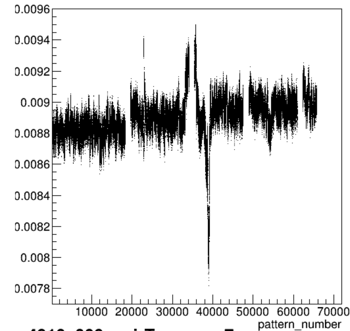
yield_sam7:pattern_number {ErrorFlag==0}
