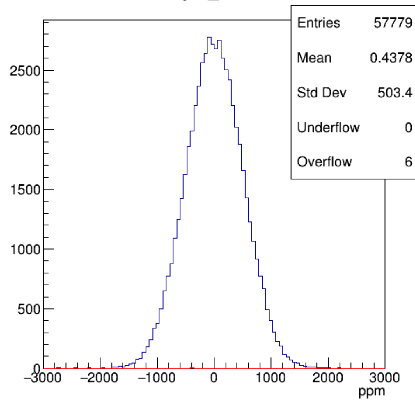
asym_sam5
