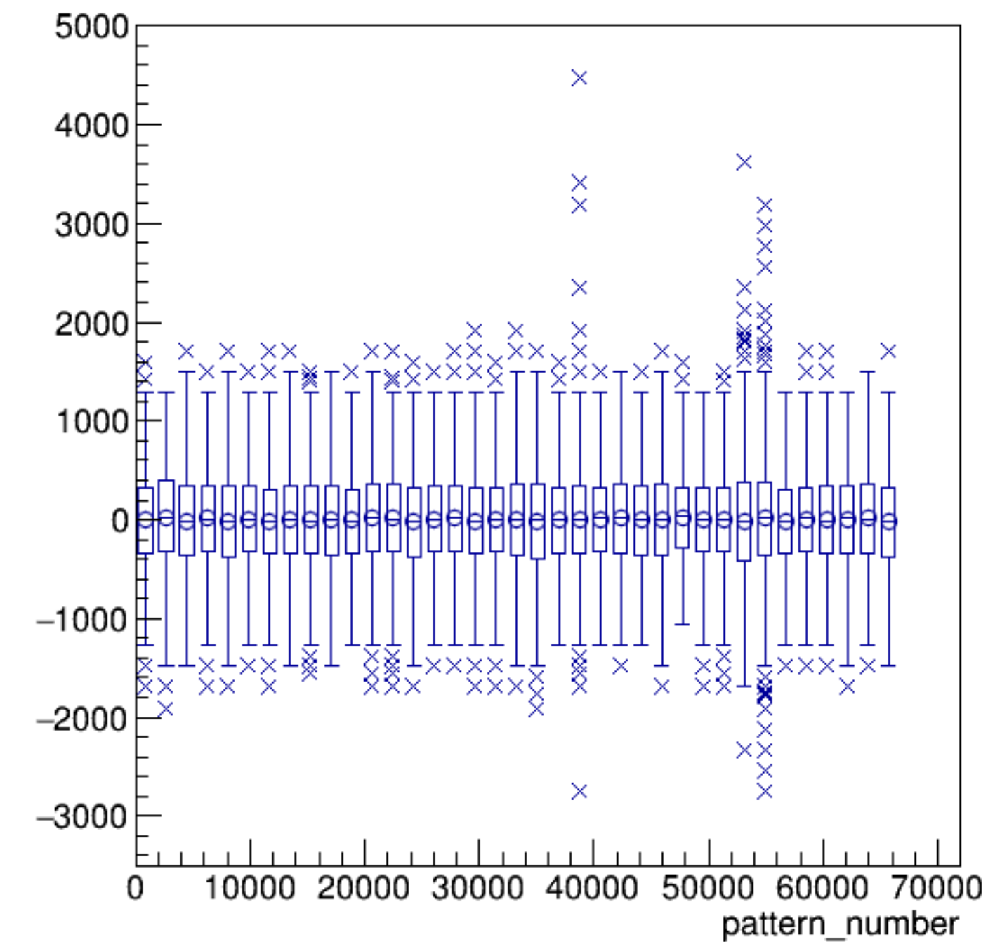
asym_sam5/ppm:pattern_number {ErrorFlag==0}
