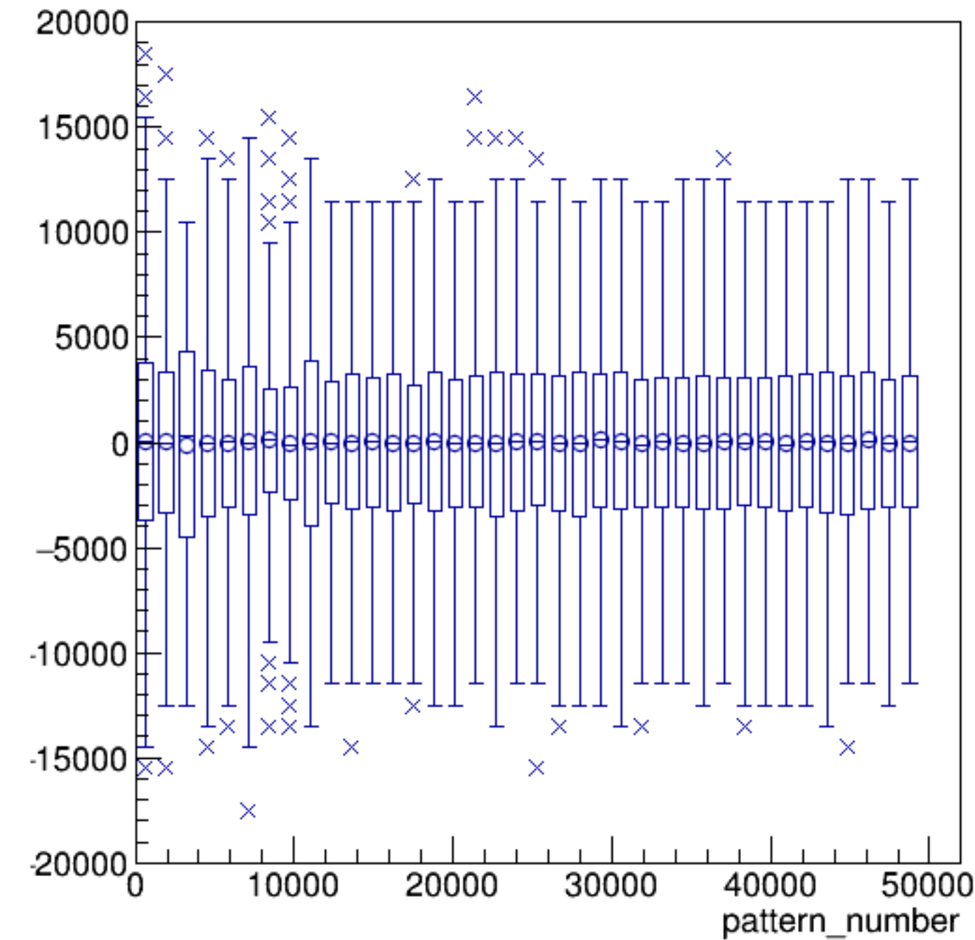
asym_sam8/ppm:pattern_number {ErrorFlag==0}
