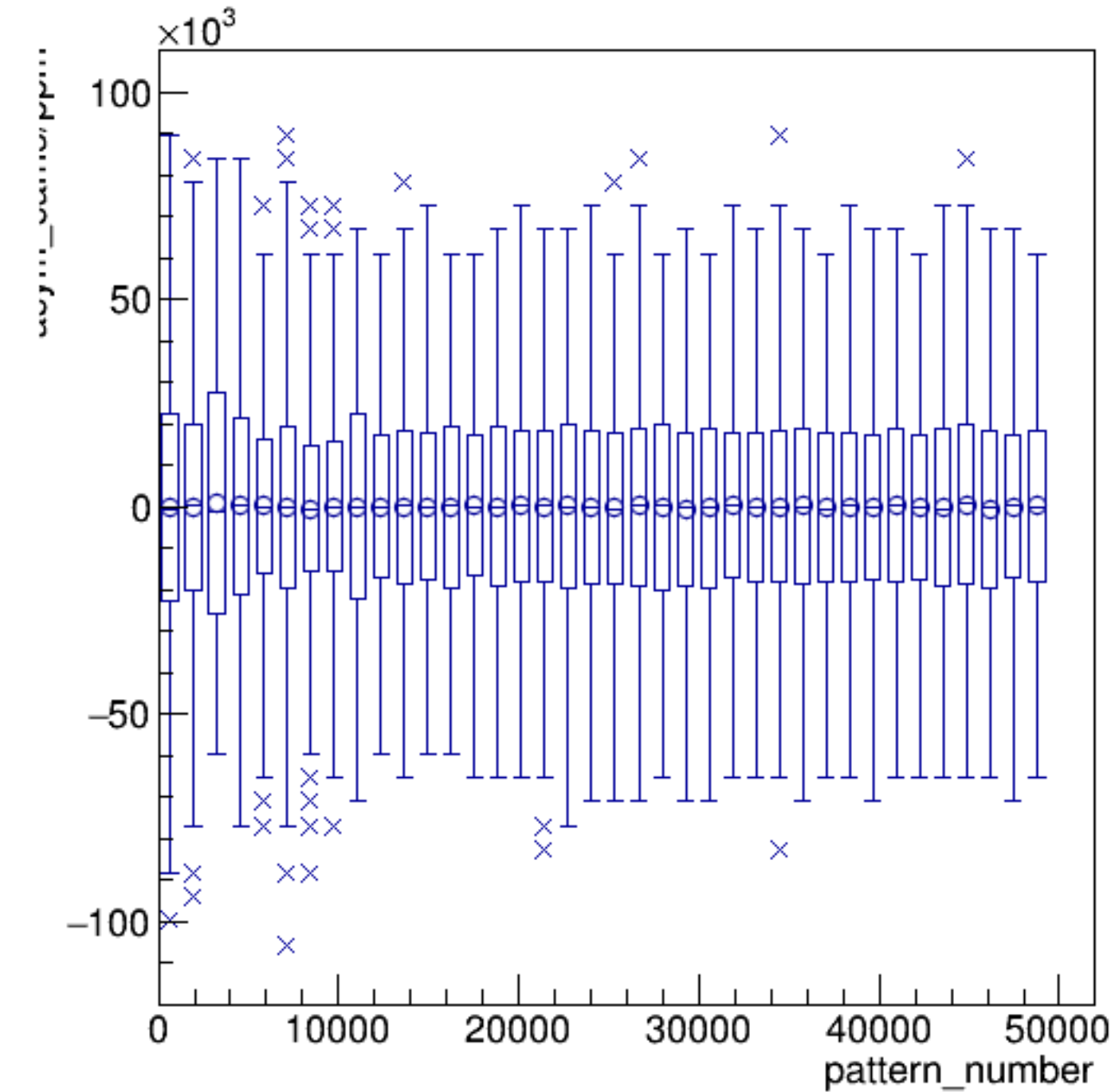
asym_sam3/ppm:pattern_number {ErrorFlag==0}
