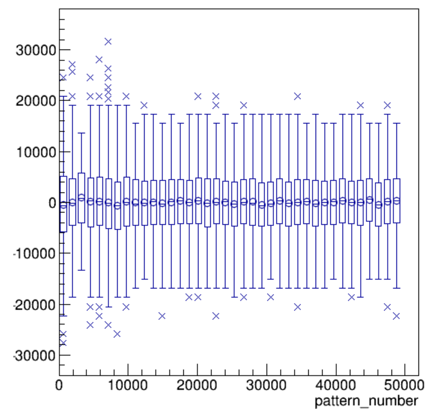
asym_sam3/ppm:pattern_number {ErrorFlag==0}
