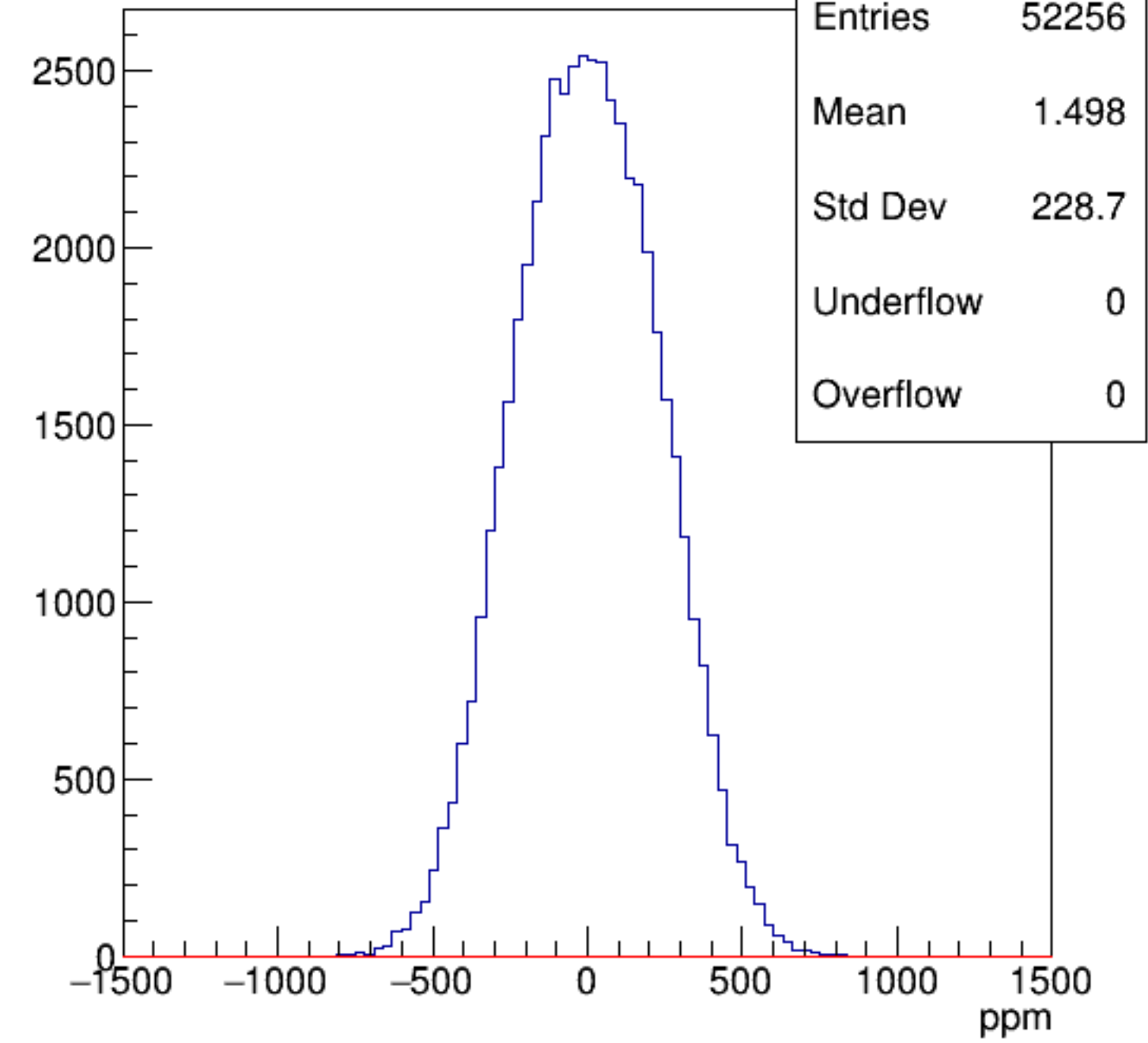
asym_bcm0l02
