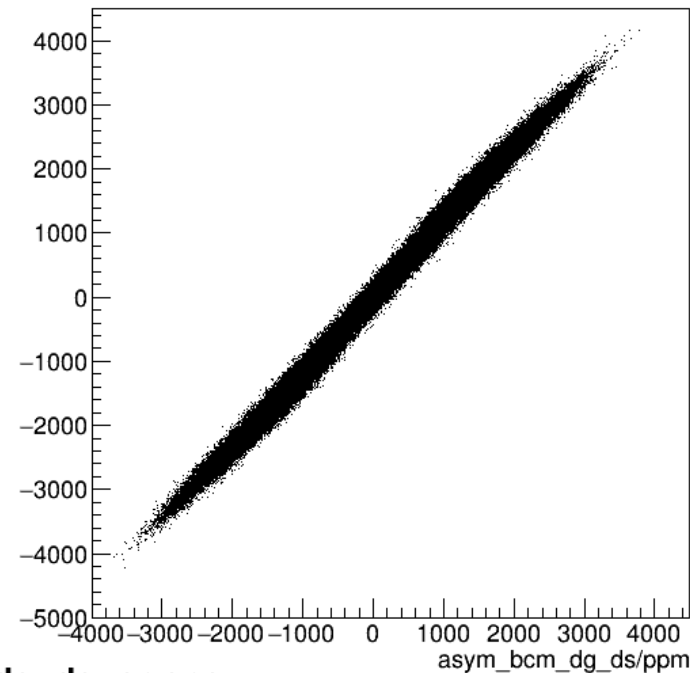
run4916_000_asym_bcm_dg_us_vs_asym_bcm_dg_ds_pr.png
