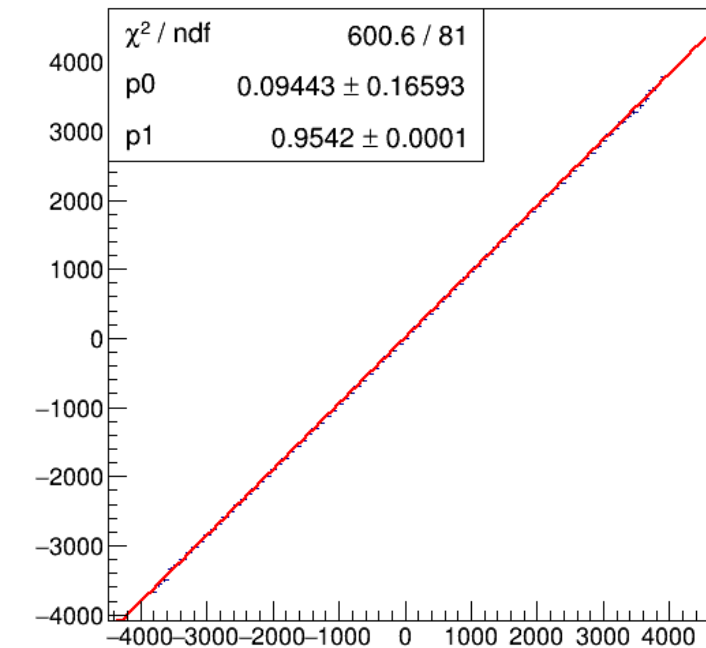
run4916_000_asym_bcm_dg_ds_vs_asym_bcm_an_us_pr.png
