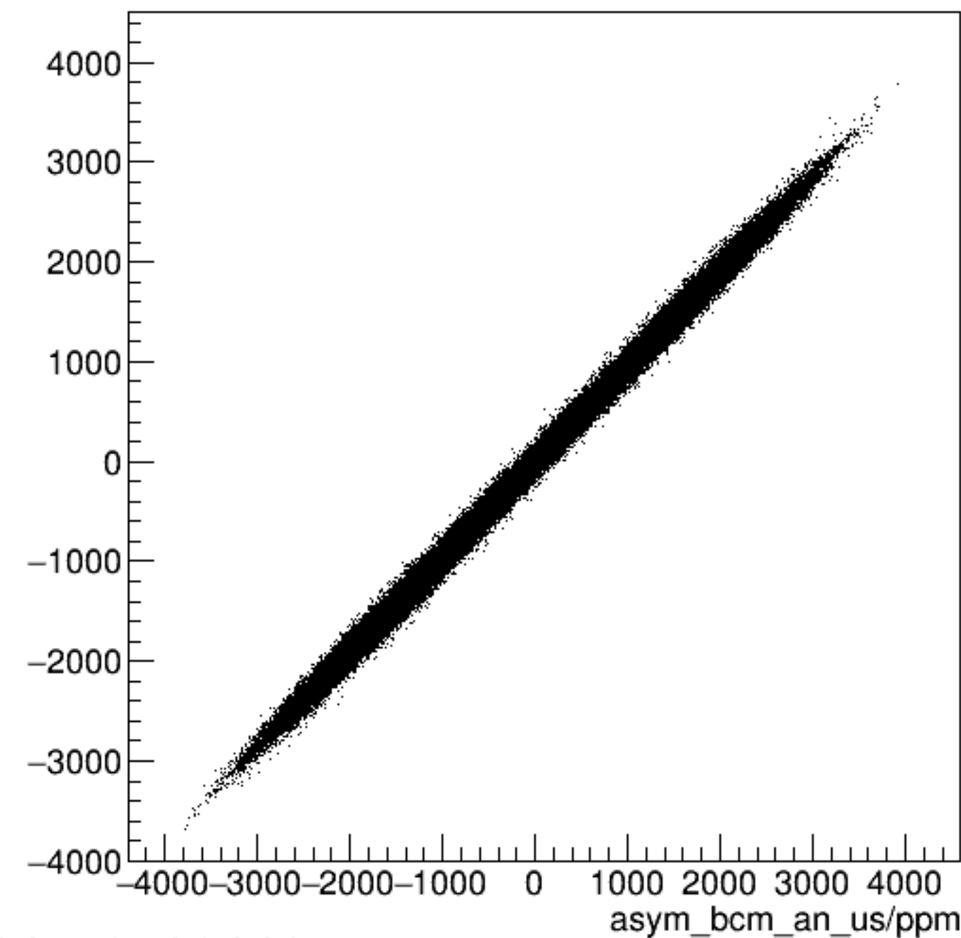
run4916_000_asym_bcm_dg_ds_vs_asym_bcm_an_us_pr.png
