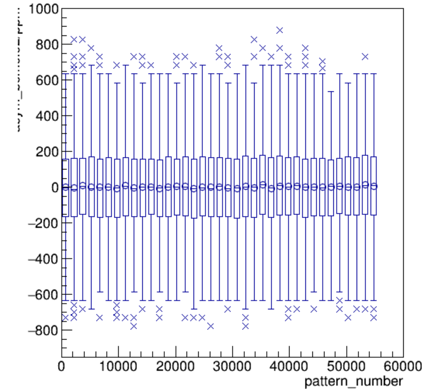
asym_bcm0l02/ppm:pattern_number {ErrorFlag==0}
