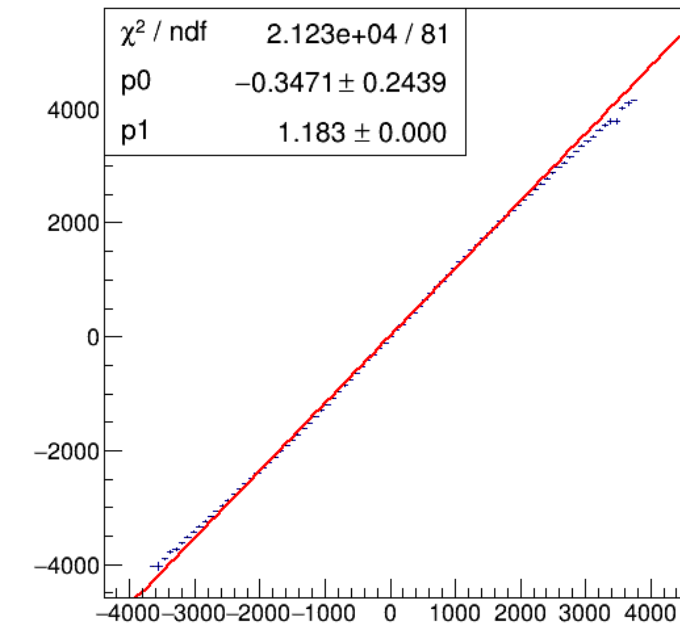
run4916_000_asym_bcm_dg_us_vs_asym_bcm_dg_ds_pr.png
