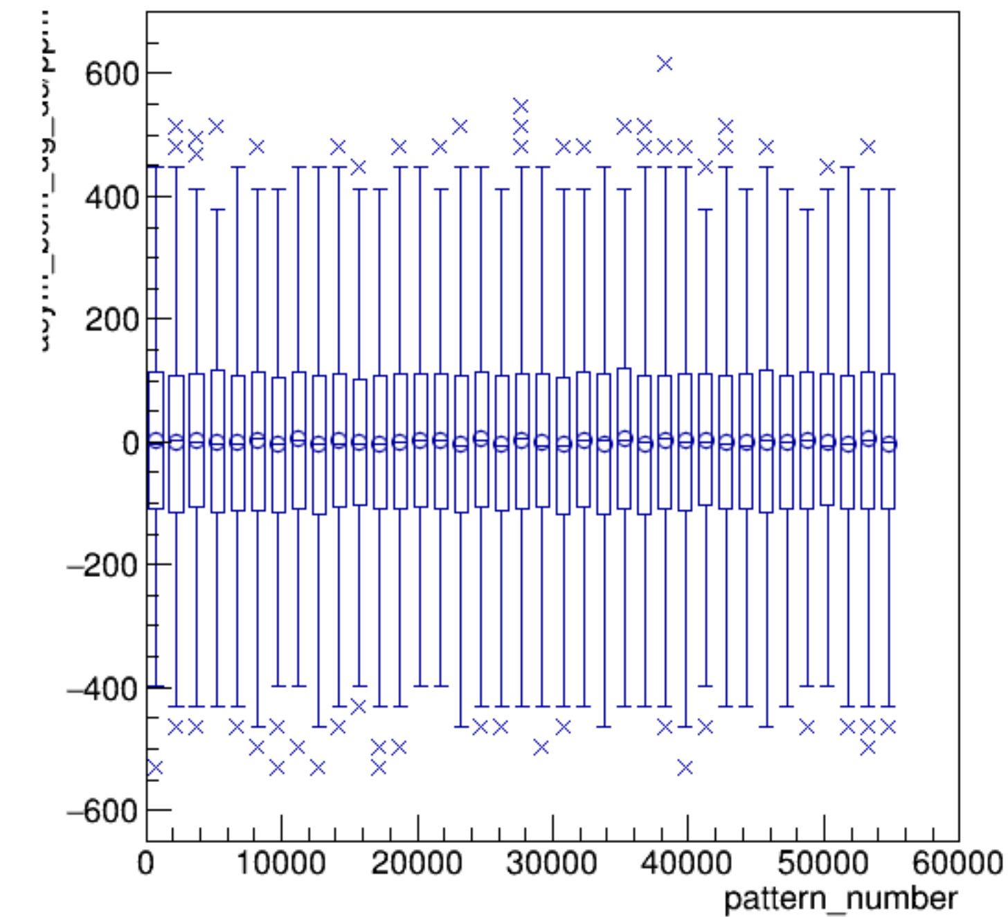
asym_bcm_dg_ds/ppm:pattern_number {ErrorFlag==0}
