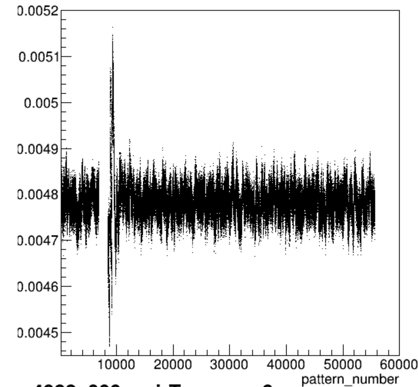
yield_sam8:pattern_number {ErrorFlag==0}
