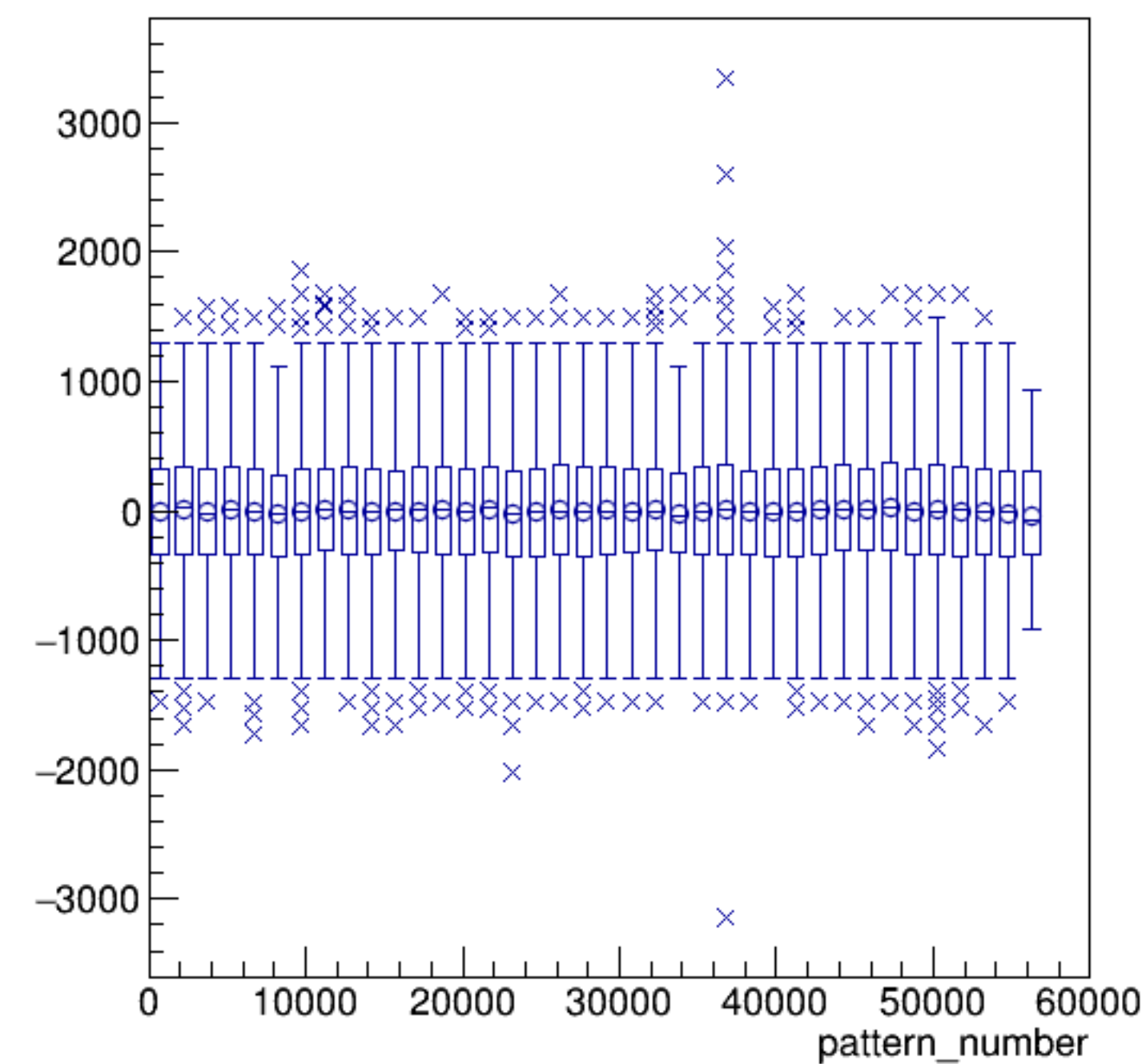
asym_sam5/ppm:pattern_number {ErrorFlag==0}
