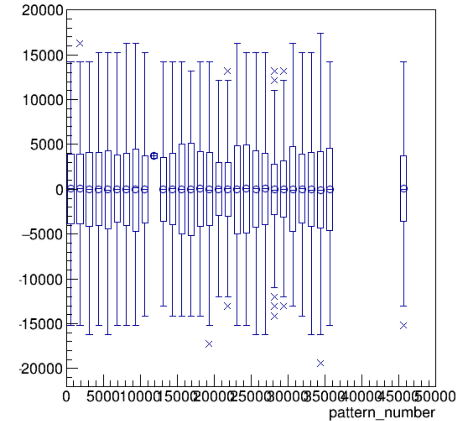
asym_sam7/ppm:pattern_number {ErrorFlag==0}
