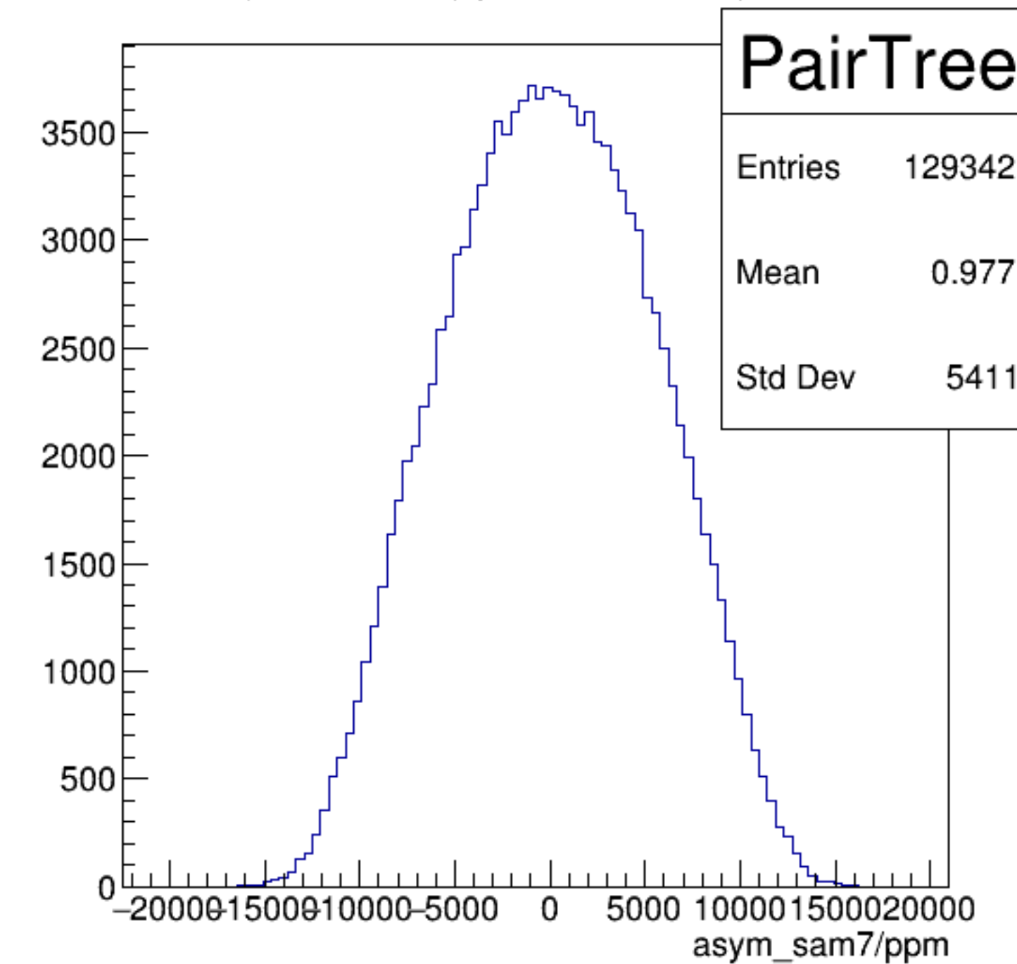
asym_sam7/ppm {ErrorFlag==0}
