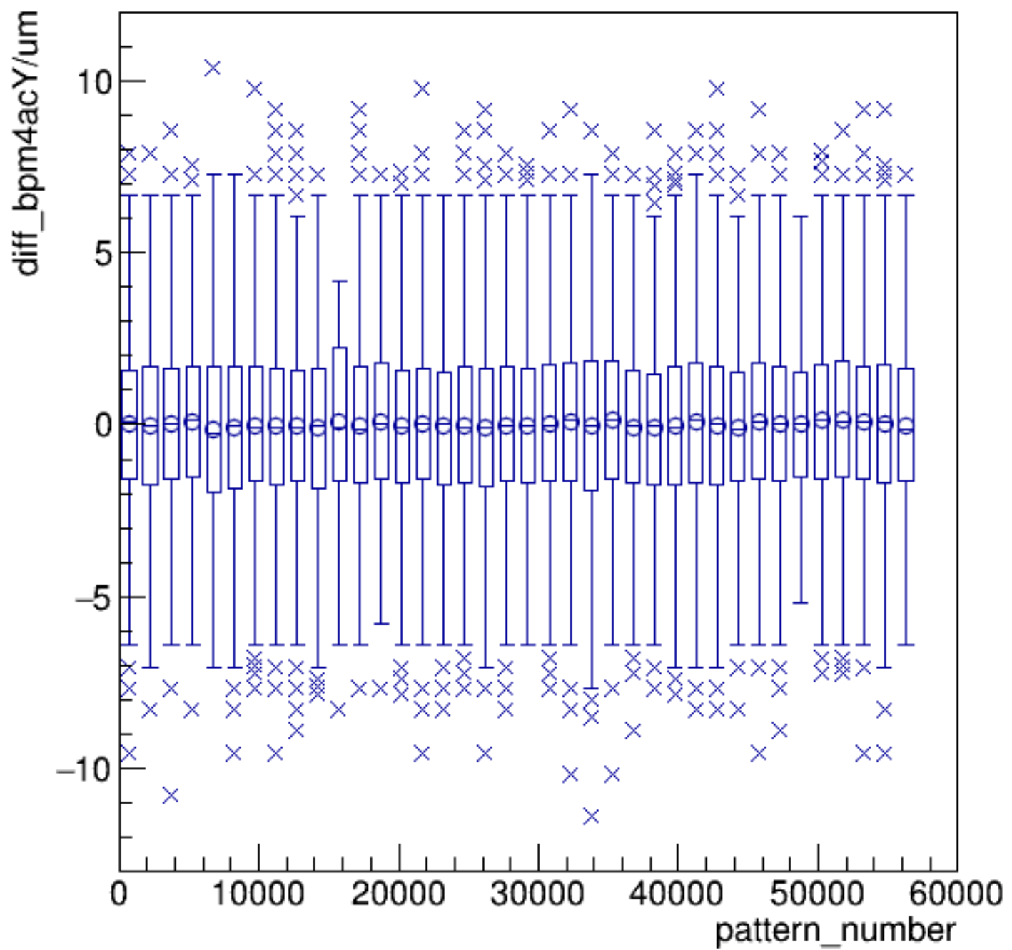
diff_bpm4acY/um:pattern_number {ErrorFlag==0}
