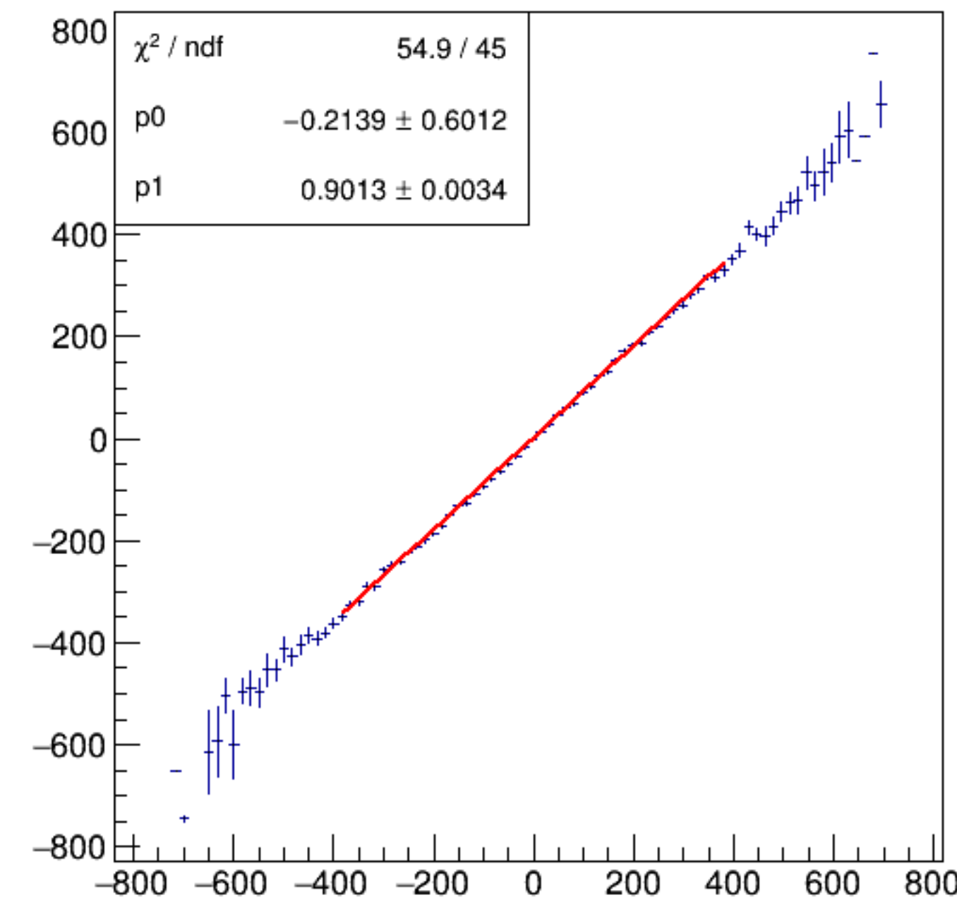
asym_bpm12WS/ppm:Aq/ppm {ErrorFlag==0}
