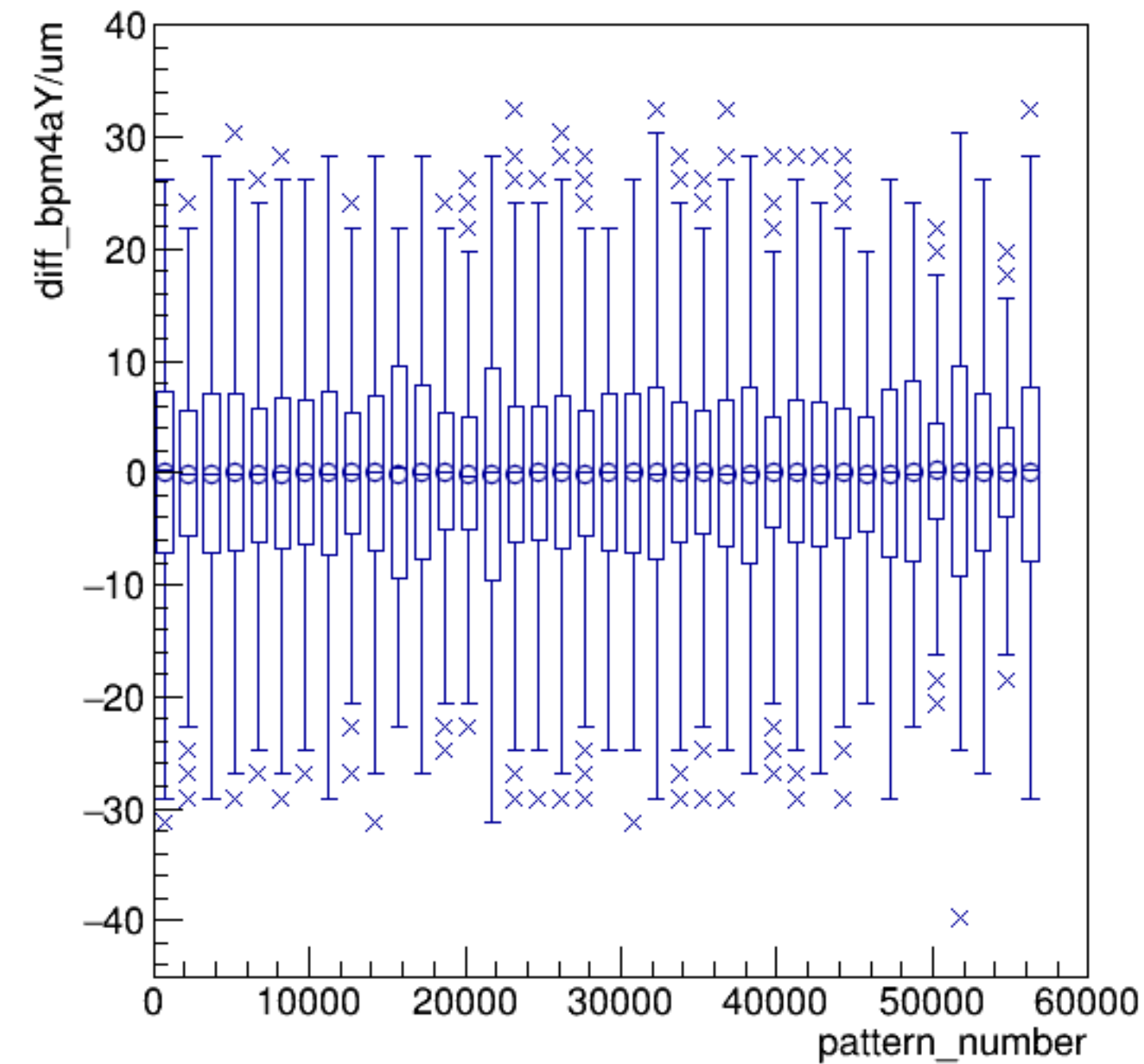
diff_bpm4aY/um:pattern_number {ErrorFlag==0}
