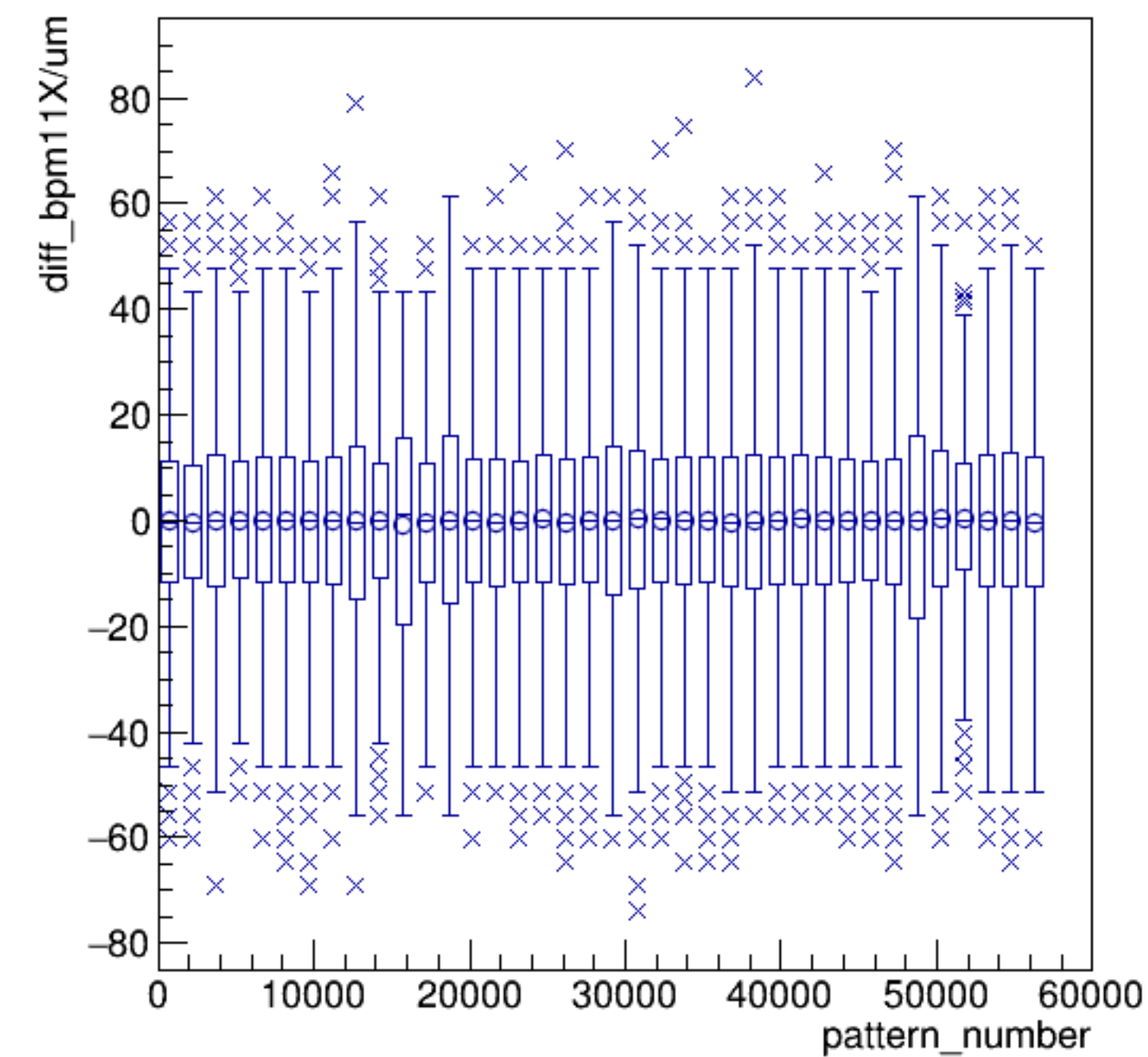
diff_bpm11X/um:pattern_number {ErrorFlag==0}
