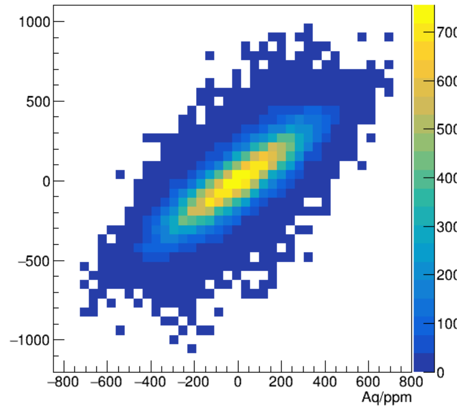
asym_bpm4aWS/ppm:Aq/ppm {ErrorFlag==0}
