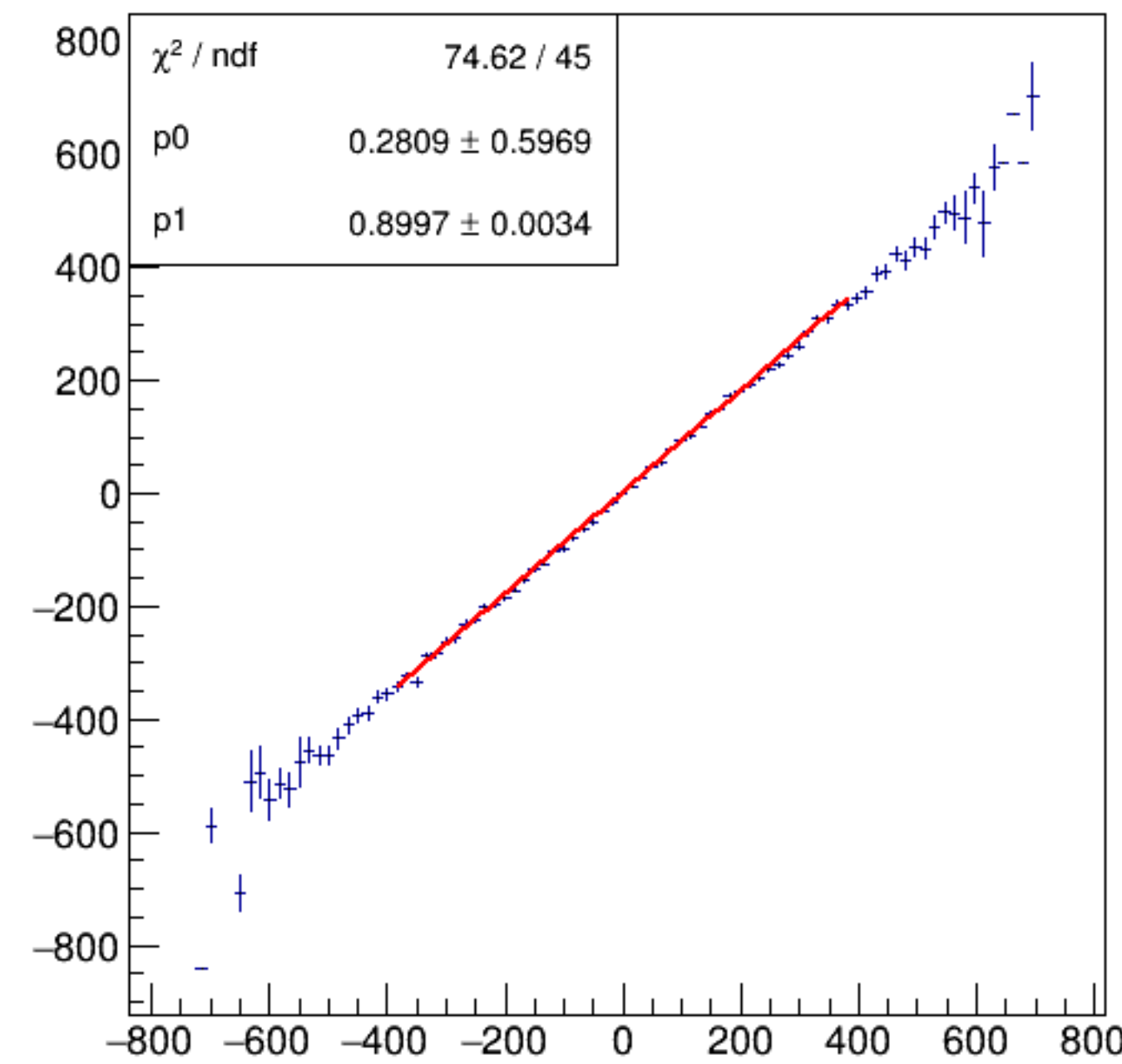
asym_bpm4aWS/ppm:Aq/ppm {ErrorFlag==0}
