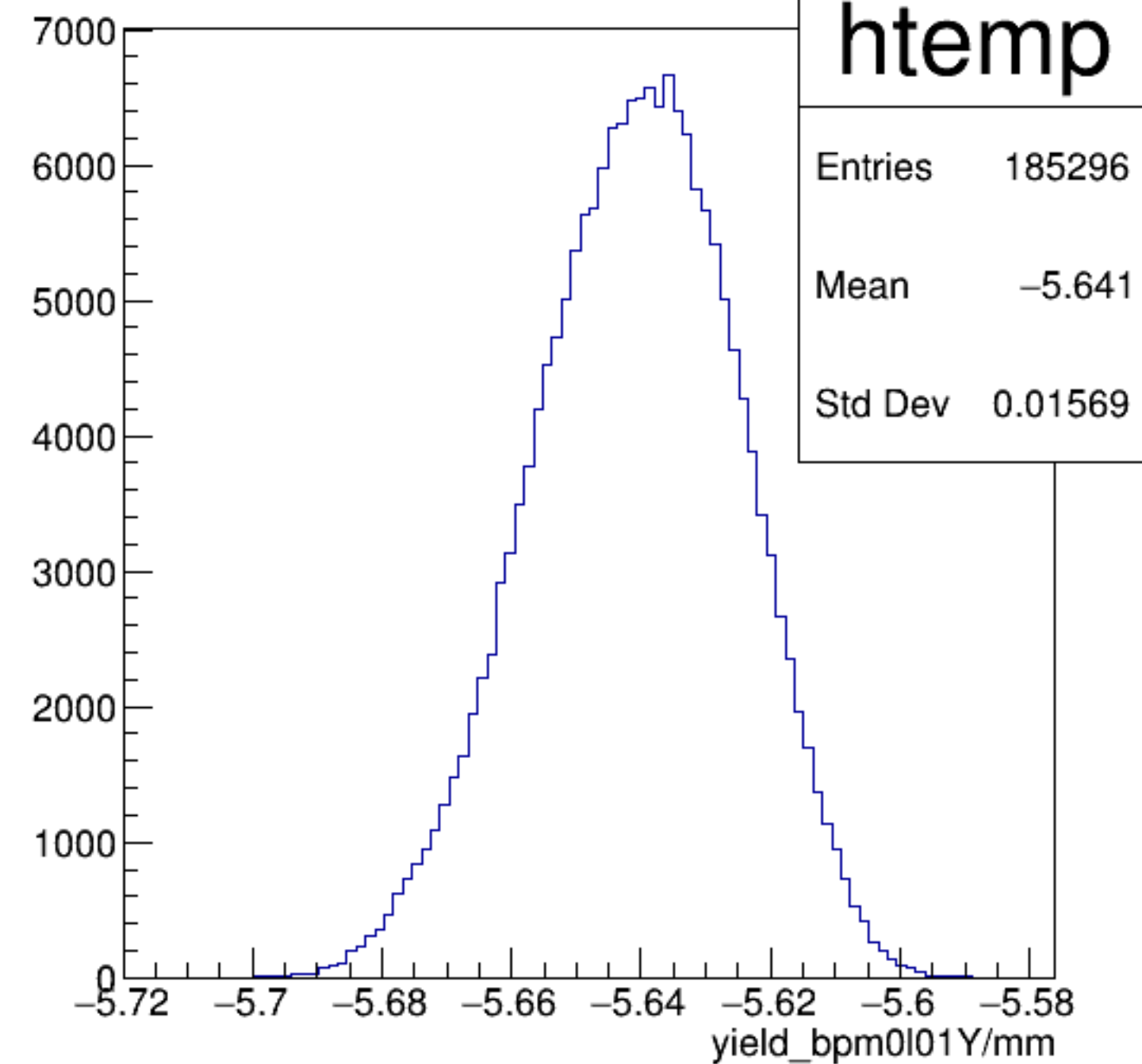
yield_bpm0l01Y/mm {ErrorFlag==0}
