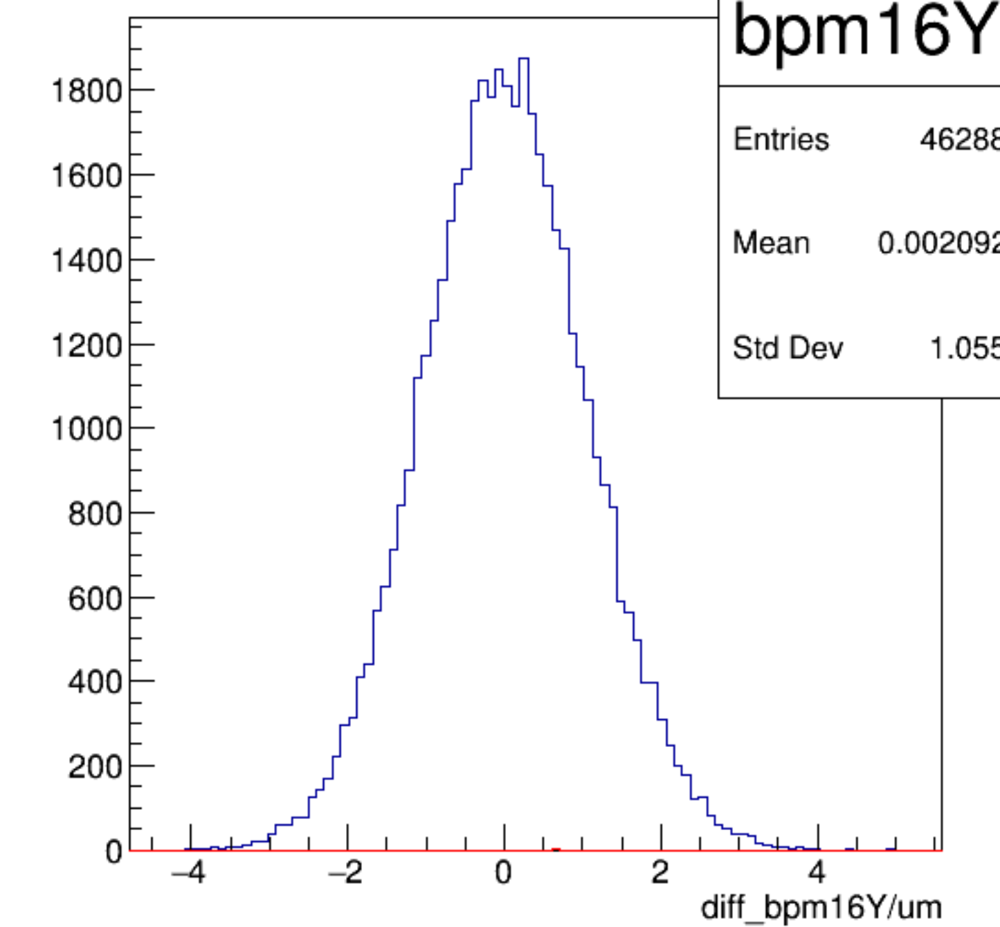
diff_bpm16Y/um {ErrorFlag==0}
