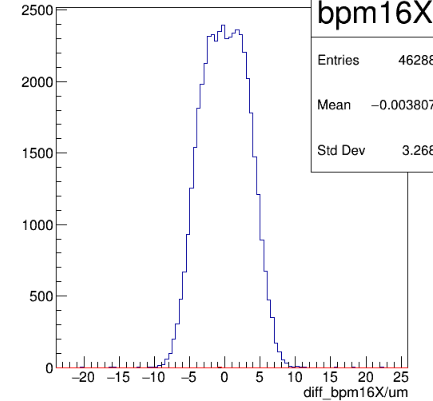
diff_bpm16X/um {ErrorFlag==0}
