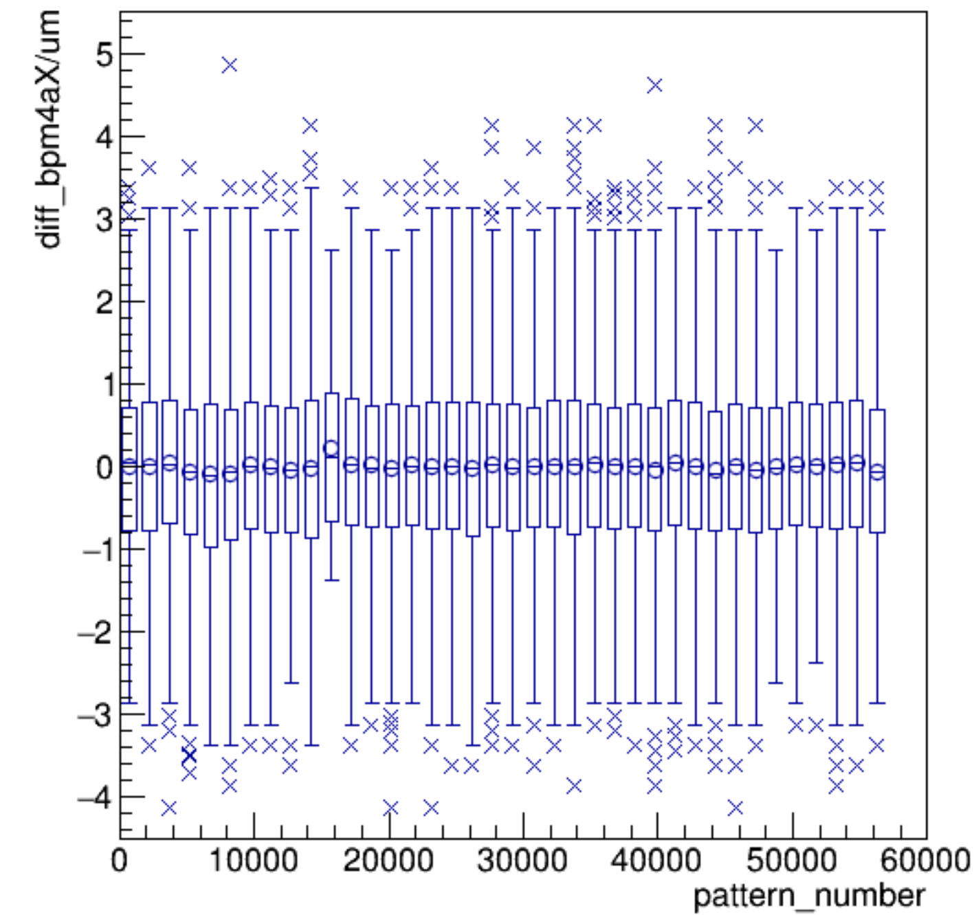
diff_bpm4aX/um:pattern_number {ErrorFlag==0}
