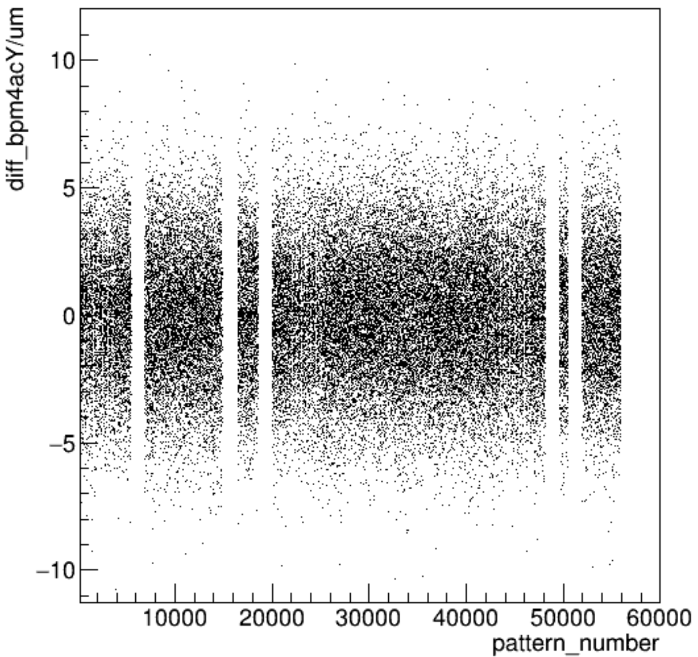
diff_bpm4acY/um:pattern_number {ErrorFlag==0}
