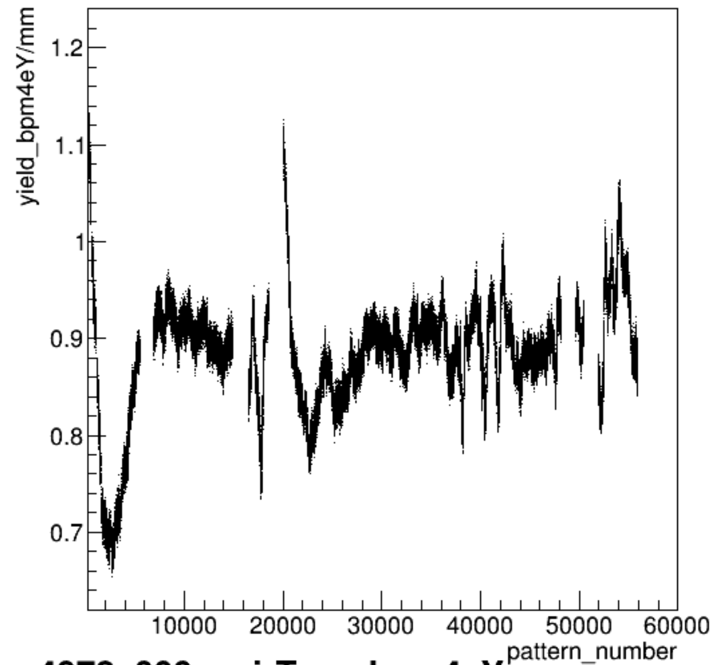
yield_bpm4eY/mm:pattern_number {ErrorFlag==0}
