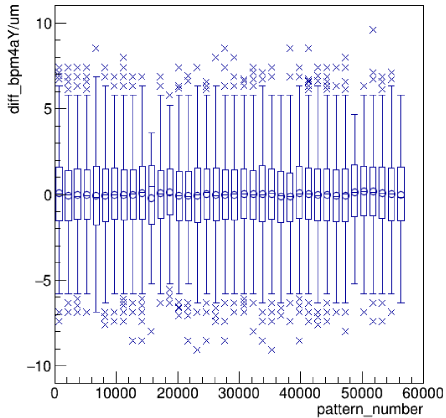
diff_bpm4aY/um:pattern_number {ErrorFlag==0}
