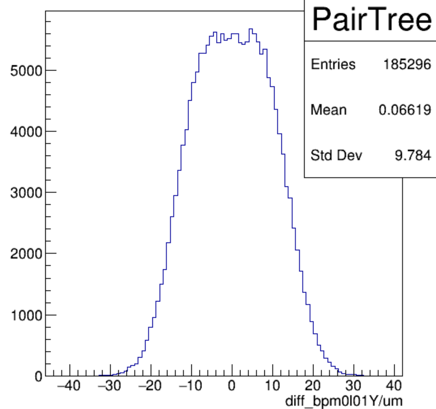
diff_bpm0l01Y/um {ErrorFlag==0}
