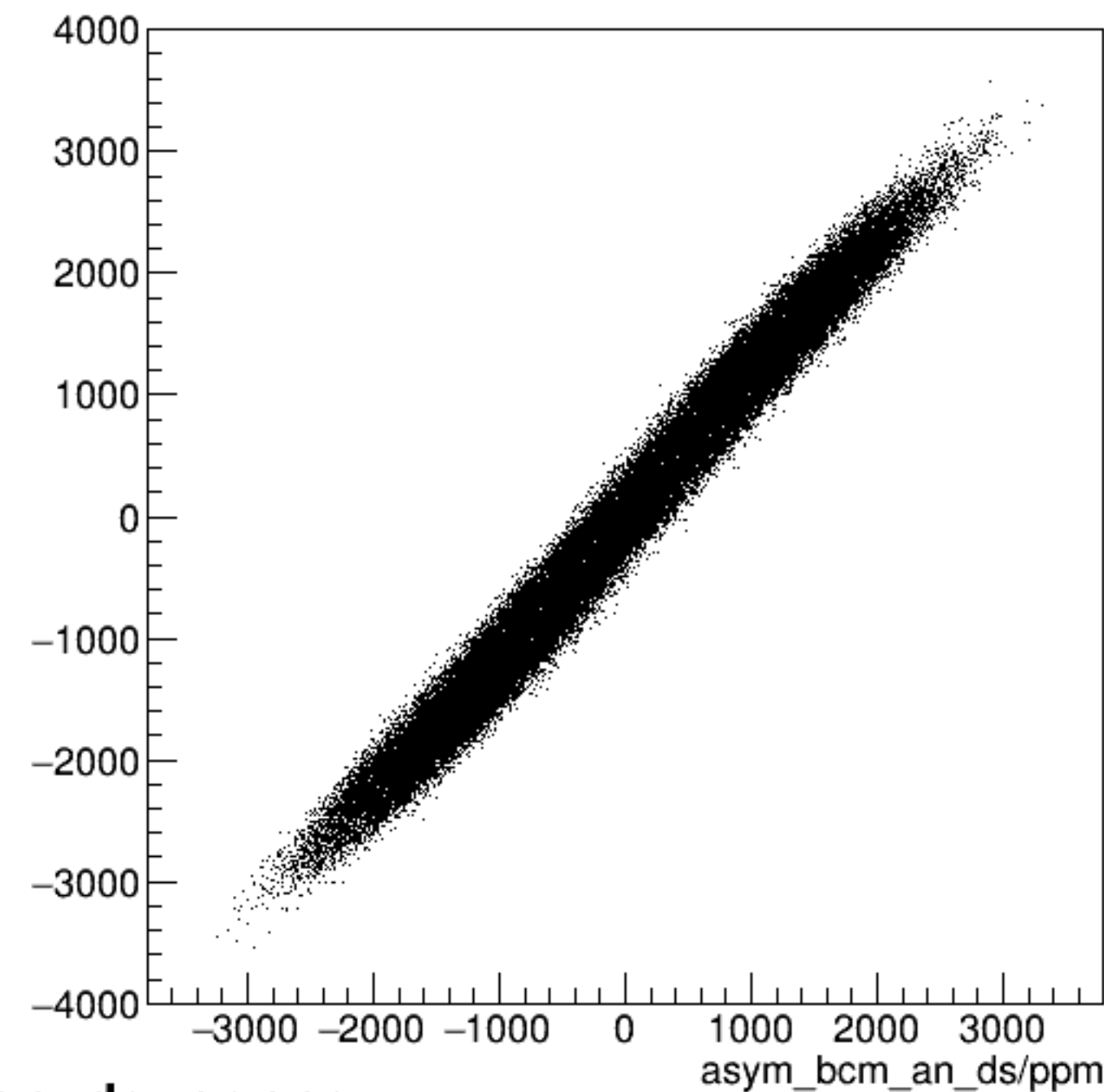
run4980_000_asym_bcm_dg_us_vs_asym_bcm_an_ds_pr.png
