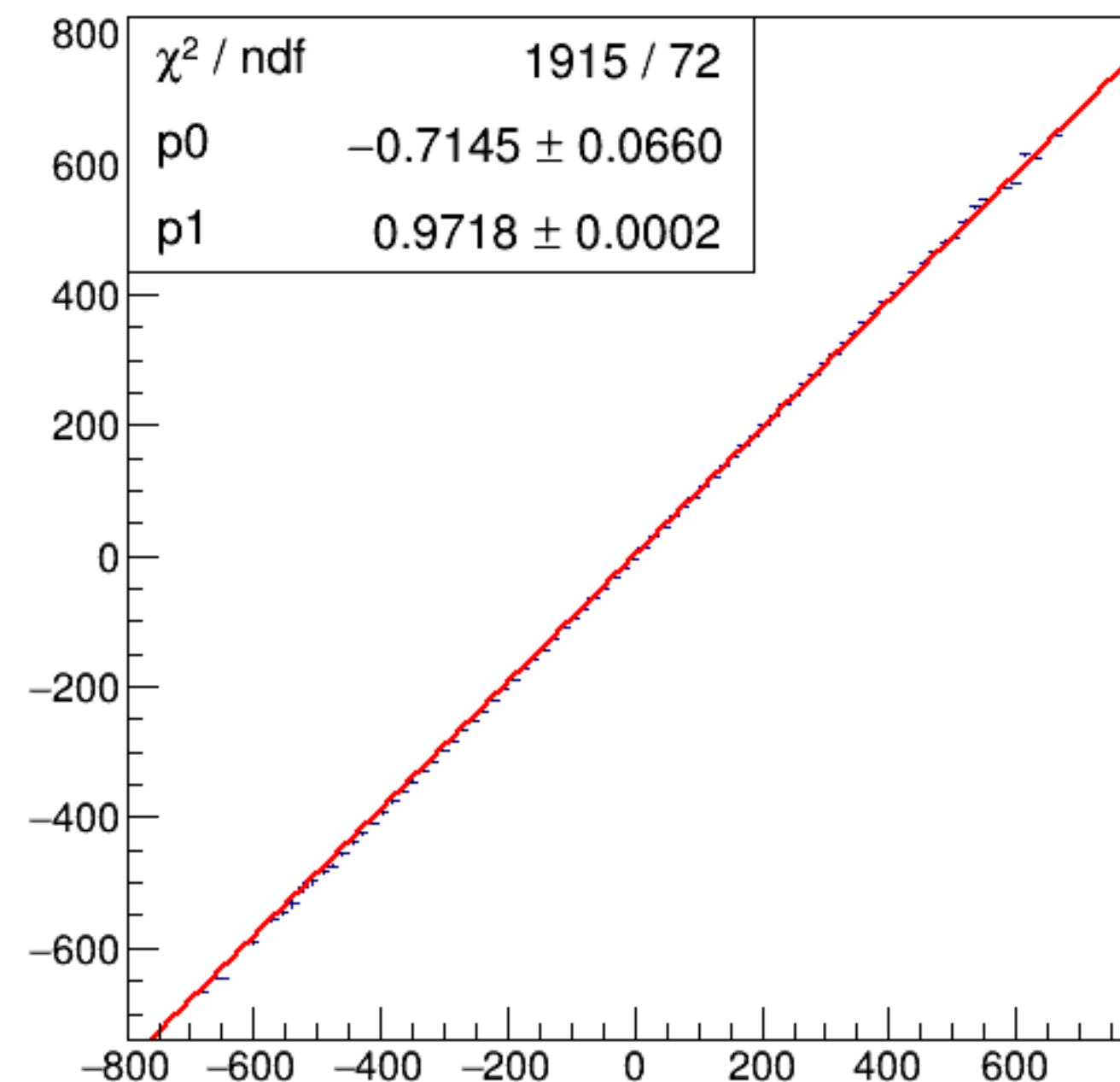
run4980_000_asym_bcm_an_ds_vs_asym_bcm_an_ds3_mul.png
