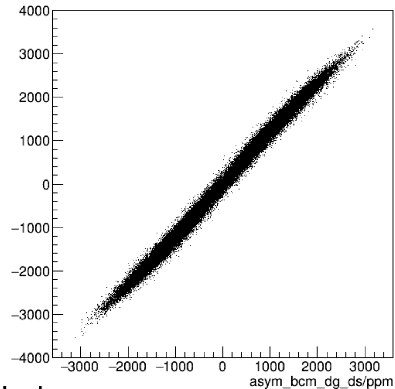
run4980_000_asym_bcm_dg_us_vs_asym_bcm_dg_ds_pr.png
