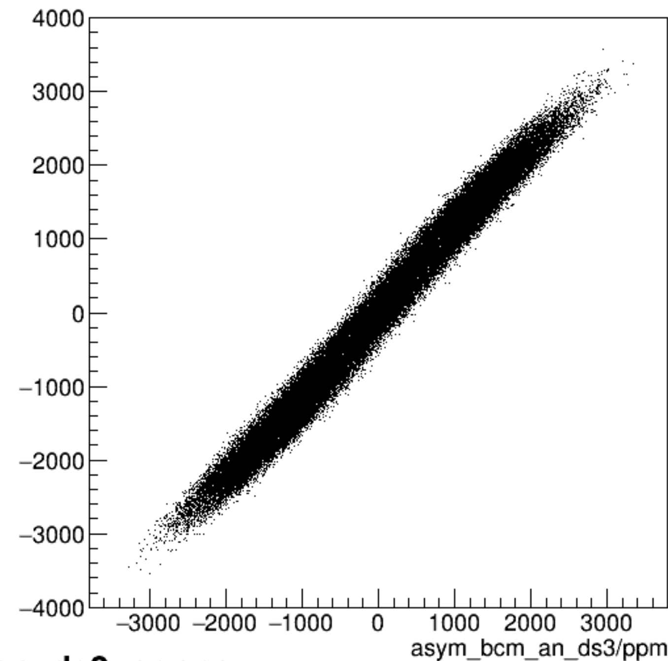
run4980_000_asym_bcm_dg_us_vs_asym_bcm_an_ds3_pr.png
