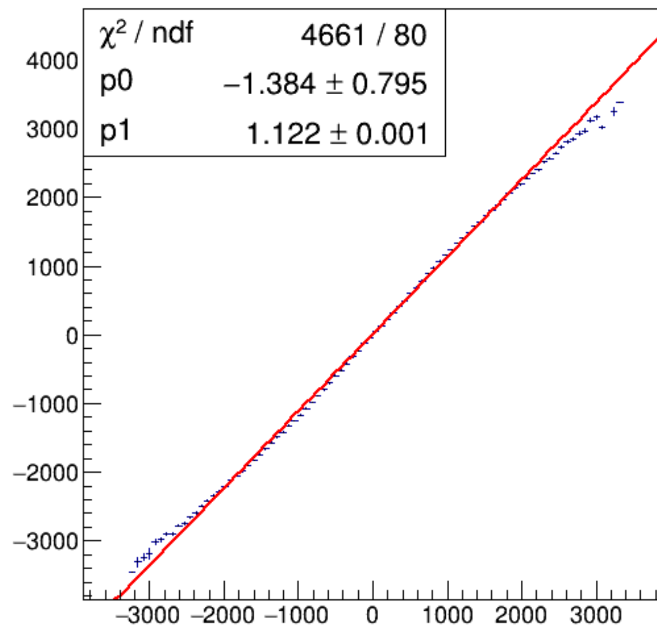
run4980_000_asym_bcm_dg_us_vs_asym_bcm_an_ds3_pr.png
