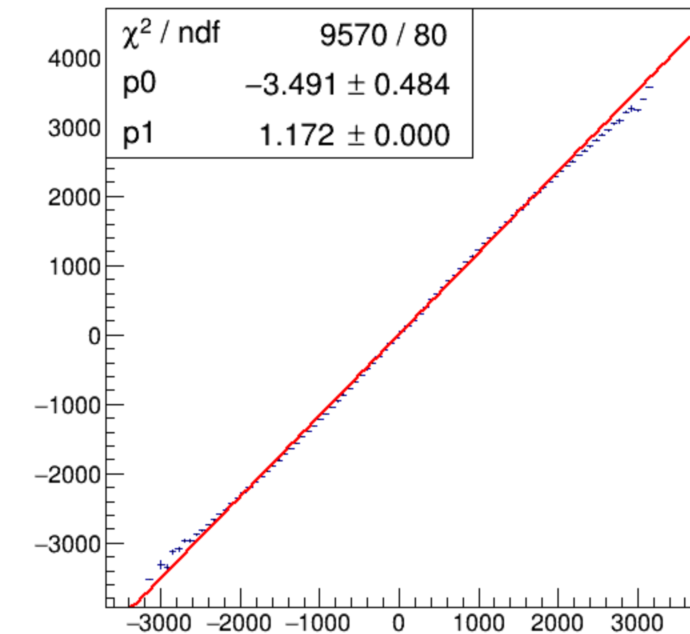
run4980_000_asym_bcm_dg_us_vs_asym_bcm_dg_ds_pr.png
