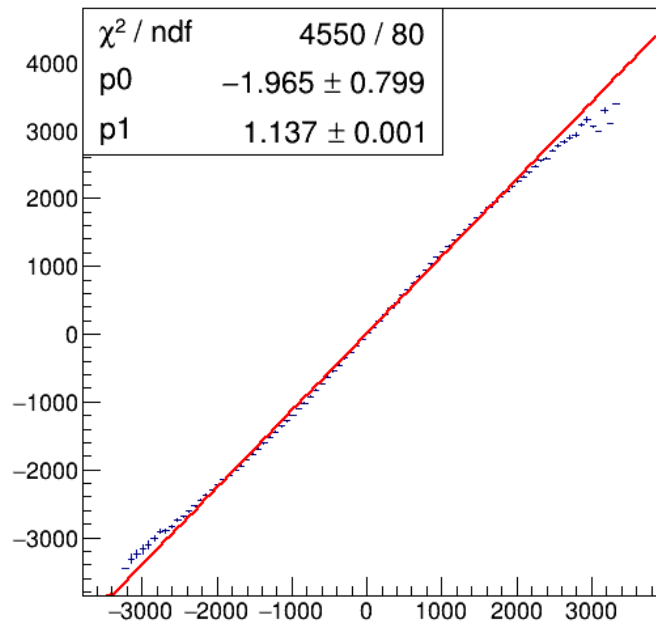
run4980_000_asym_bcm_dg_us_vs_asym_bcm_an_ds_pr.png
