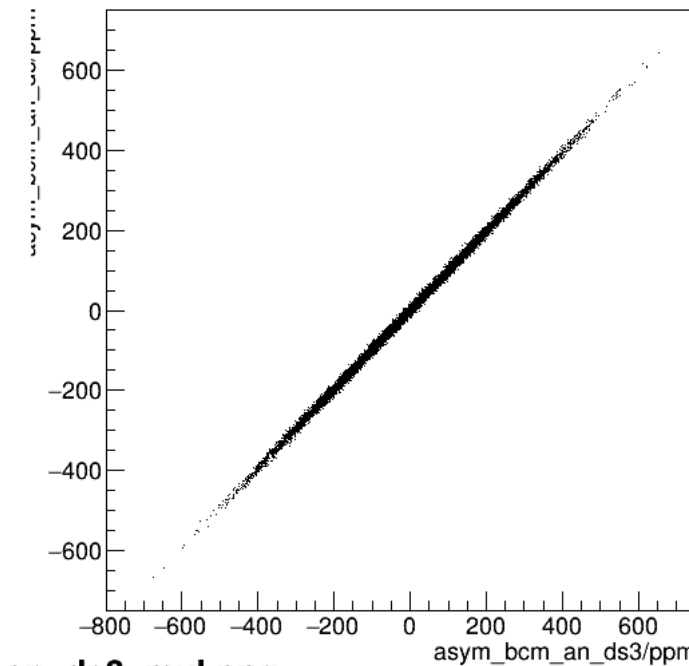
run4980_000_asym_bcm_an_ds_vs_asym_bcm_an_ds3_mul.png
