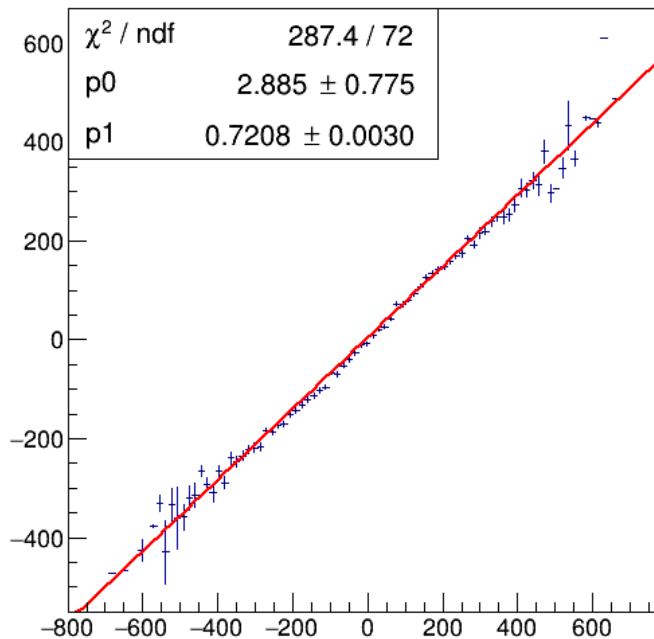
run4980_000_asym_bcm_an_us_vs_asym_bcm_an_ds3_mul.png
