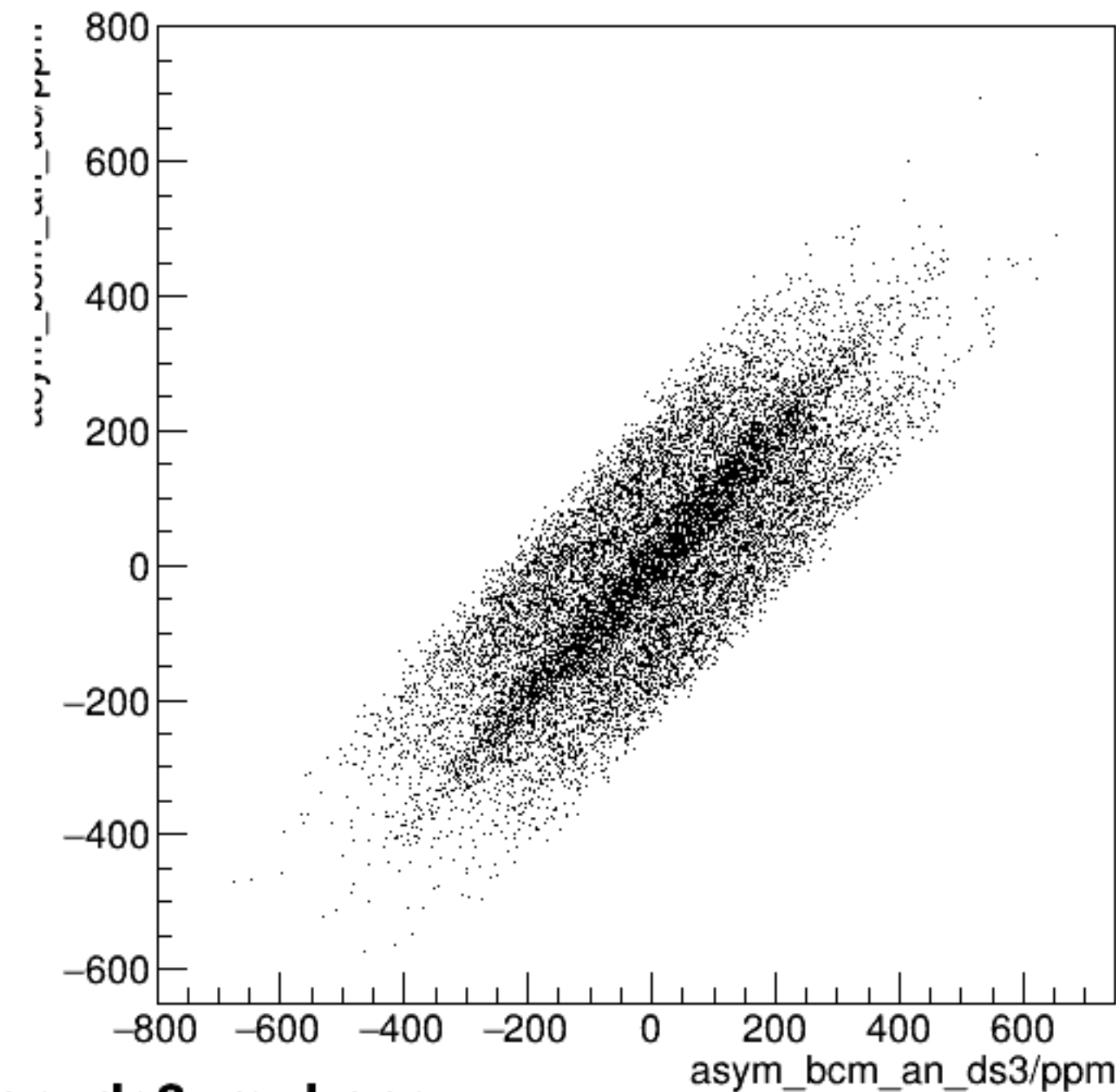
run4980_000_asym_bcm_an_us_vs_asym_bcm_an_ds3_mul.png
