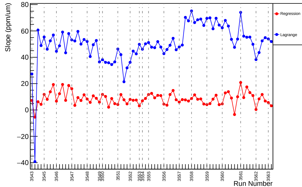
Slug10: Slope : usl_vs_evMon10 (ppm/um)
