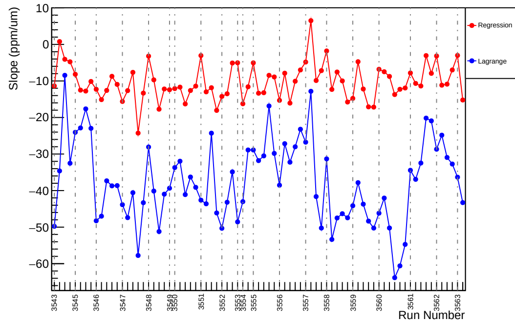
Slug10: Slope : usl_vs_evMon11 (ppm/um)
