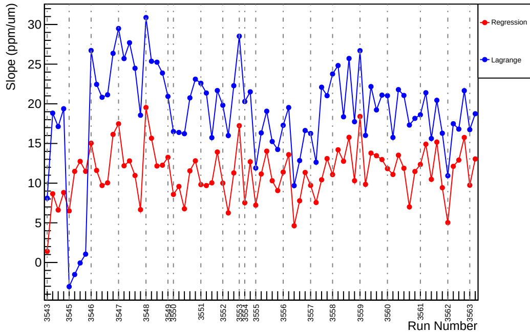
Slug10: Slope : usl_vs_evMon8 (ppm/um)
