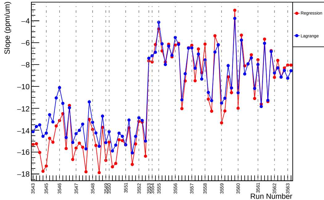
Slug10: Slope : usl_vs_evMon6 (ppm/um)
