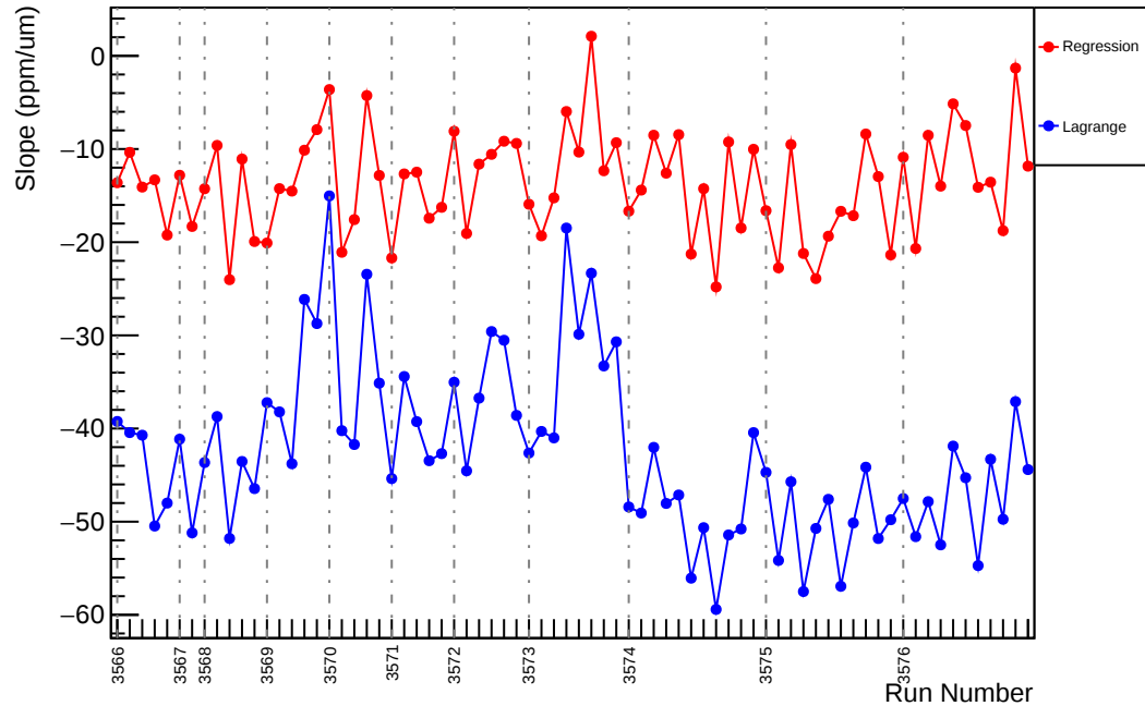
Slug11: Slope : usl_vs_evMon11 (ppm/um)
