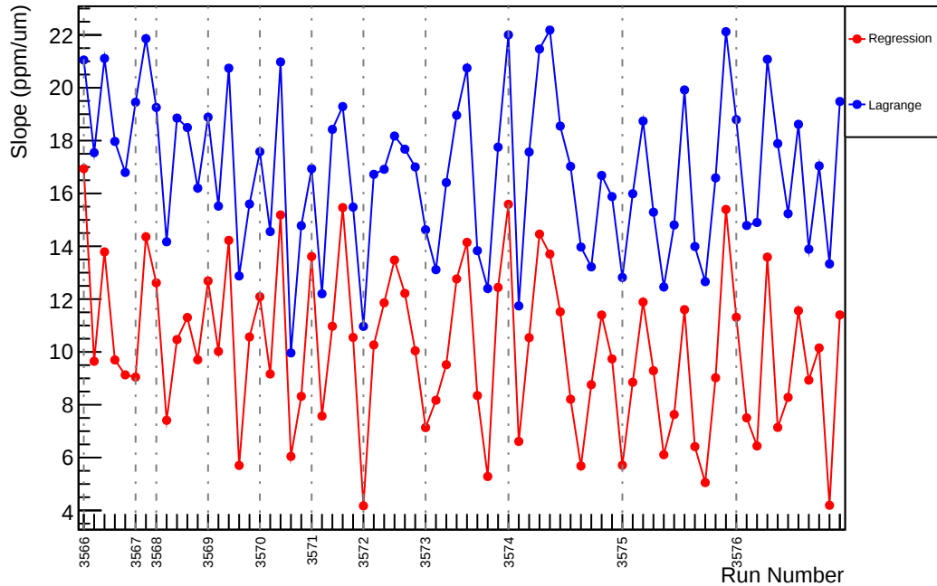
Slug11: Slope : usl_vs_evMon8 (ppm/um)
