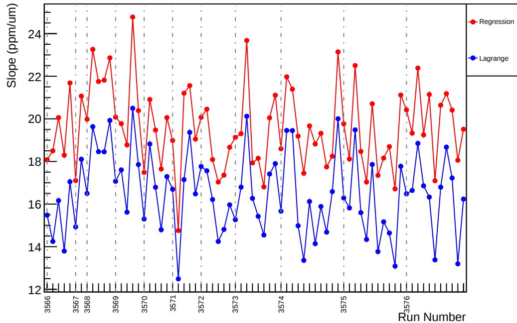
Slug11: Slope : usl_vs_evMon7 (ppm/um)
