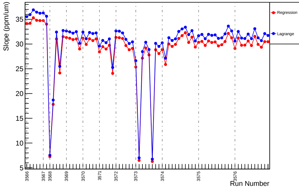
Slug11: Slope : usl_vs_evMon0 (ppm/um)
