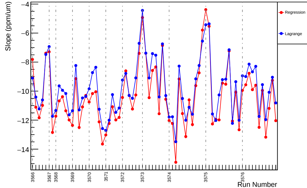
Slug11: Slope : usl_vs_evMon6 (ppm/um)
