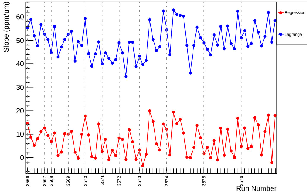
Slug11: Slope : usl_vs_evMon10 (ppm/um)
