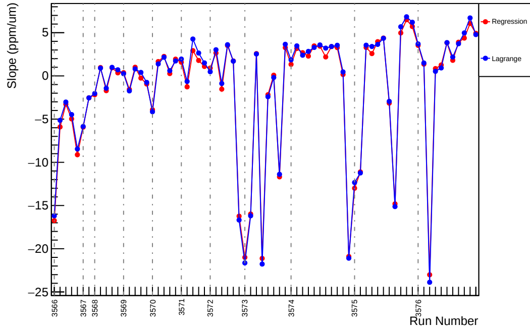
Slug11: Slope : usl_vs_evMon3 (ppm/um)
