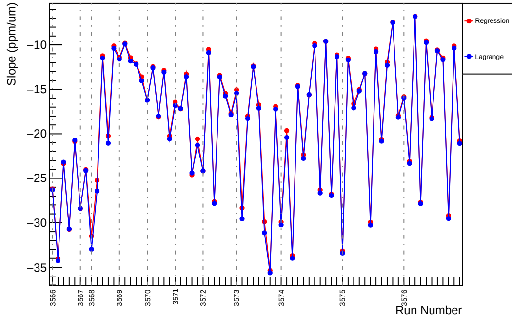
Slug11: Slope : usl_vs_evMon1 (ppm/um)
