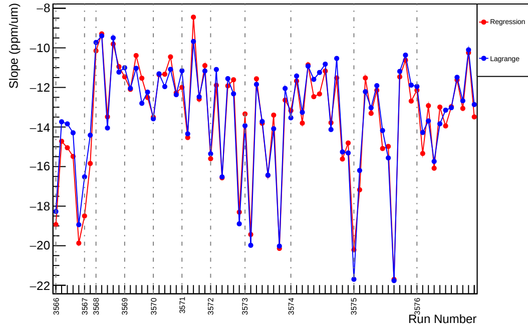
Slug11: Slope : usl_vs_evMon4 (ppm/um)
