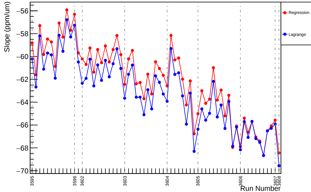
Slug12: Slope : usl_vs_evMon0 (ppm/um)
