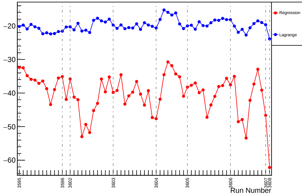
Slug12: Slope : usl_vs_evMon4 (ppm/um)
