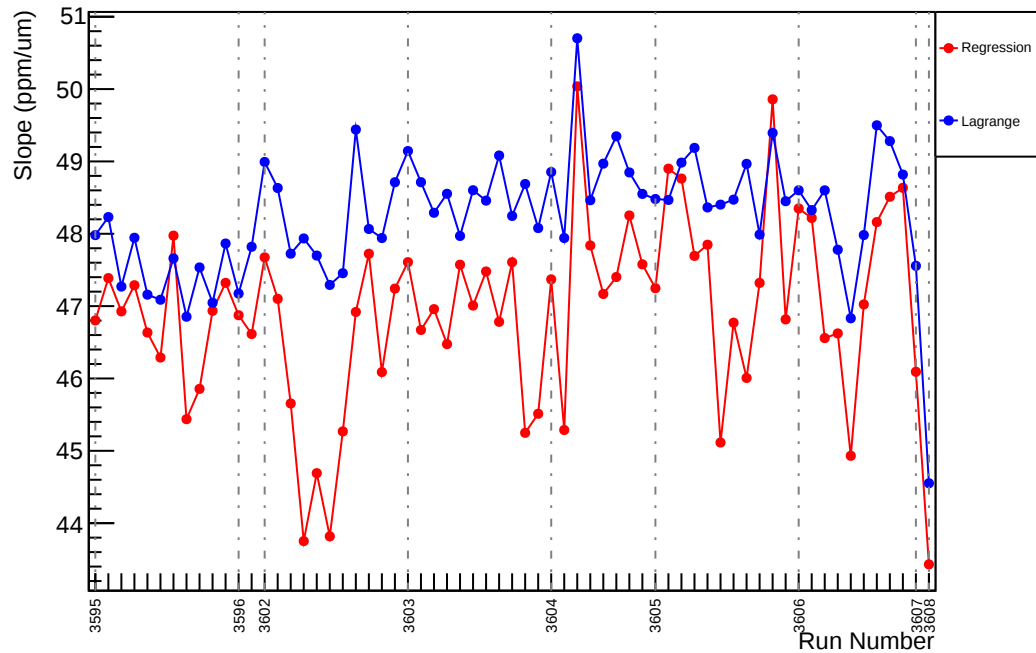
Slug12: Slope : usl_vs_evMon3 (ppm/um)
