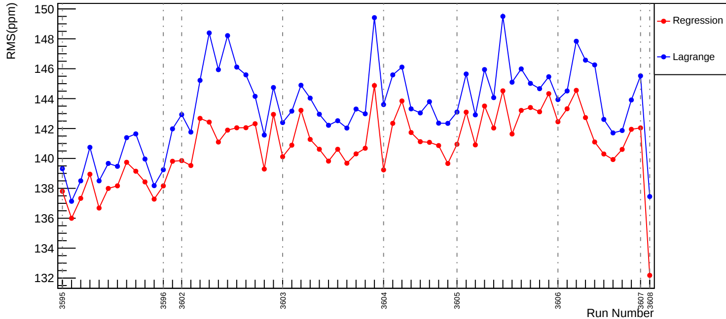
Slug12: Corrected RMS (ppm): asym_usl
