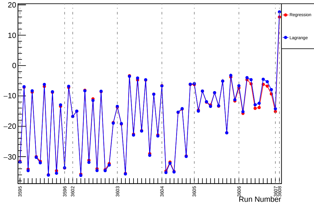
Slug12: Slope : usl_vs_evMon2 (ppm/um)
