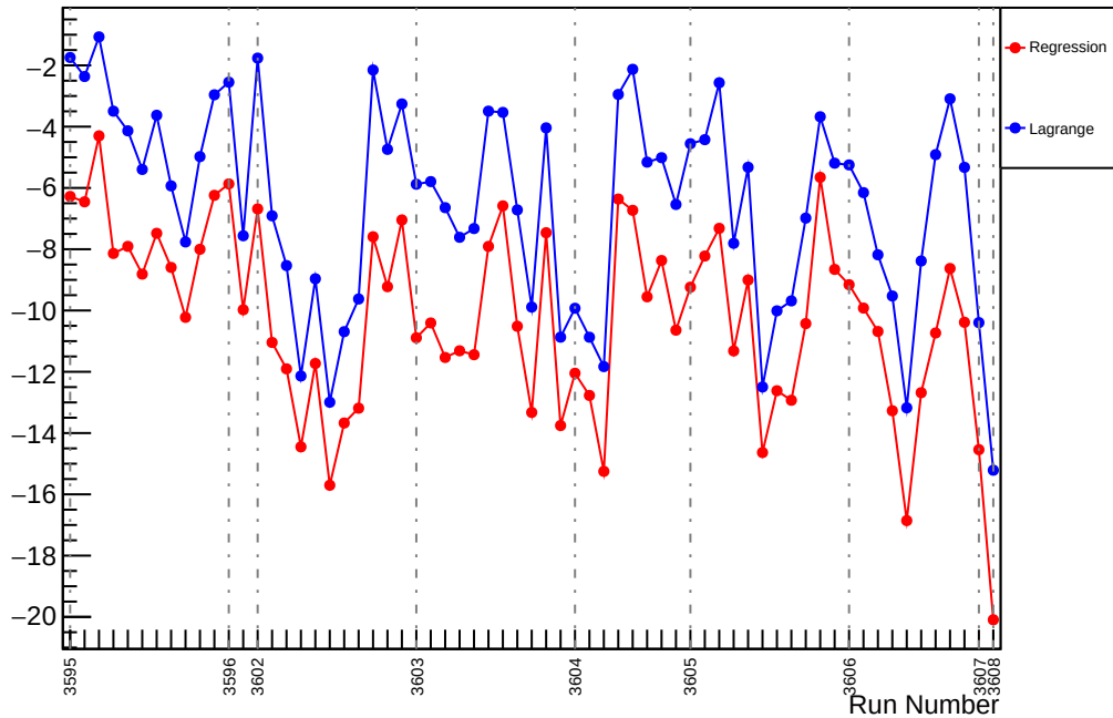
Slug12: Slope : usl_vs_evMon6 (ppm/um)
