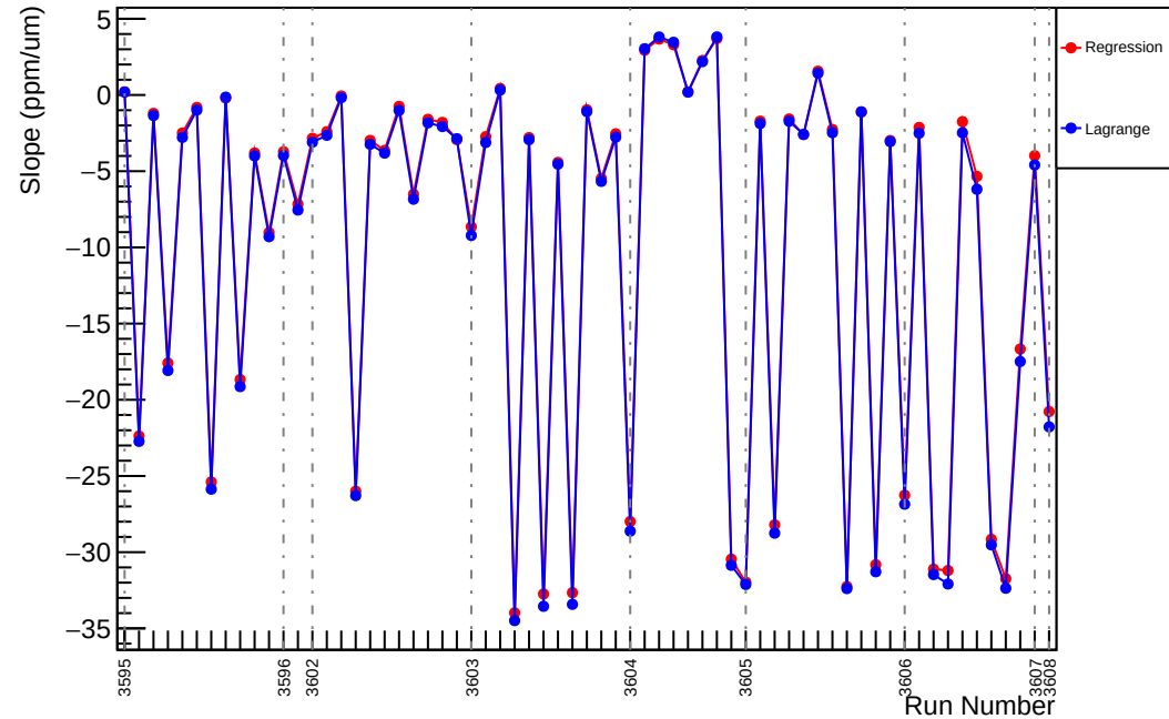
Slug12: Slope : usl_vs_evMon1 (ppm/um)
