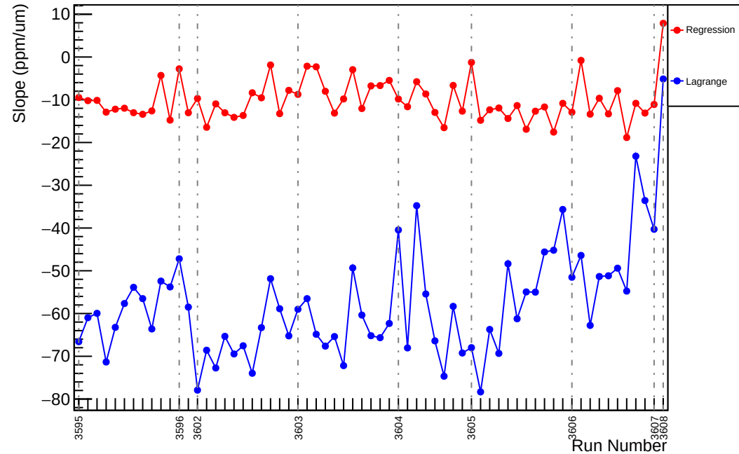
Slug12: Slope : usl_vs_evMon10 (ppm/um)
