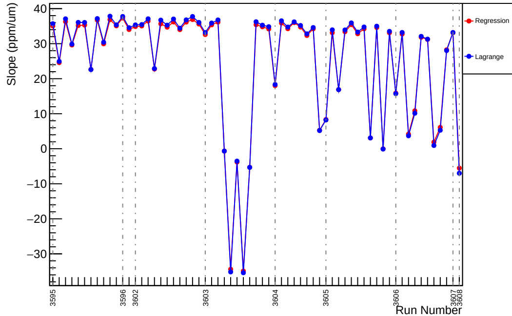
Slug12: Slope : usl_vs_evMon2 (ppm/um)
