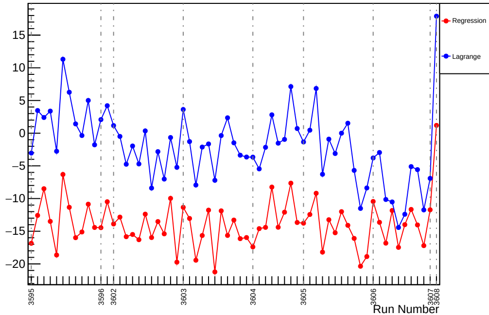
Slug12: Slope : usl_vs_evMon9 (ppm/um)
