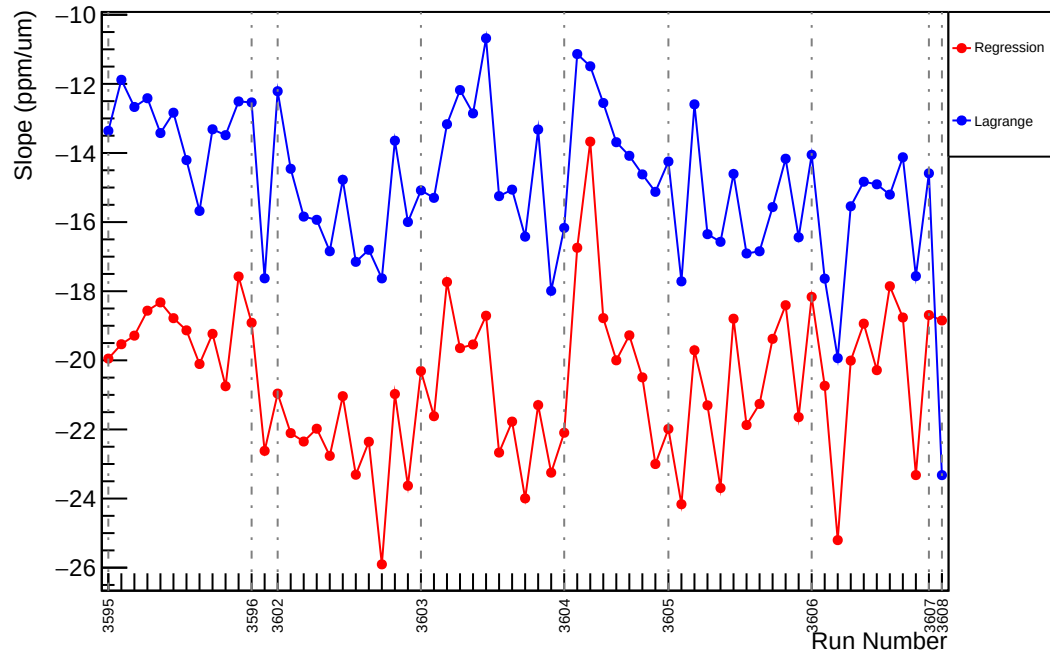
Slug12: Slope : usl_vs_evMon7 (ppm/um)
