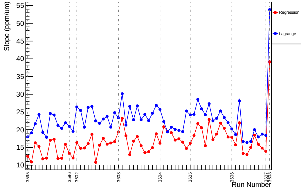
Slug12: Slope : usl_vs_evMon8 (ppm/um)
