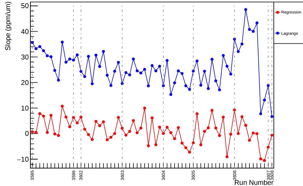
Slug12: Slope : usr_vs_evMon10 (ppm/um)
