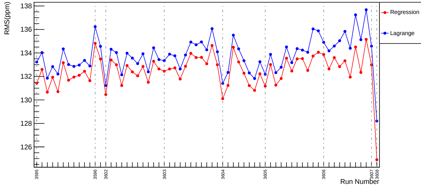
Slug12: Corrected RMS (ppm): asym_usr
