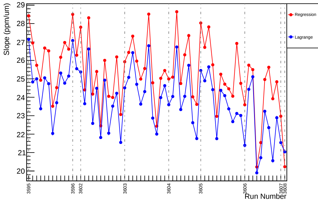
Slug12: Slope : usr_vs_evMon6 (ppm/um)
