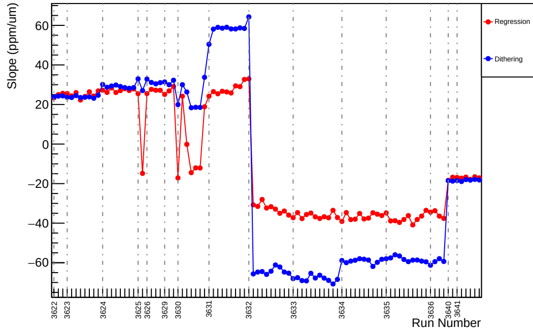
Slug13: Slope : us_avg_vs_evMon3 (ppm/um)
