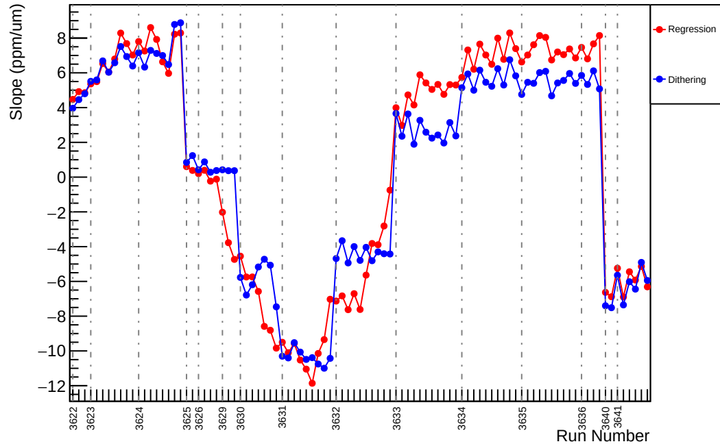
Slug13: Slope : us_avg_vs_evMon0 (ppm/um)
