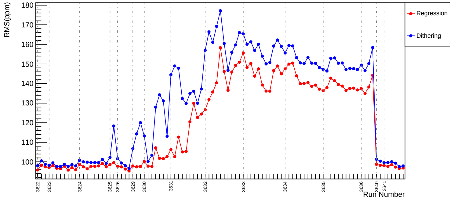
Slug13: Corrected RMS (ppm): asym_us_avg
