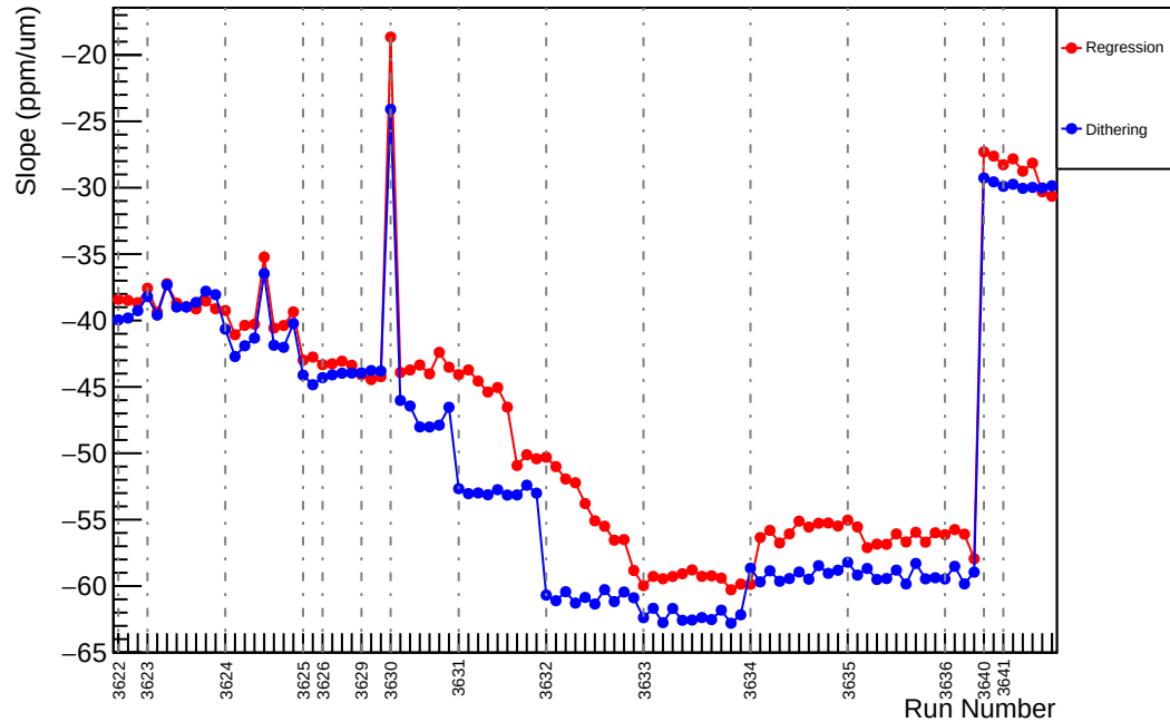
Slug13: Slope : us_avg_vs_evMon2 (ppm/um)
