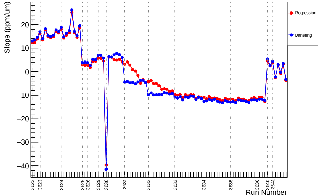
Slug13: Slope : us_avg_vs_evMon1 (ppm/um)
