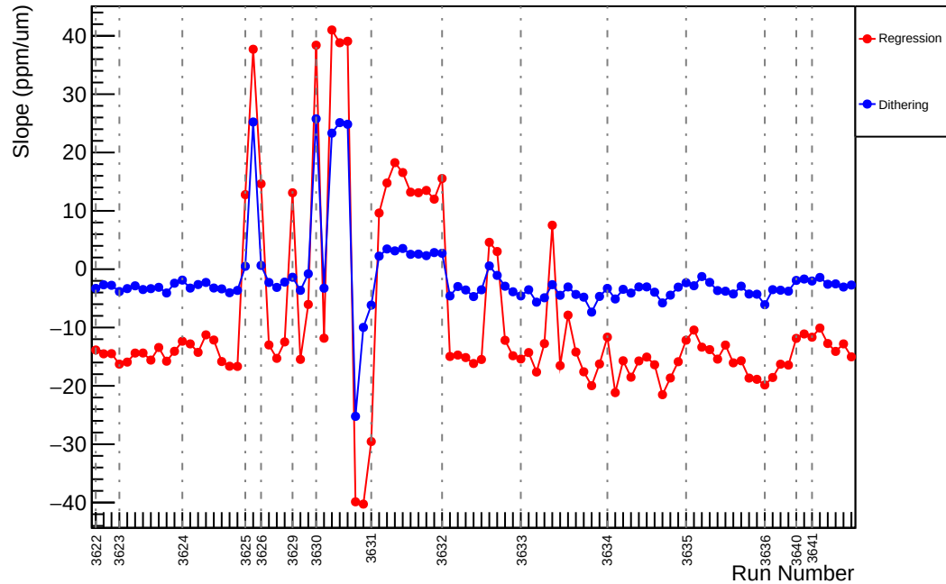
Slug13: Slope : us_dd_vs_evMon4 (ppm/um)
