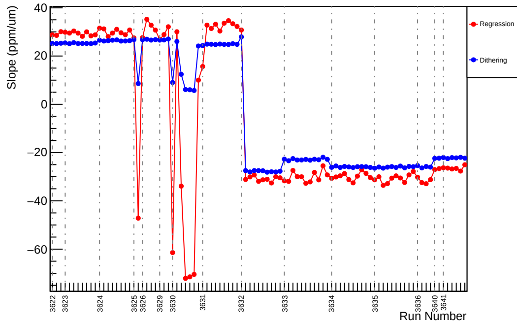
Slug13: Slope : us_dd_vs_evMon3 (ppm/um)
