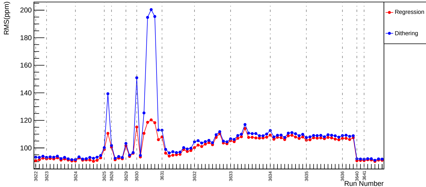
Slug13: Corrected RMS (ppm): asym_us_dd
