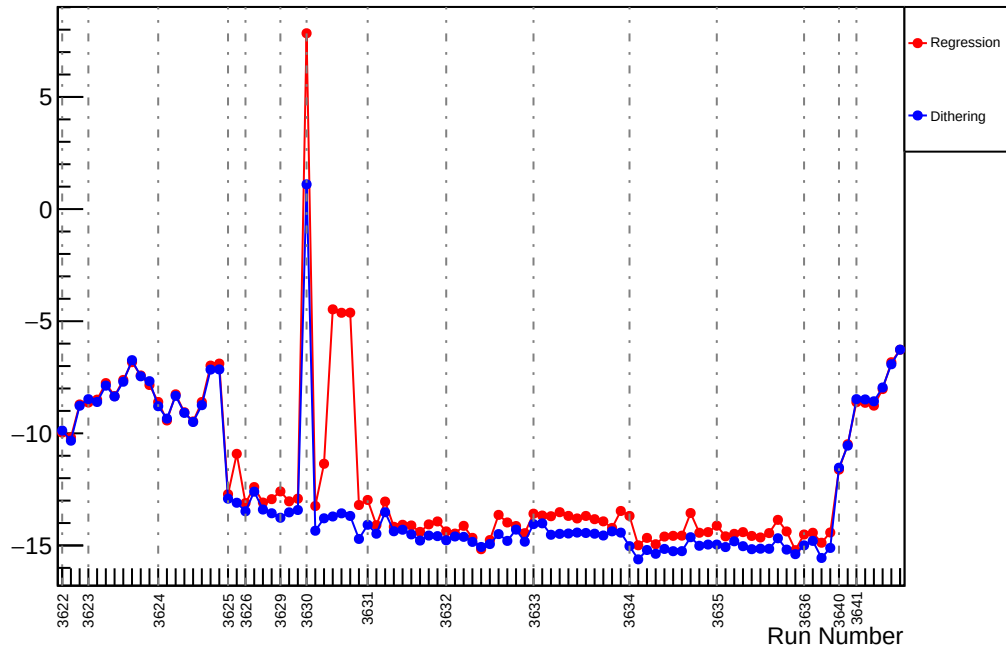
Slug13: Slope : us_dd_vs_evMon2 (ppm/um)
