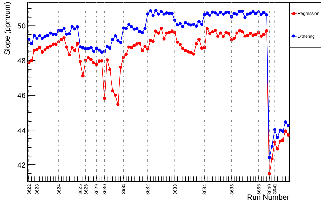
Slug13: Slope : us_dd_vs_evMon0 (ppm/um)
