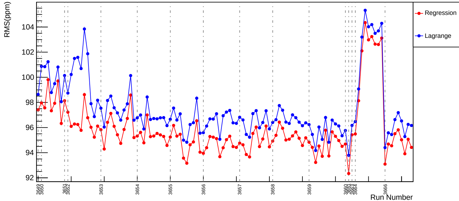
Slug14: Corrected RMS (ppm): asym_us_avg
