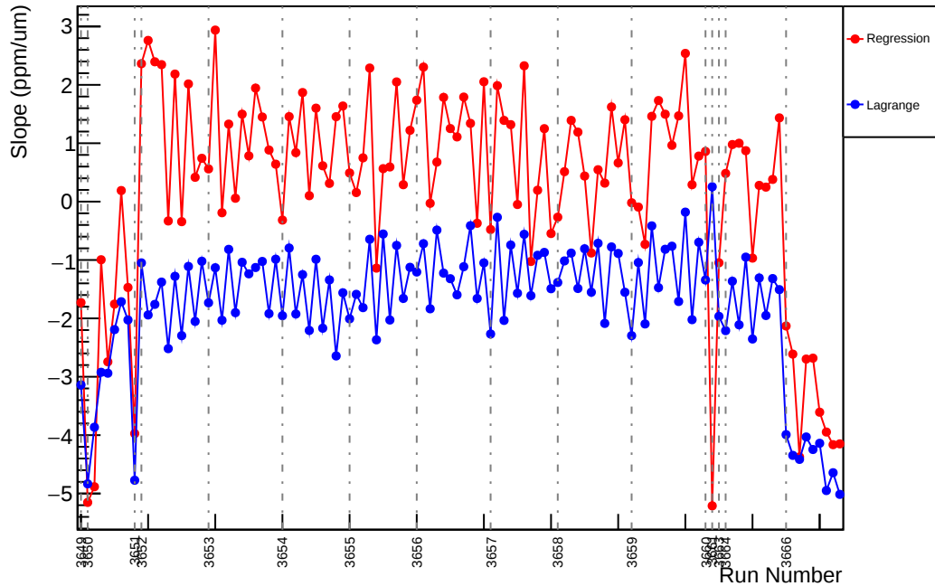
Slug14: Slope : usr_vs_evMon3 (ppm/um)
