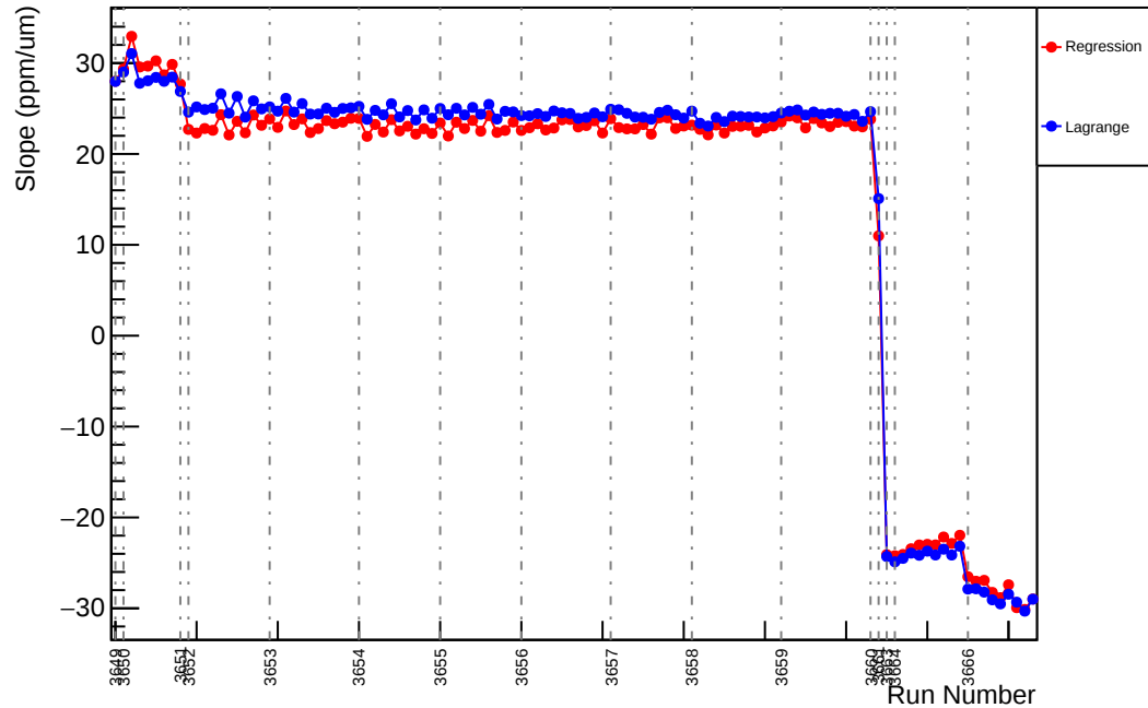
Slug14: Slope : usr_vs_evMon2 (ppm/um)
