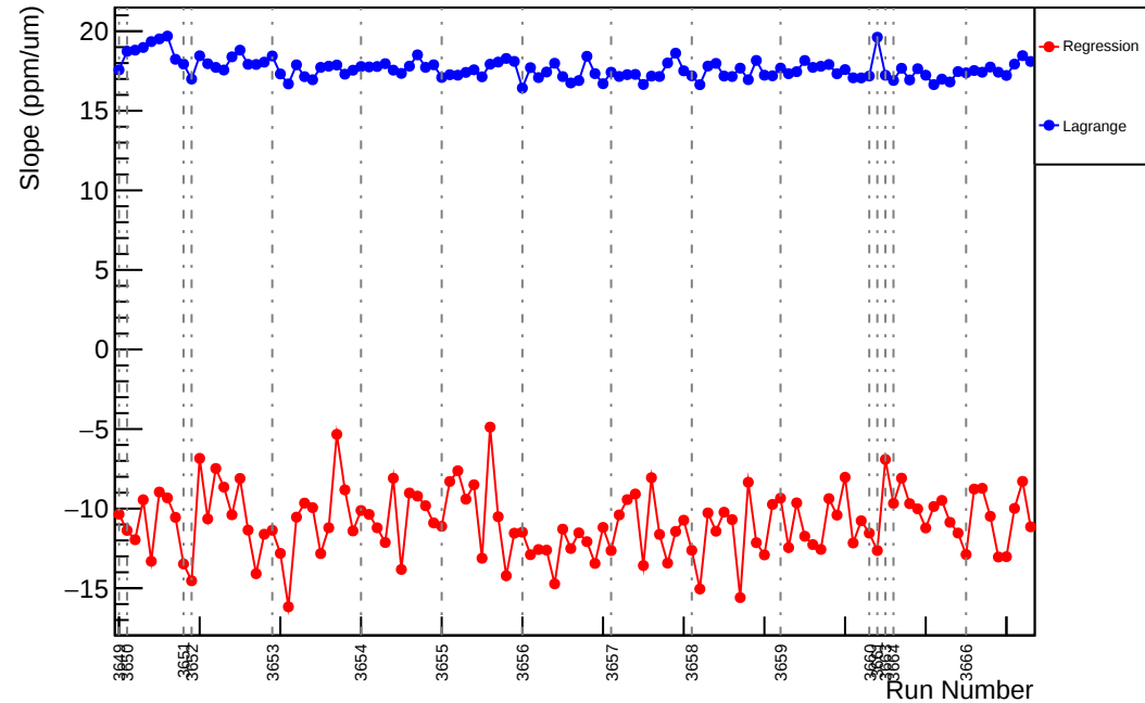
Slug14: Slope : usr_vs_evMon4 (ppm/um)
