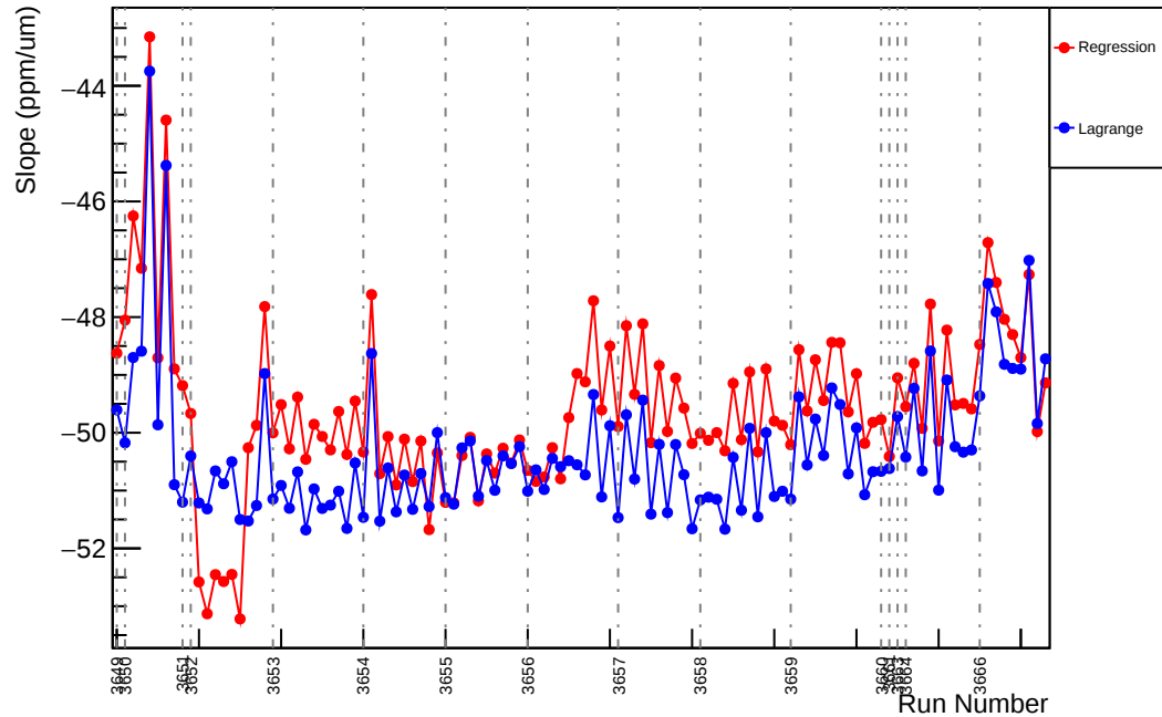
Slug14: Slope : usr_vs_evMon0 (ppm/um)
