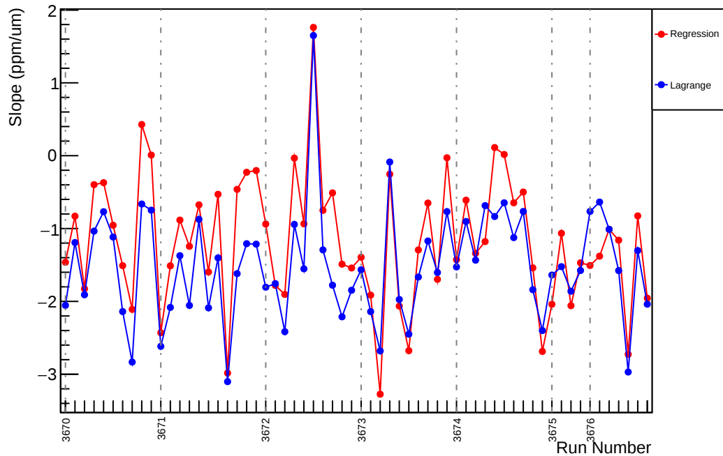
Slug15: Slope : us_avg_vs_evMon5 (ppm/um)
