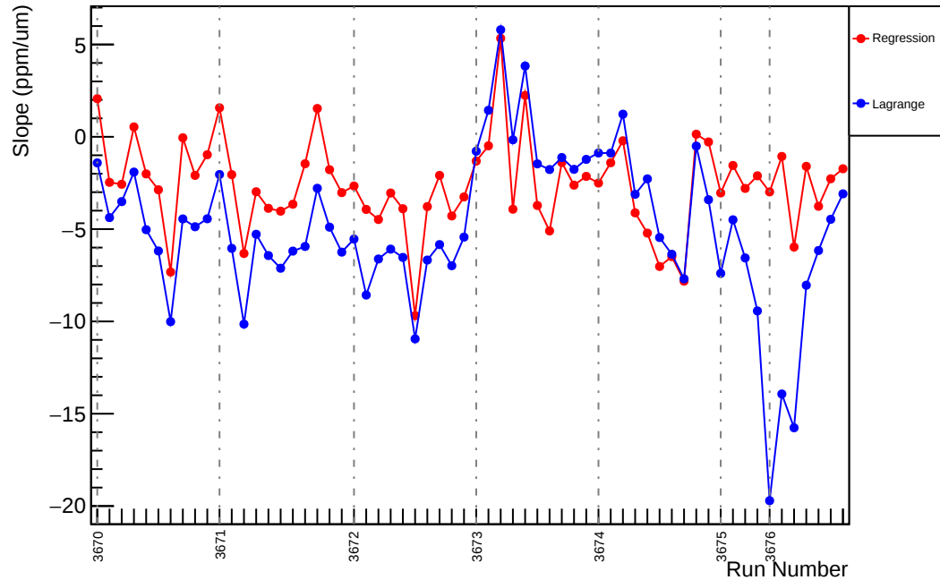
Slug15: Slope : us_avg_vs_evMon7 (ppm/um)
