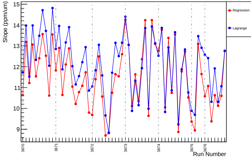
Slug15: Slope : us_avg_vs_evMon6 (ppm/um)
