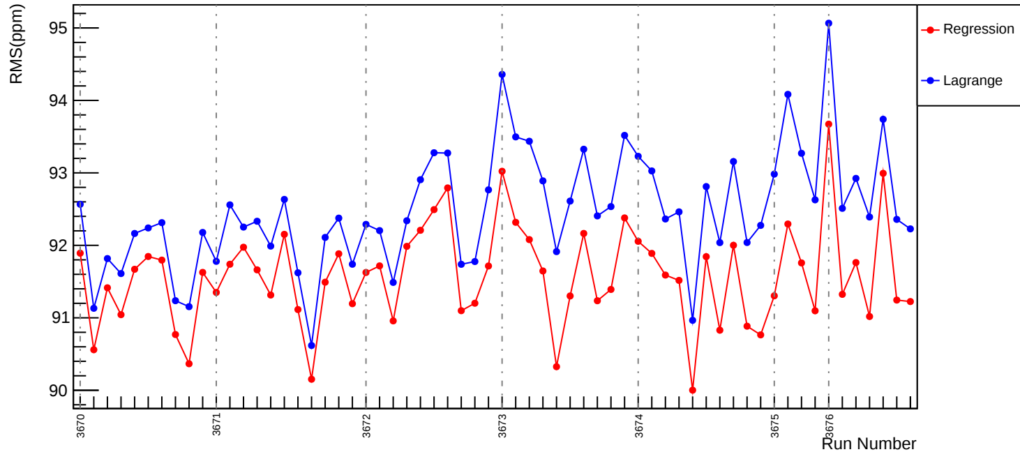
Slug15: Corrected RMS (ppm): asym_us_dd
