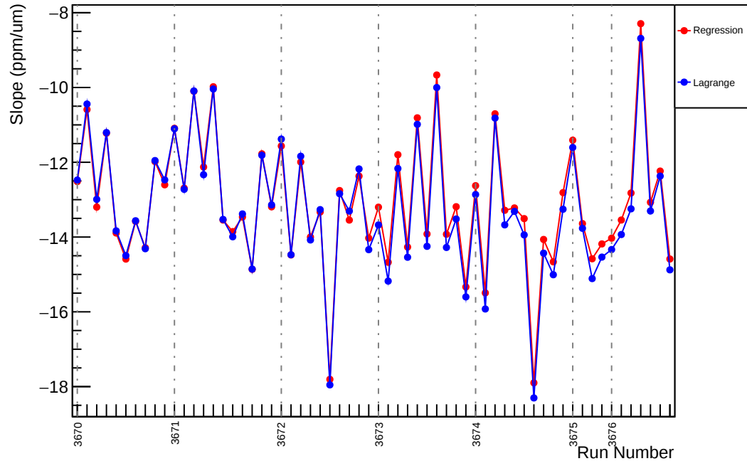
Slug15: Slope : us_dd_vs_evMon1 (ppm/um)
