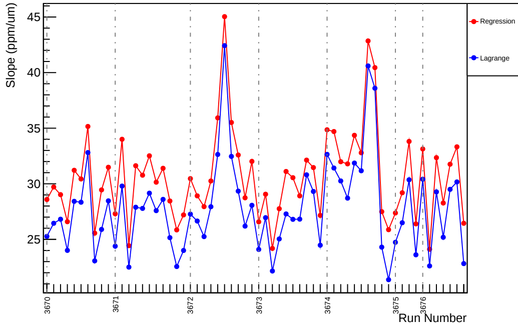
Slug15: Slope : us_dd_vs_evMon5 (ppm/um)
