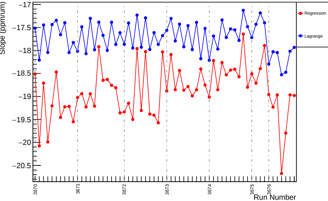
Slug15: Slope : us_dd_vs_evMon3 (ppm/um)
