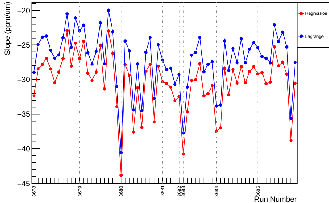
Slug16: Slope : us_dd_vs_evMon5 (ppm/um)
