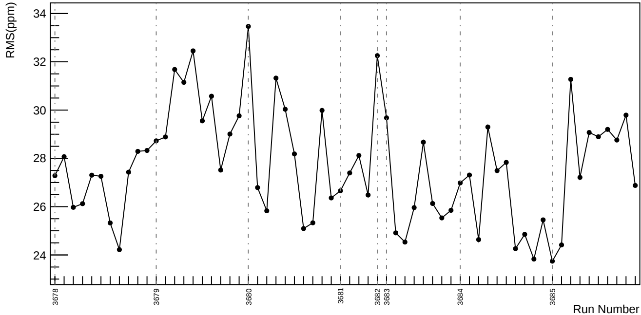
Slug16: asym_usr: \sqrt{\sigma_{\text{dit}}^2 - \sigma_{\text{reg}}^2} (ppm)
