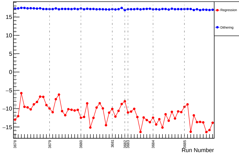
Slug16: Slope : usr_vs_evMon4 (ppm/um)
