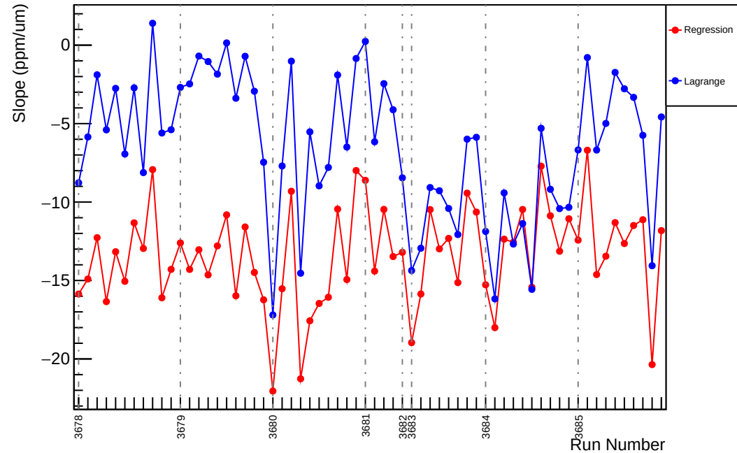
Slug16: Slope : usr_vs_evMon7 (ppm/um)
