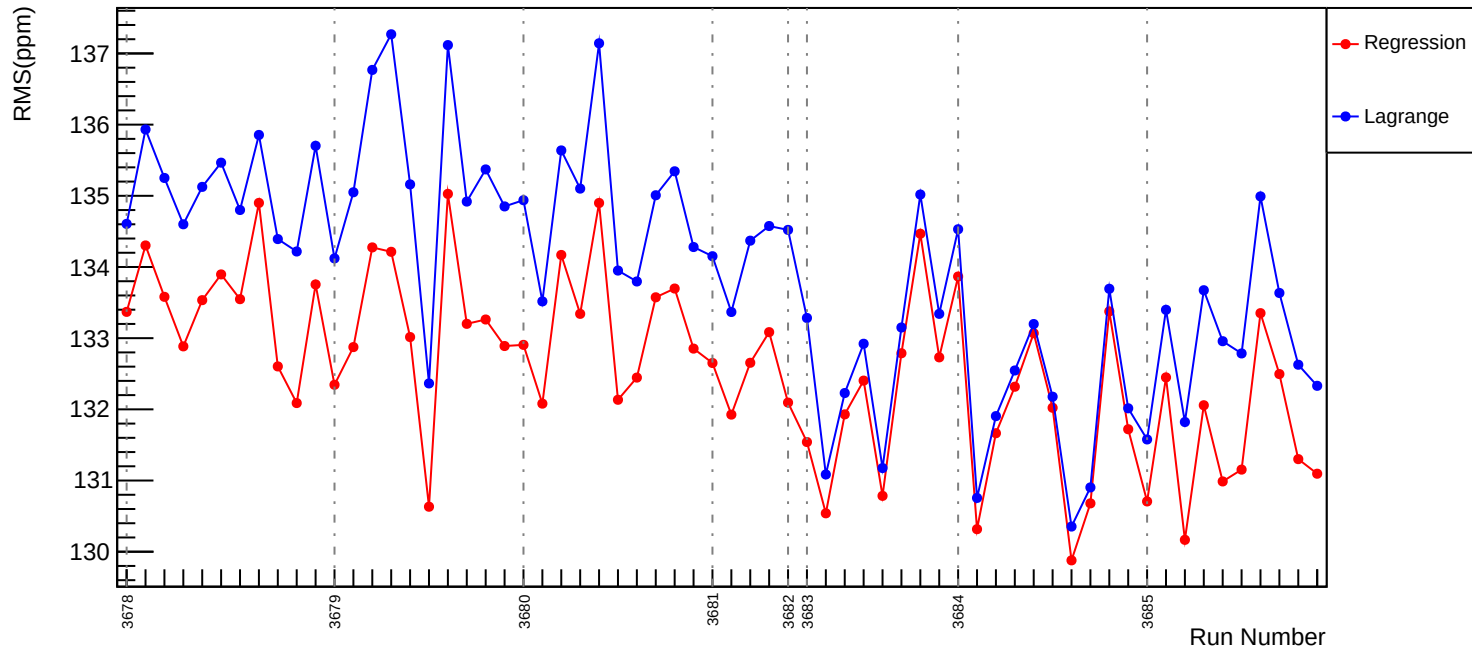
Slug16: Corrected RMS (ppm): asym_usr
