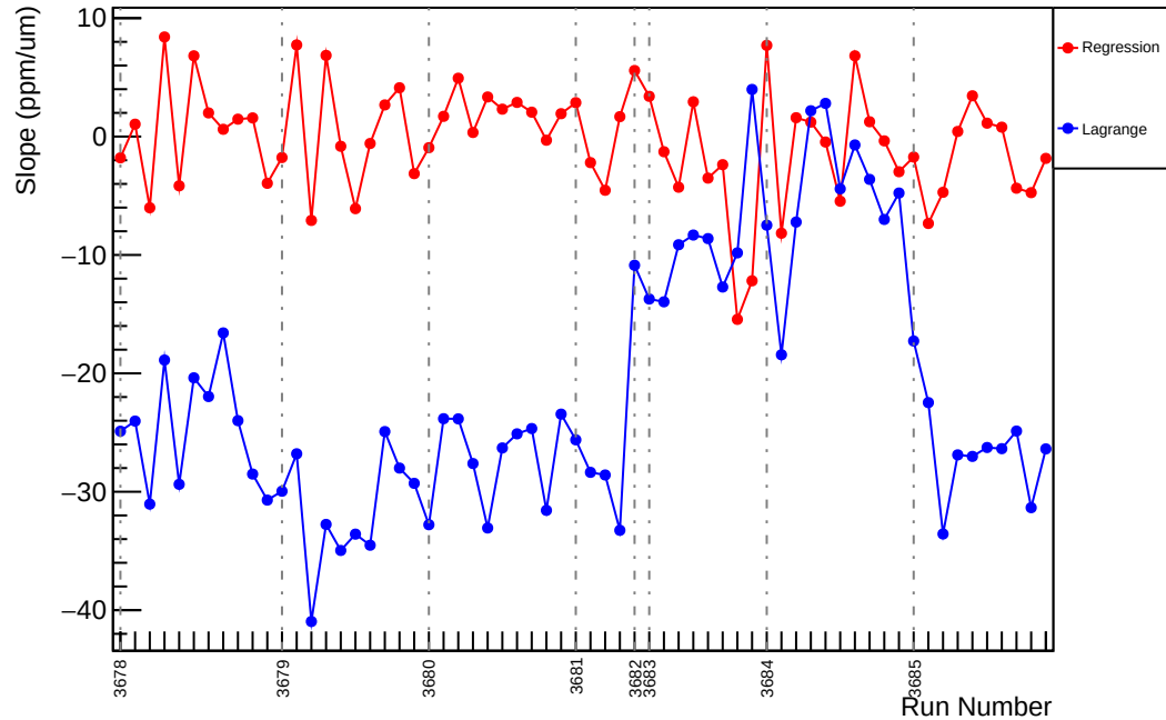
Slug16: Slope : usr_vs_evMon10 (ppm/um)
