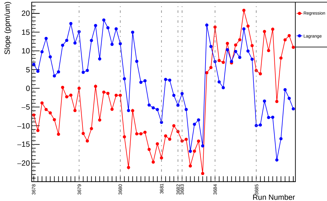
Slug16: Slope : usr_vs_evMon11 (ppm/um)
