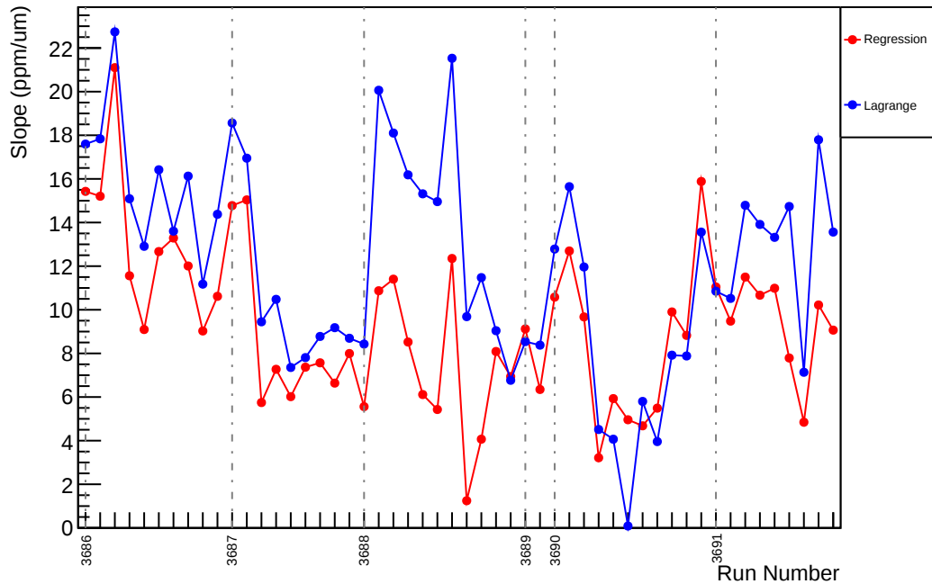
Slug17: Slope : us_avg_vs_evMon11 (ppm/um)
