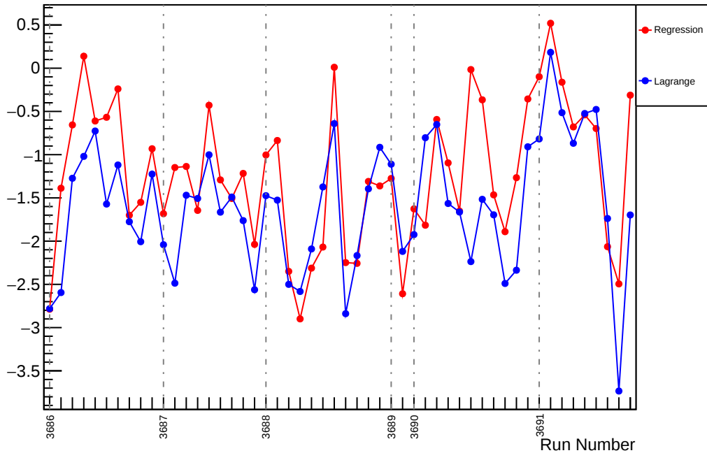
Slug17: Slope : us_avg_vs_evMon5 (ppm/um)
