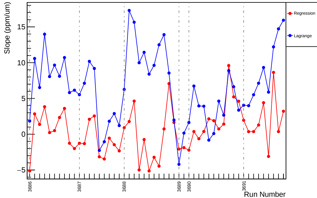
Slug17: Slope : us_avg_vs_evMon10 (ppm/um)
