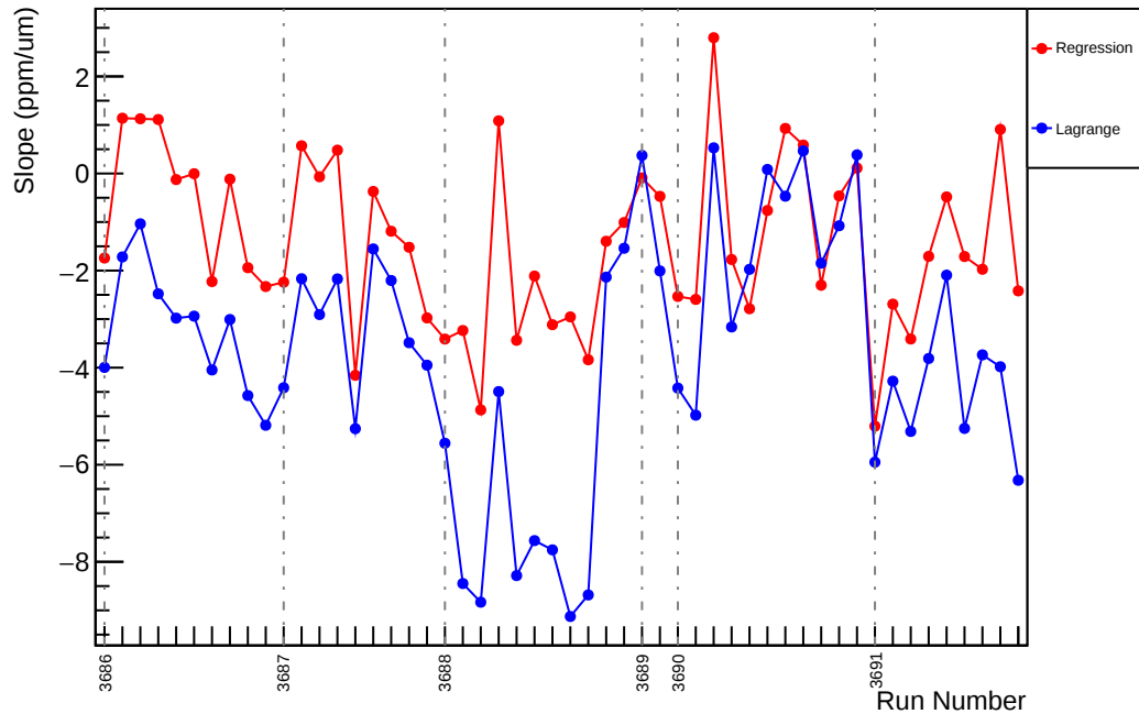
Slug17: Slope : us_avg_vs_evMon7 (ppm/um)
