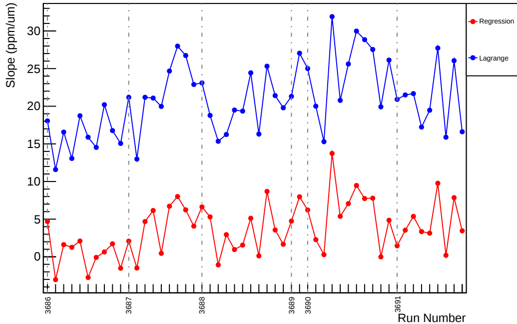
Slug17: Slope : us_dd_vs_evMon11 (ppm/um)
