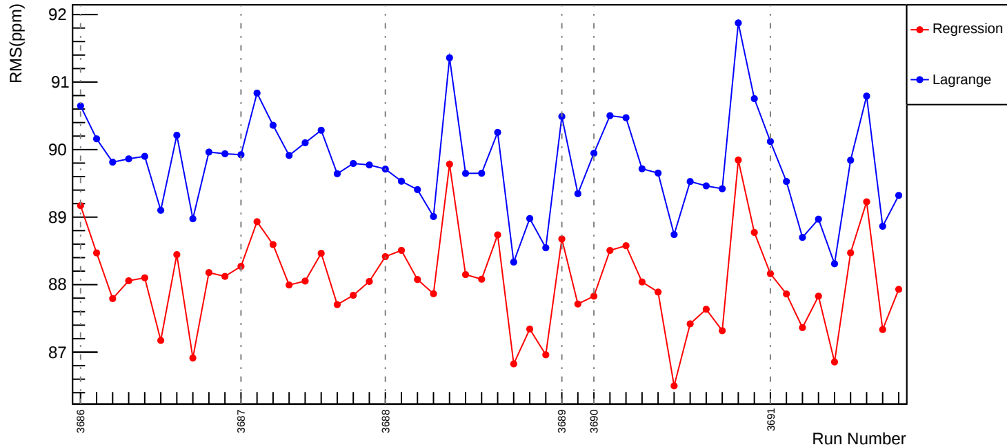
Slug17: Corrected RMS (ppm): asym_us_dd
