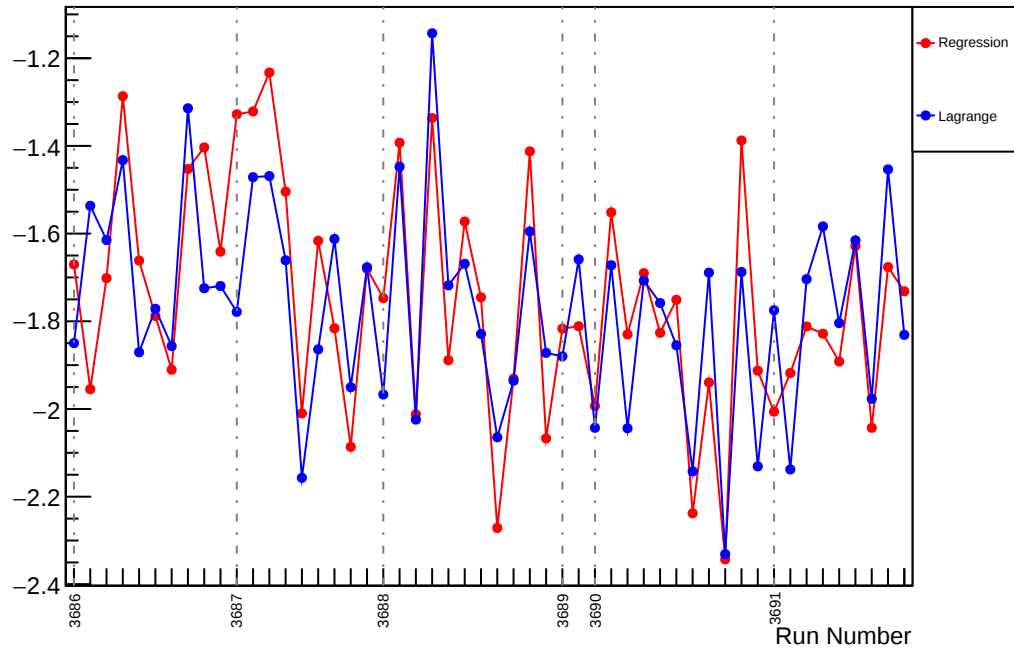
Slug17: Slope : us_dd_vs_evMon2 (ppm/um)
