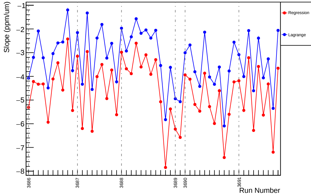
Slug17: Slope : us_dd_vs_evMon6 (ppm/um)
