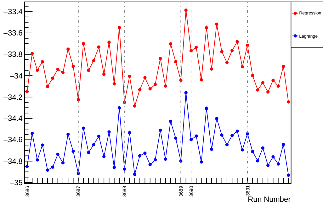
Slug17: Slope : us_dd_vs_evMon0 (ppm/um)
