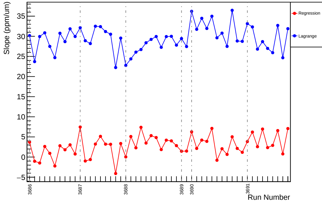
Slug17: Slope : us_dd_vs_evMon10 (ppm/um)
