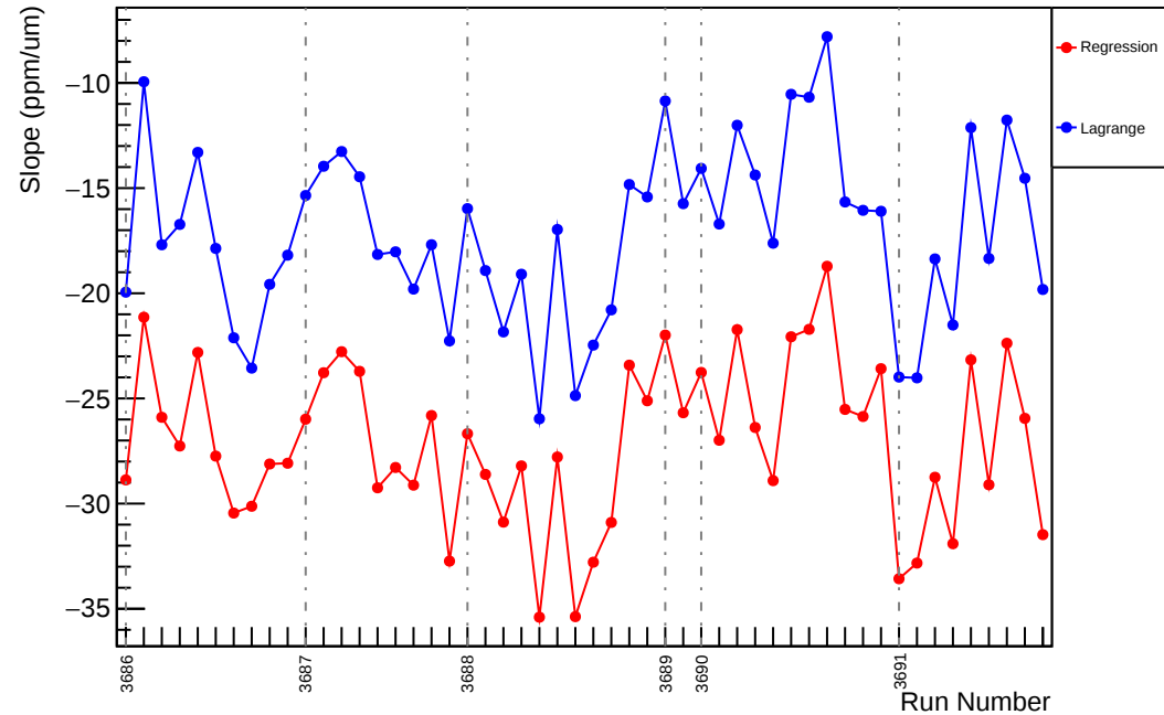
Slug17: Slope : usr_vs_evMon5 (ppm/um)
