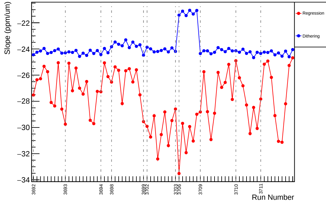
Slug18: Slope : us_dd_vs_evMon3 (ppm/um)
