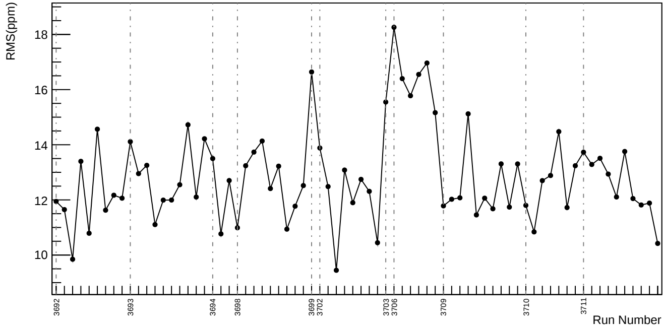
Slug18: asym_us_dd: \sqrt{\sigma_{\text{dit}}^2 - \sigma_{\text{reg}}^2} (ppm)
