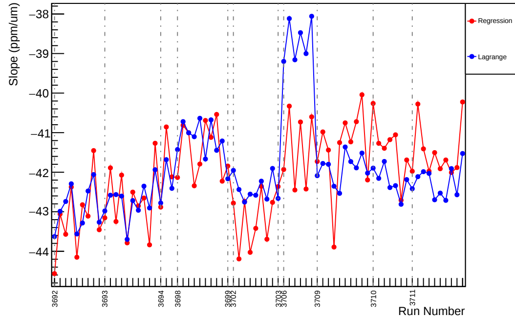
Slug18: Slope : usl_vs_evMon3 (ppm/um)
