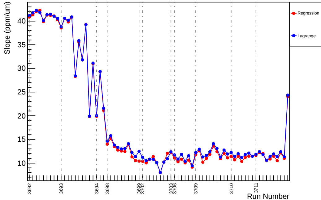
Slug18: Slope : usl_vs_evMon2 (ppm/um)
