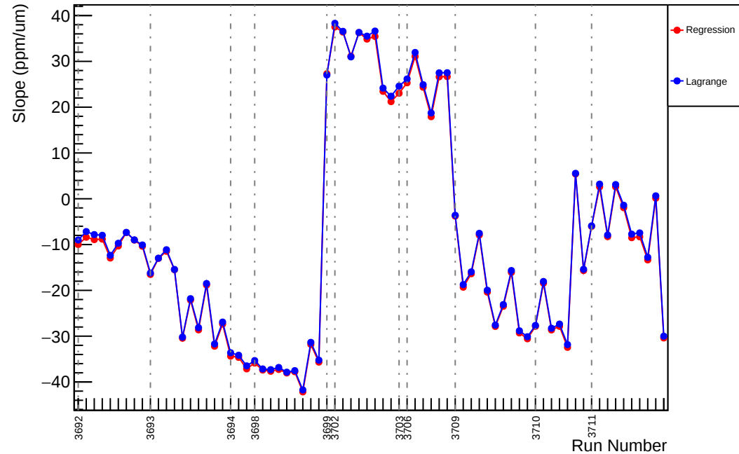
Slug18: Slope : usl_vs_evMon1 (ppm/um)
