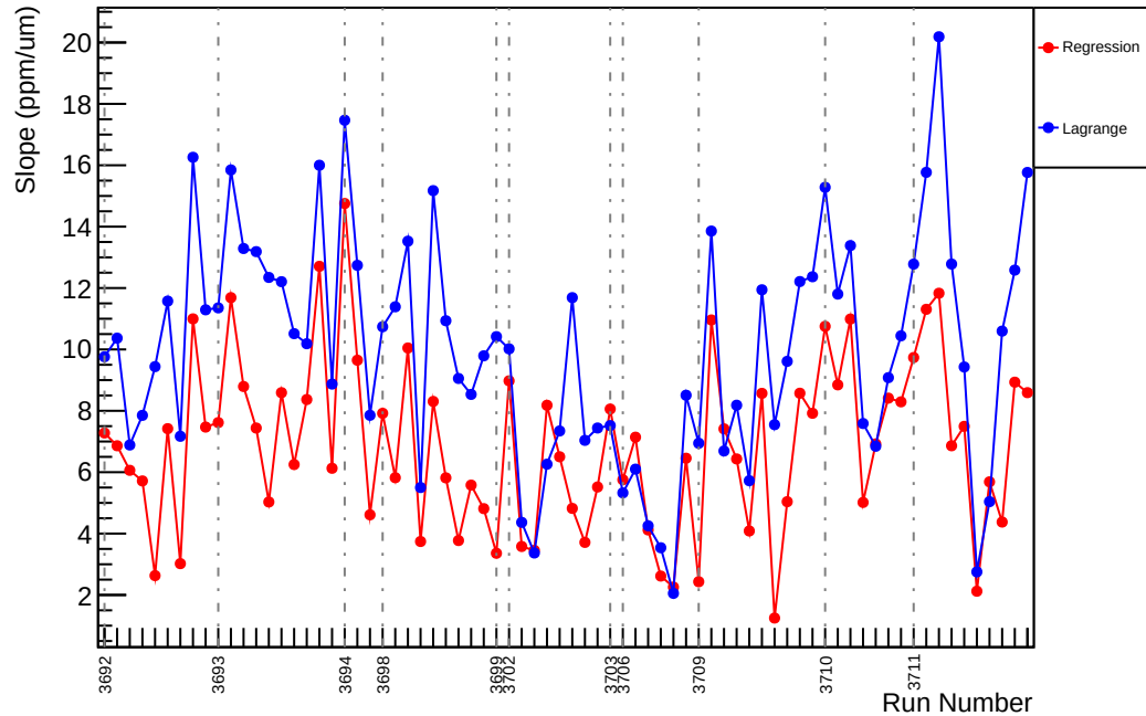
Slug18: Slope : usl_vs_evMon8 (ppm/um)
