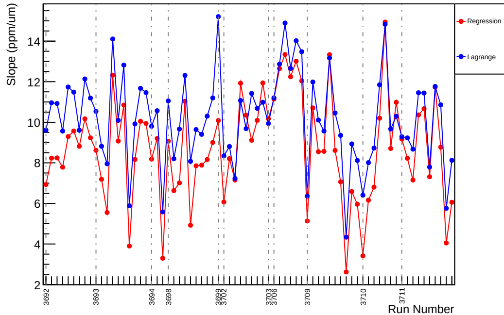
Slug18: Slope : usl_vs_evMon6 (ppm/um)
