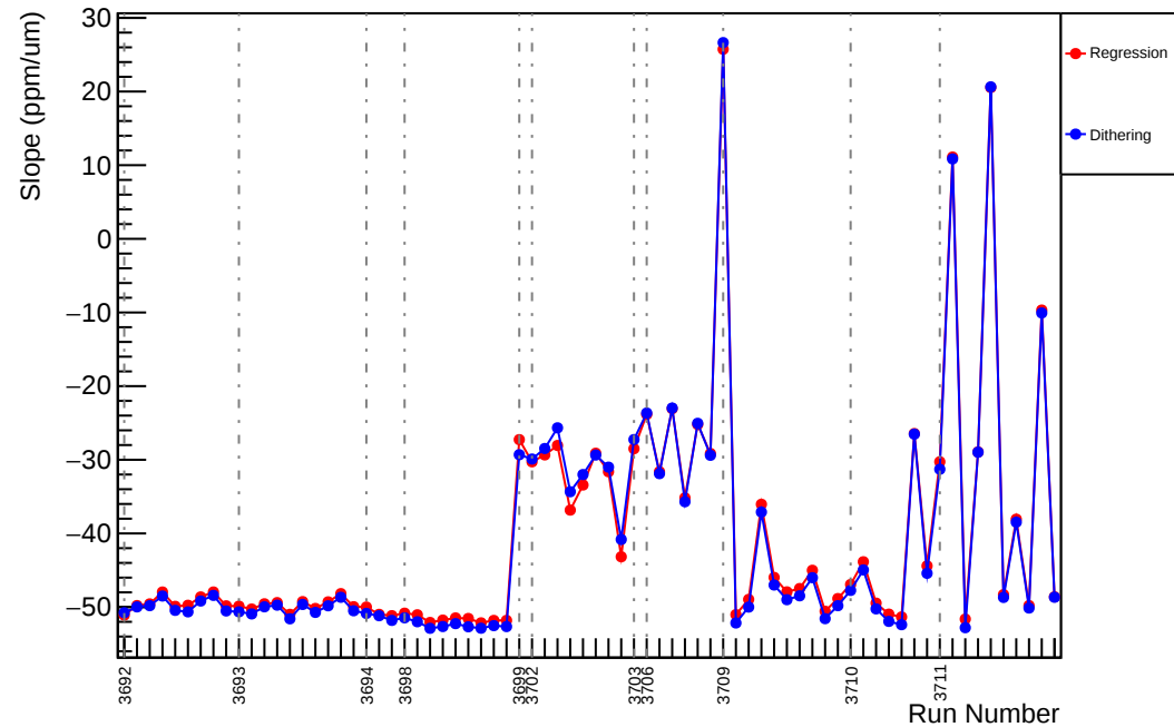
Slug18: Slope : usr_vs_evMon0 (ppm/um)
