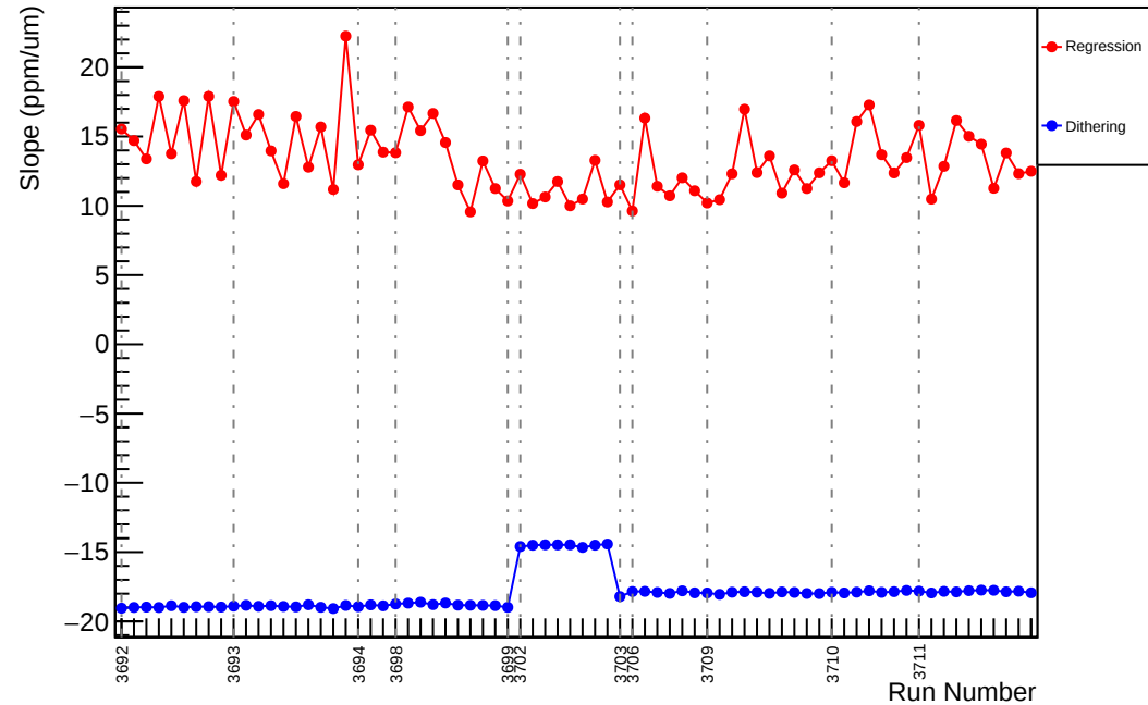
Slug18: Slope : usr_vs_evMon4 (ppm/um)
