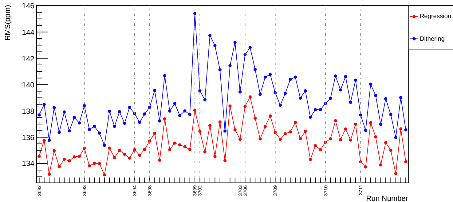
Slug18: Corrected RMS (ppm): asym_usr
