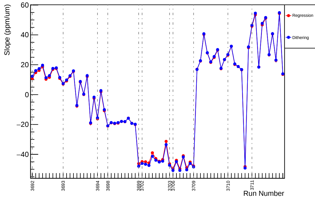
Slug18: Slope : usr_vs_evMon1 (ppm/um)
