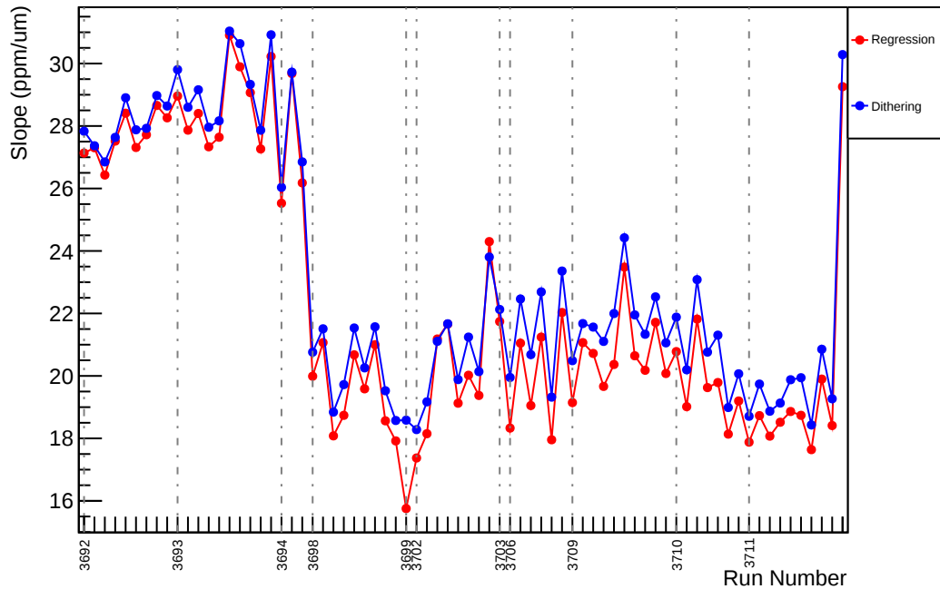
Slug18: Slope : usr_vs_evMon2 (ppm/um)
