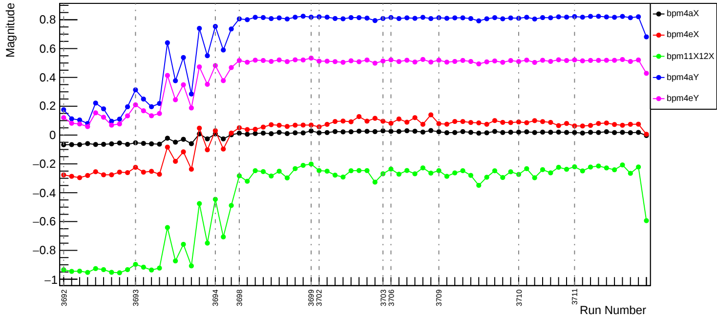
Slug18: EigenVector #2
