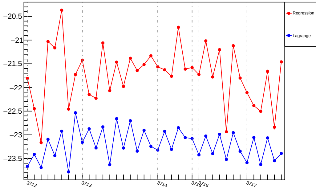
Slug19: Slope : us_avg_vs_evMon3 (ppm/um)
