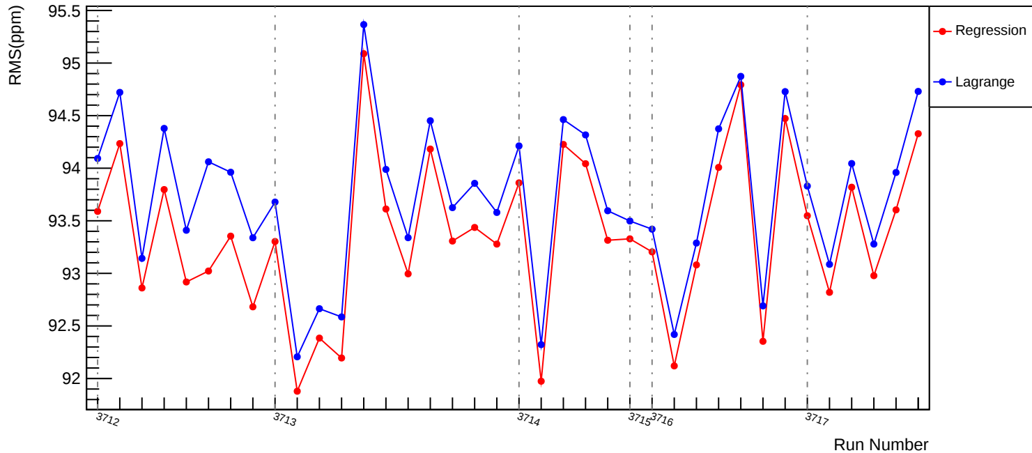
Slug19: Corrected RMS (ppm): asym_us_avg
