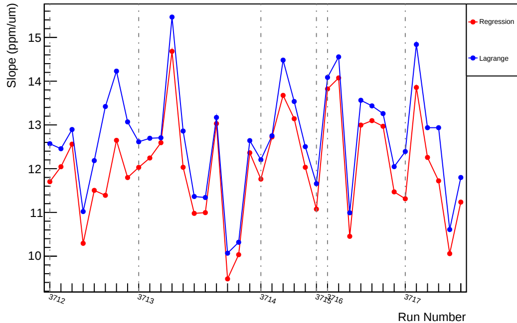
Slug19: Slope : us_avg_vs_evMon6 (ppm/um)
