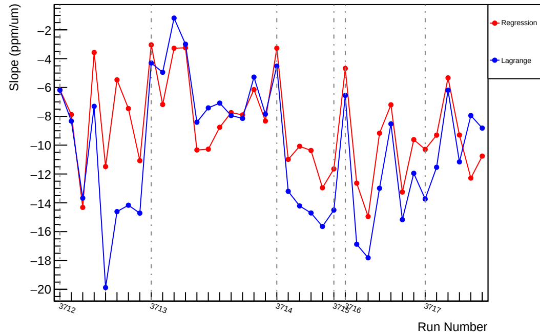
Slug19: Slope : us_avg_vs_evMon11 (ppm/um)
