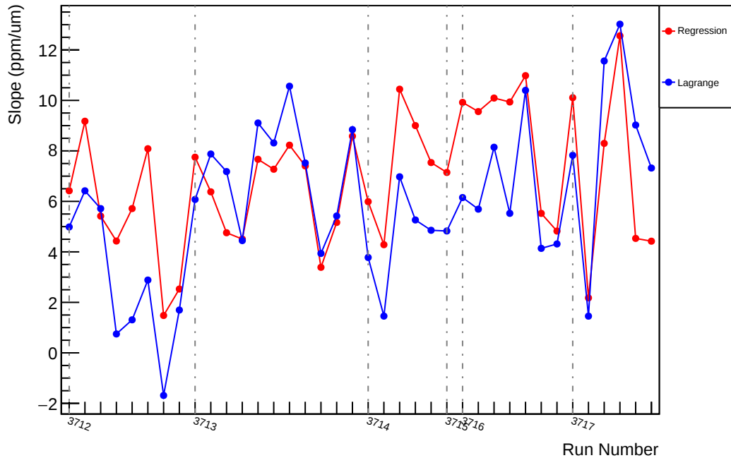
Slug19: Slope : us_avg_vs_evMon9 (ppm/um)
