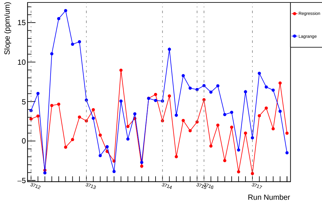
Slug19: Slope : us_avg_vs_evMon10 (ppm/um)
