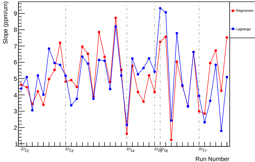
Slug19: Slope : us_avg_vs_evMon8 (ppm/um)
