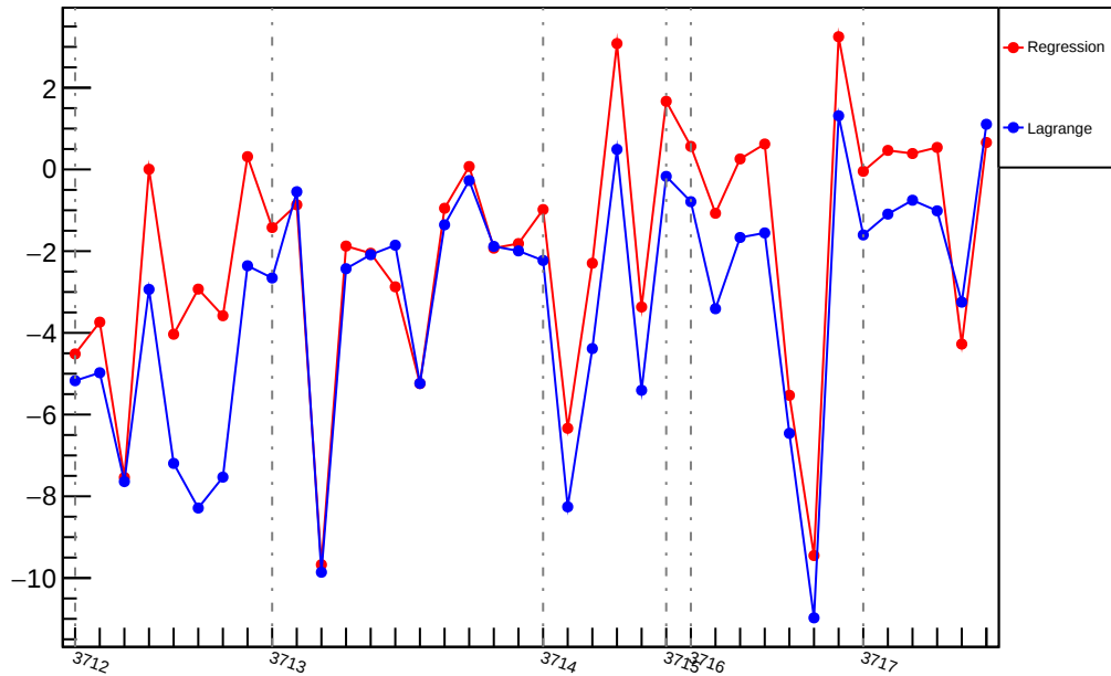
Slug19: Slope : us_avg_vs_evMon7 (ppm/um)
