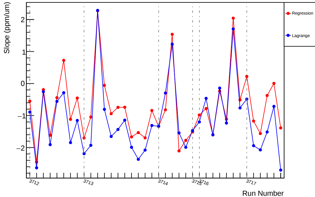
Slug19: Slope : us_avg_vs_evMon5 (ppm/um)
