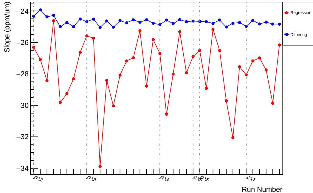
Slug19: Slope : us_dd_vs_evMon3 (ppm/um)
