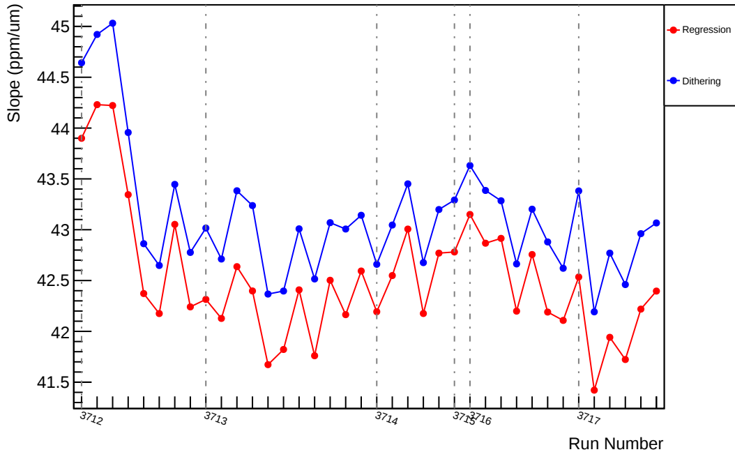
Slug19: Slope : us_dd_vs_evMon0 (ppm/um)
