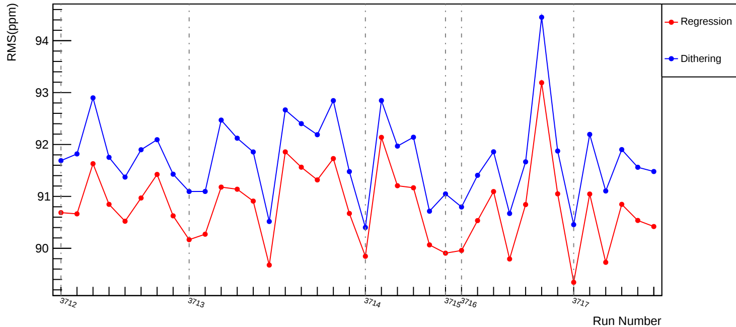
Slug19: Corrected RMS (ppm): asym_us_dd
