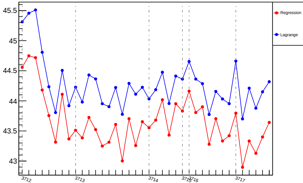
Slug19: Slope : us_dd_vs_evMon0 (ppm/um)
