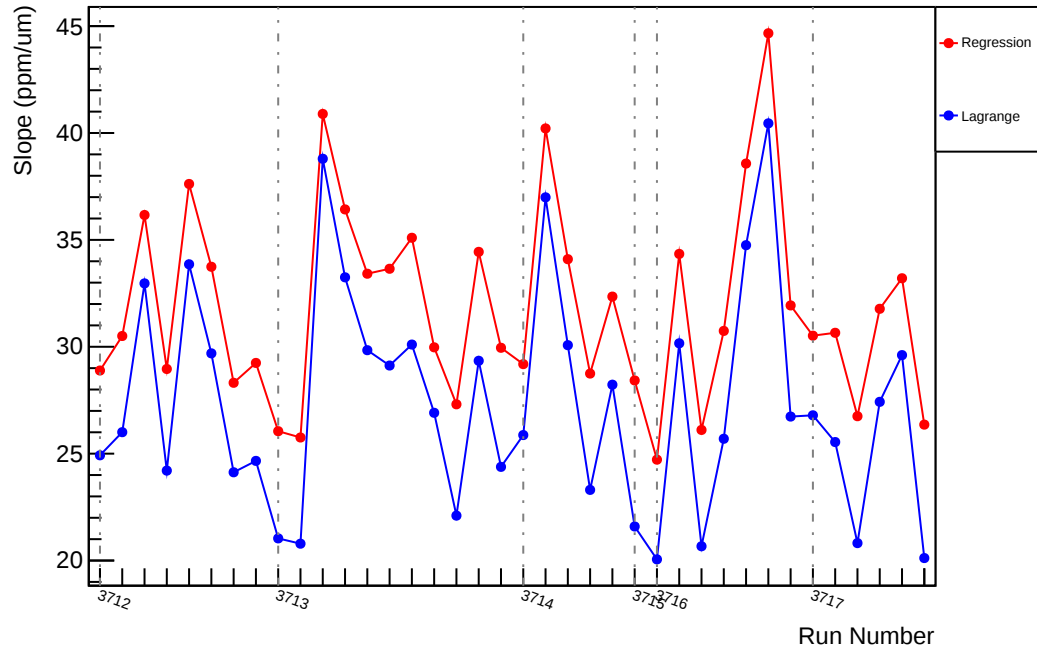
Slug19: Slope : us_dd_vs_evMon5 (ppm/um)
