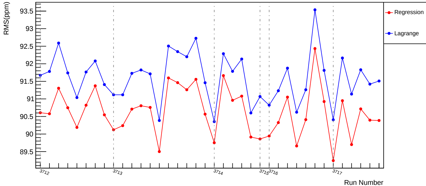
Slug19: Corrected RMS (ppm): asym_us_dd
