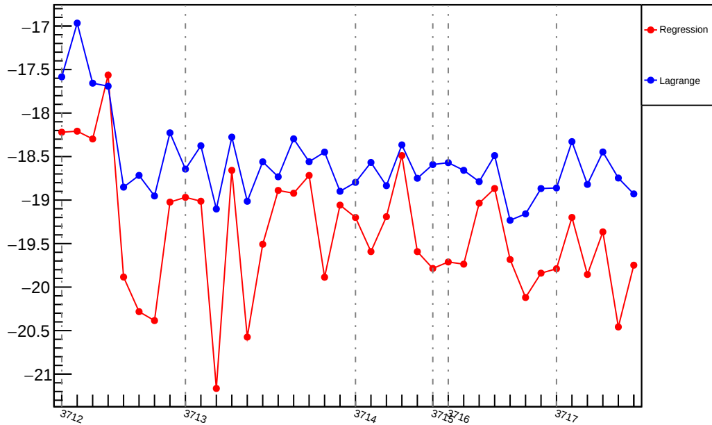
Slug19: Slope : us_dd_vs_evMon3 (ppm/um)
